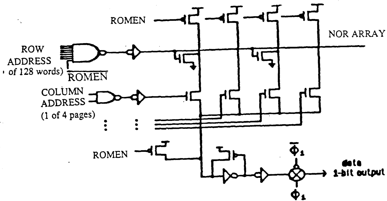
Figure 13. Circuit Diagram of ROM
