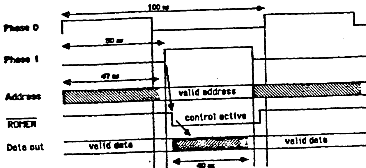
Figure 14. Timing Diagram of ROM
