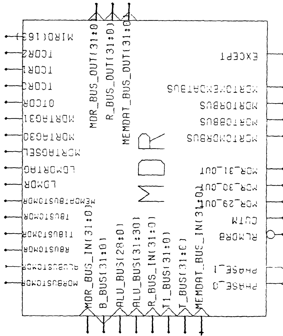
Figure 9. MDR Block's Symbol
