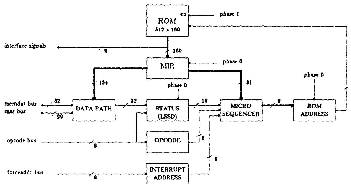
FIGURE 4 BLOCK DIAGRAM OF VLSI-PLM
