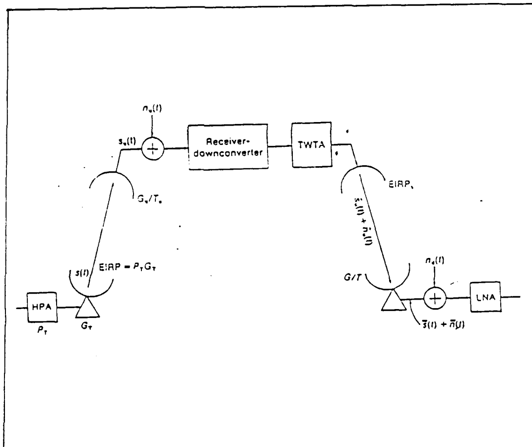
Figure 1.6 Basic link analysis
