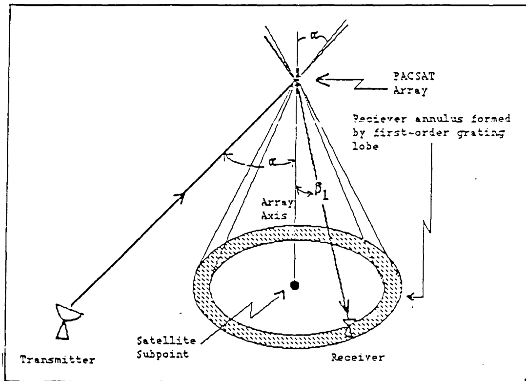
Figure 6.1 PACSAT link configuration
