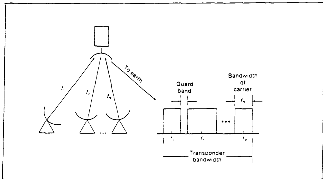
Figure 1.7 FDMA frame structure
