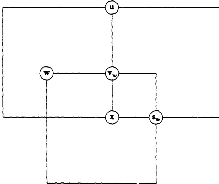
Figure 4.3. Processor w in SW(u, \alpha^i)
