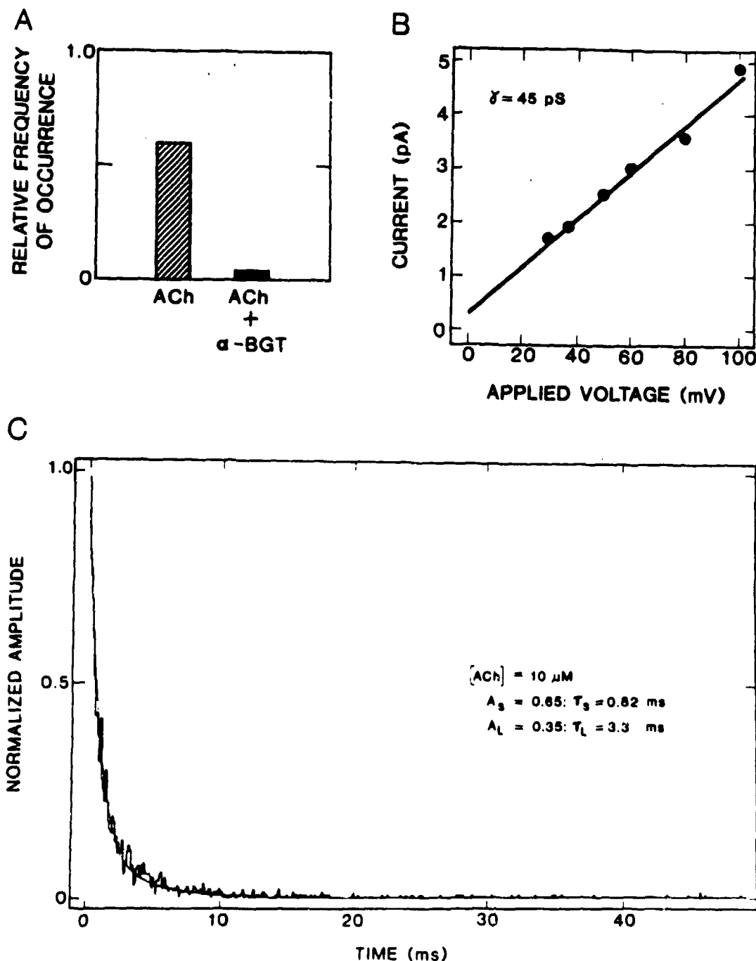
Figure 6. Analysis of single acetylcholine receptor currents in TE671 cells. A , \alpha -bungarotoxin (0.04-0.15 \mu M in various experiments) blocks the opening of receptor channels induced by acetylcholine (at 0.5-50 \mu M). B , The receptor channels behave ohmically with a conductance of 45 pS. C , Receptor channels frequently open for short durations (0.82 ms) and less frequently open for longer durations (3.3 ms) in 10 \mu M acetylcholine at 100 mv. The data for 2,035 openings (noisy curve) are fit by a sum of two exponentials (smooth curve). Reproduced from reference 23.
