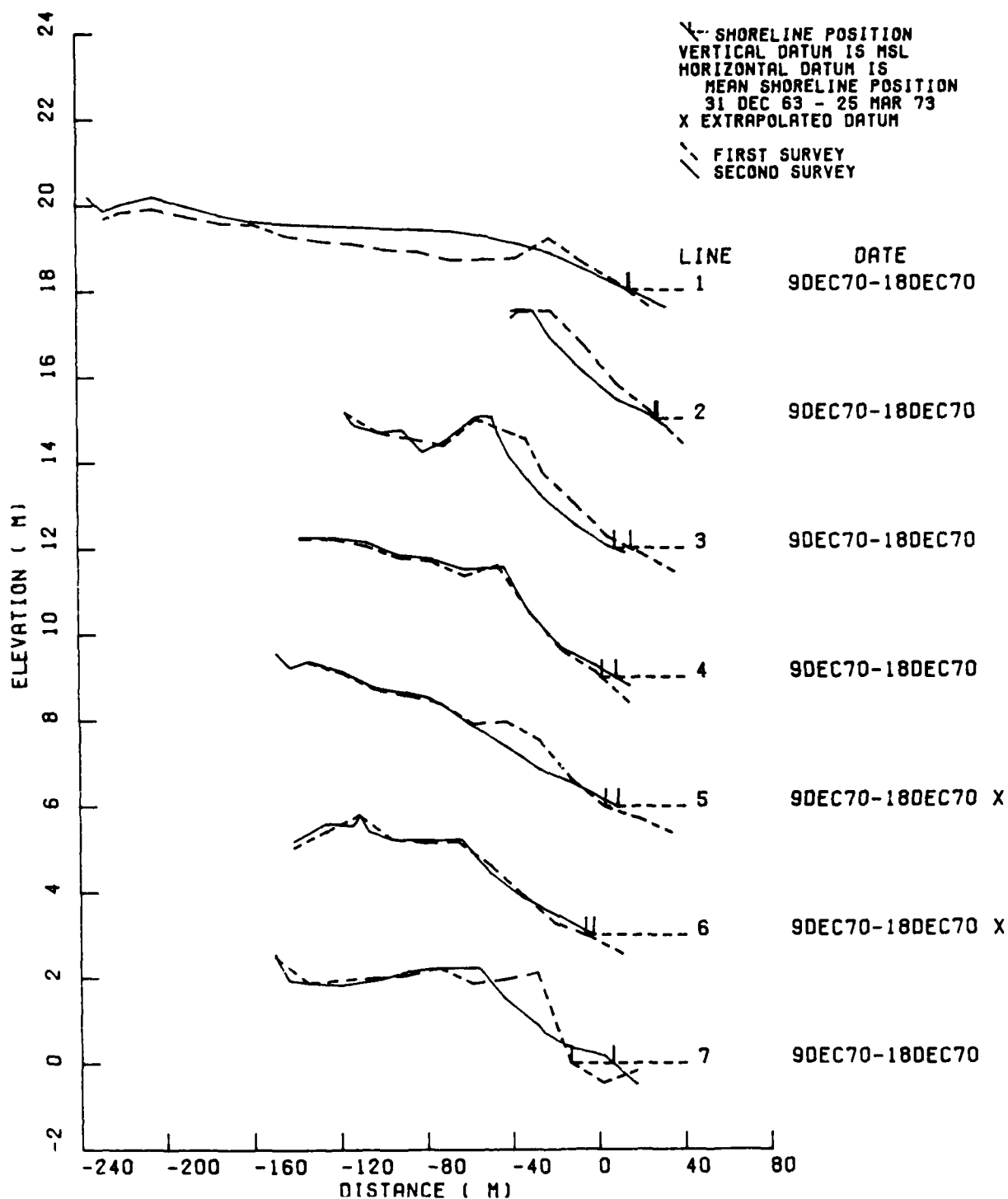
Figure H19. Profile comparisons for surveys at Atlantic City, N. J.
