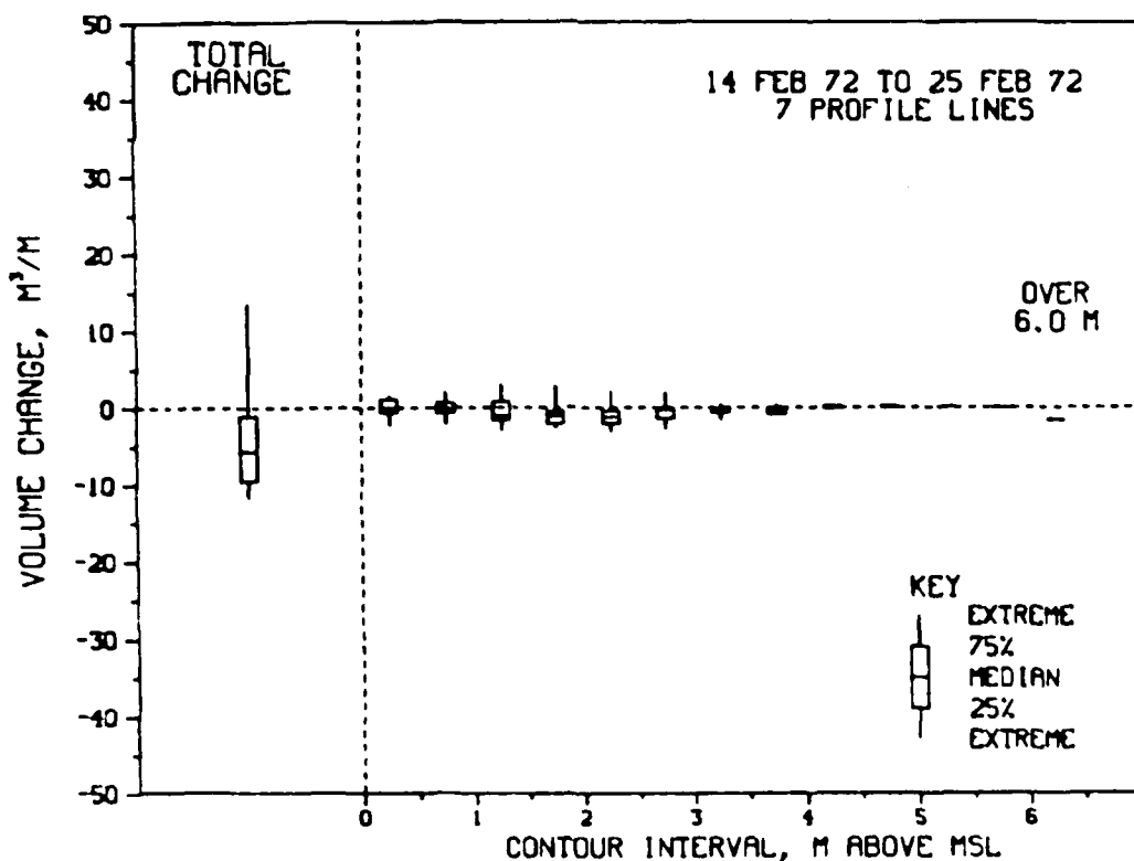
Figure 18. Distribution of volume changes by contour for Misquamicut, R. I.
