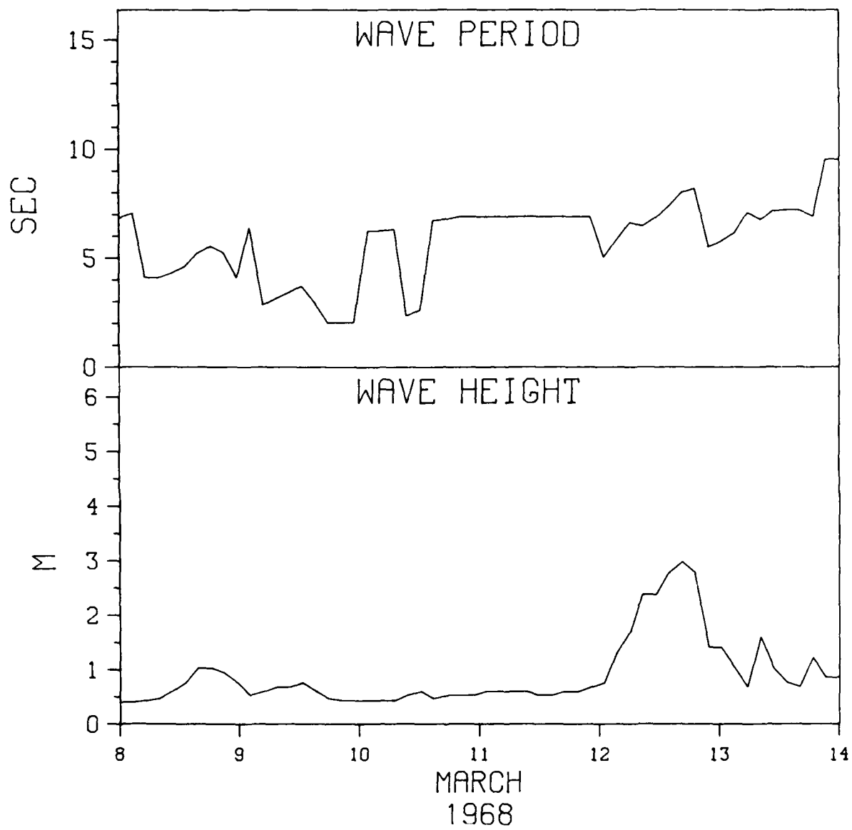
Figure E3. Hindcasted wave data for Misquamicut, R. I.
