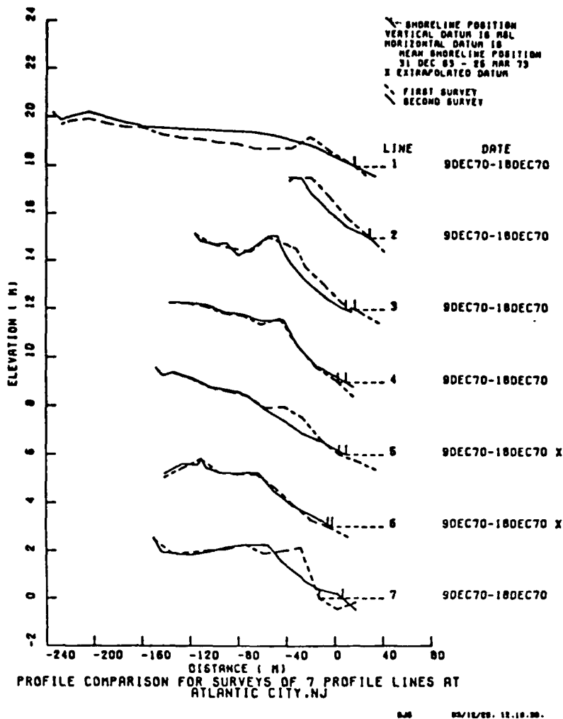
Figure 2. Example cross-section plot
