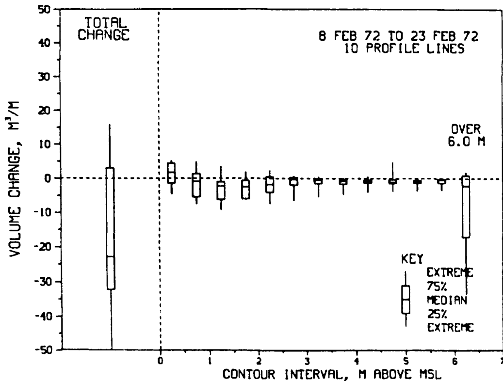
Figure I5. Distribution of volume changes by contour for Nauset Beach, Mass.
