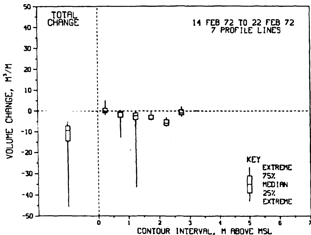
Figure I20. Distribution of volume changes by contour for Atlantic City, N. J.
