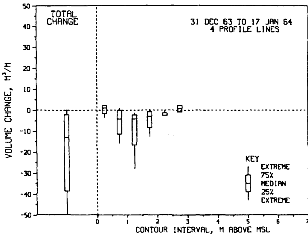
Figure C7. Distribution of volume changes by contour for Atlantic City, N. J.
