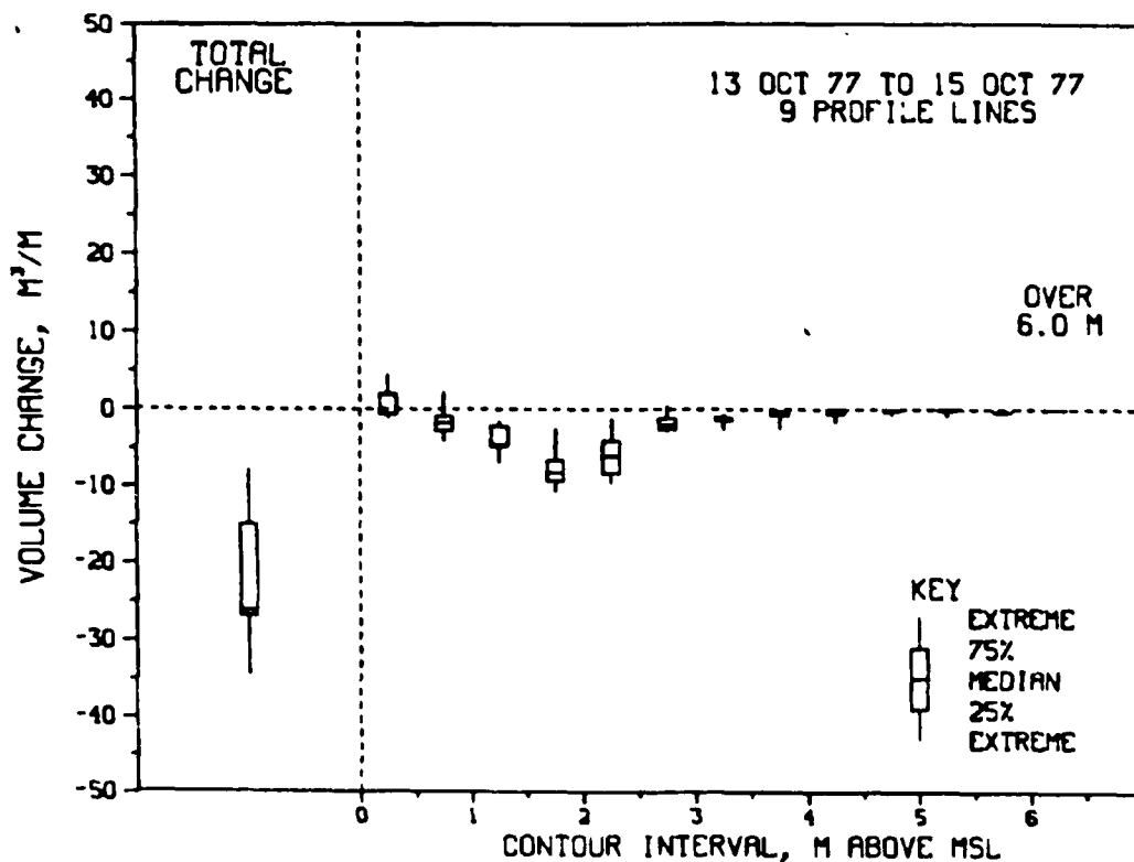
Figure K4. Distribution of volume changes by contour for Long Beach Island, N. J.
