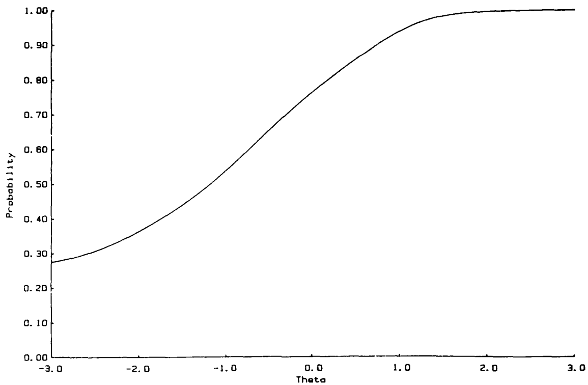
Figure B-127. Test Characteristic Curve for Word Knowledge Subtest on ASVAB Form 11a (Female Sample).
