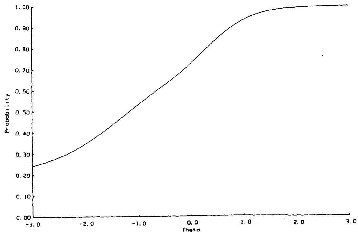
Figure B-80. Test Characteristic Curve for Paragraph Comprehension Subtest on ASVAB Form 12a (Male Sample).
