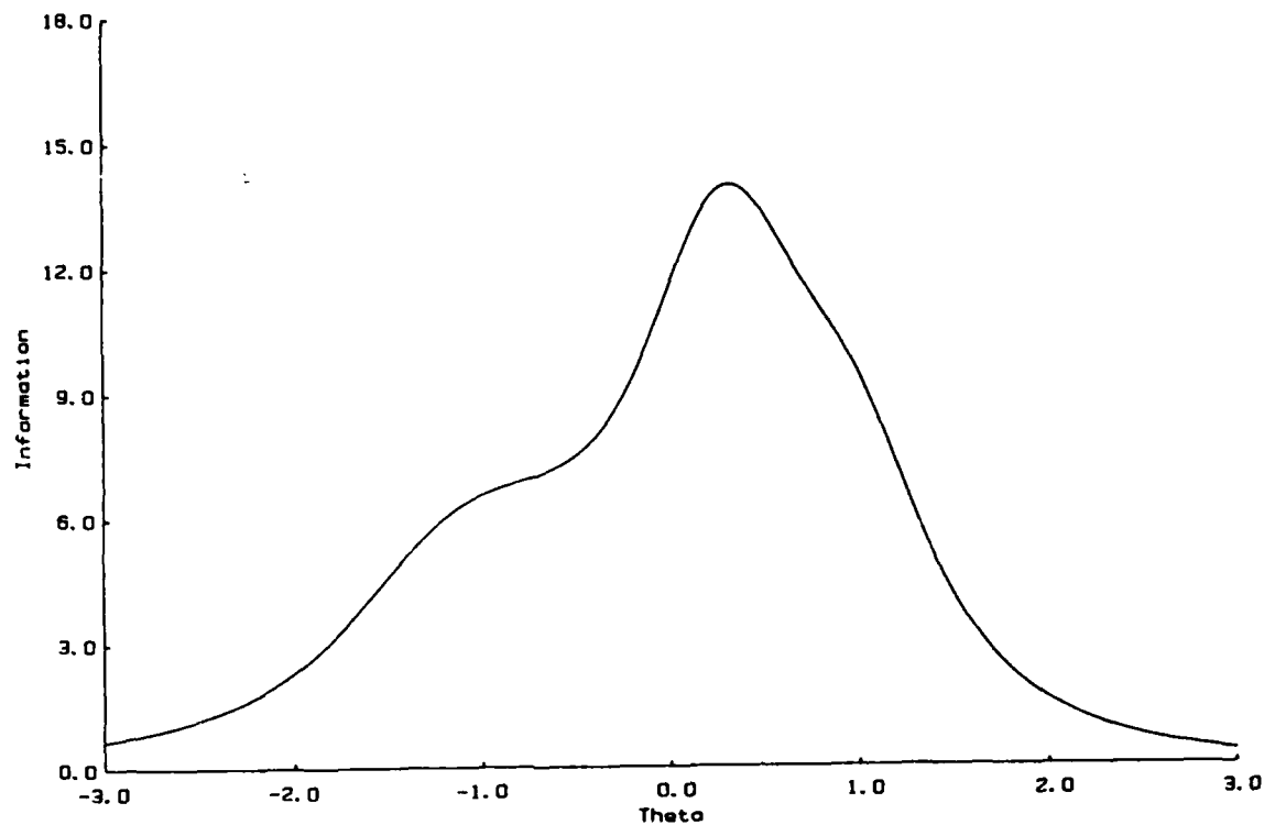
Figure A-29. Test Information Curve for Auto and Shop Information Subtest on ASVAB Form 11a (Total Sample).
