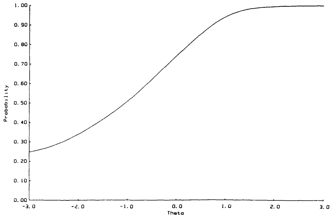
Figure 8-15. Test Characteristic Curve for Word Knowledge Subtest on ASVAB Form 11a (Total Sample).
