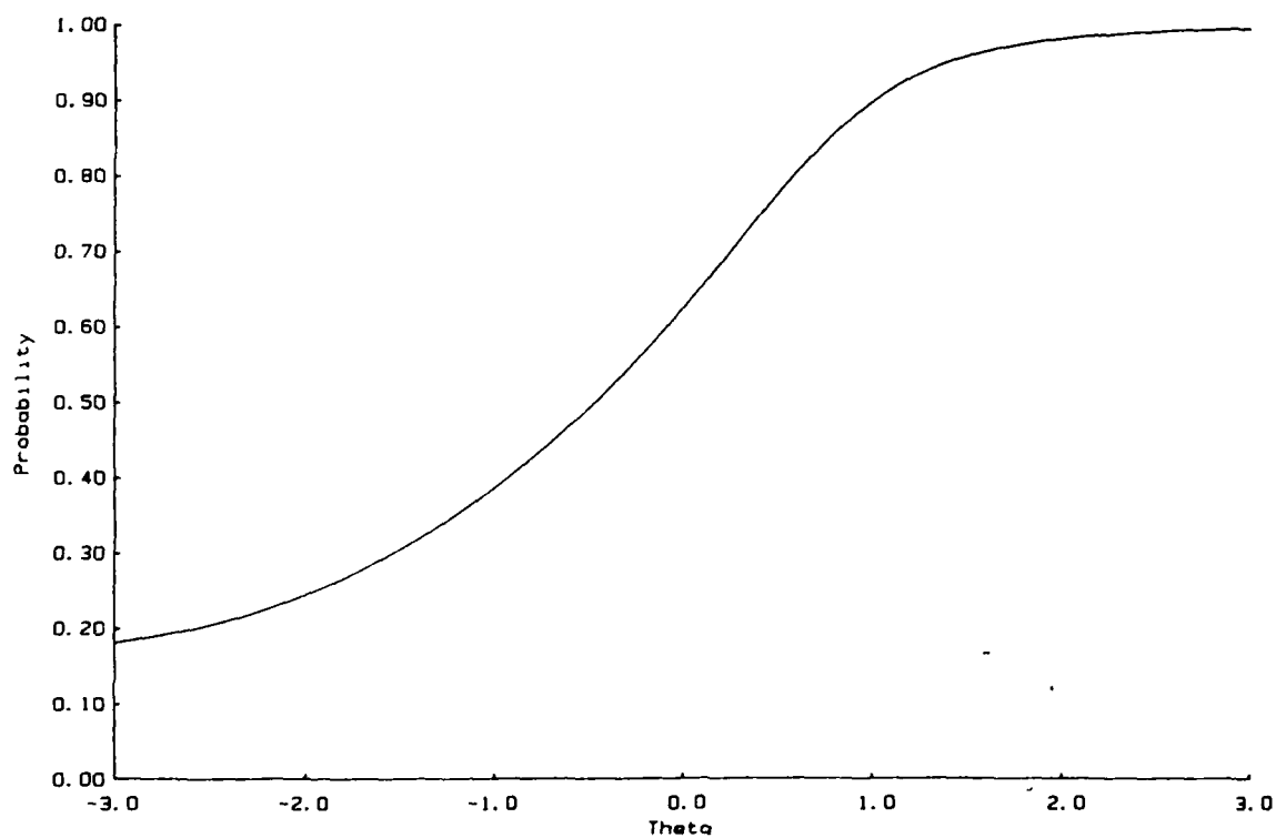
Figure B-64. Test Characteristic Curve for Arithmetic Reasoning Subtest on ASVAB Form 11a (Male Sample).
