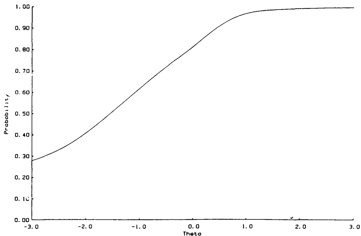
Figure B-81. Test Characteristic Curve for Paragraph Comprehension Subtest on ASVAB Form 12b (Male Sample).
