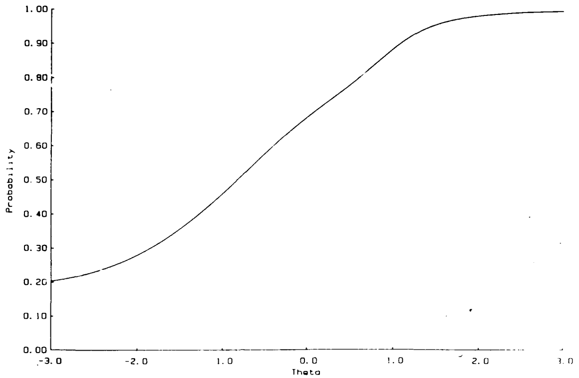
Figure 8-61. Test Characteristic Curve for General Science Subtest on ASVAB Form 13a (Male Sample).
