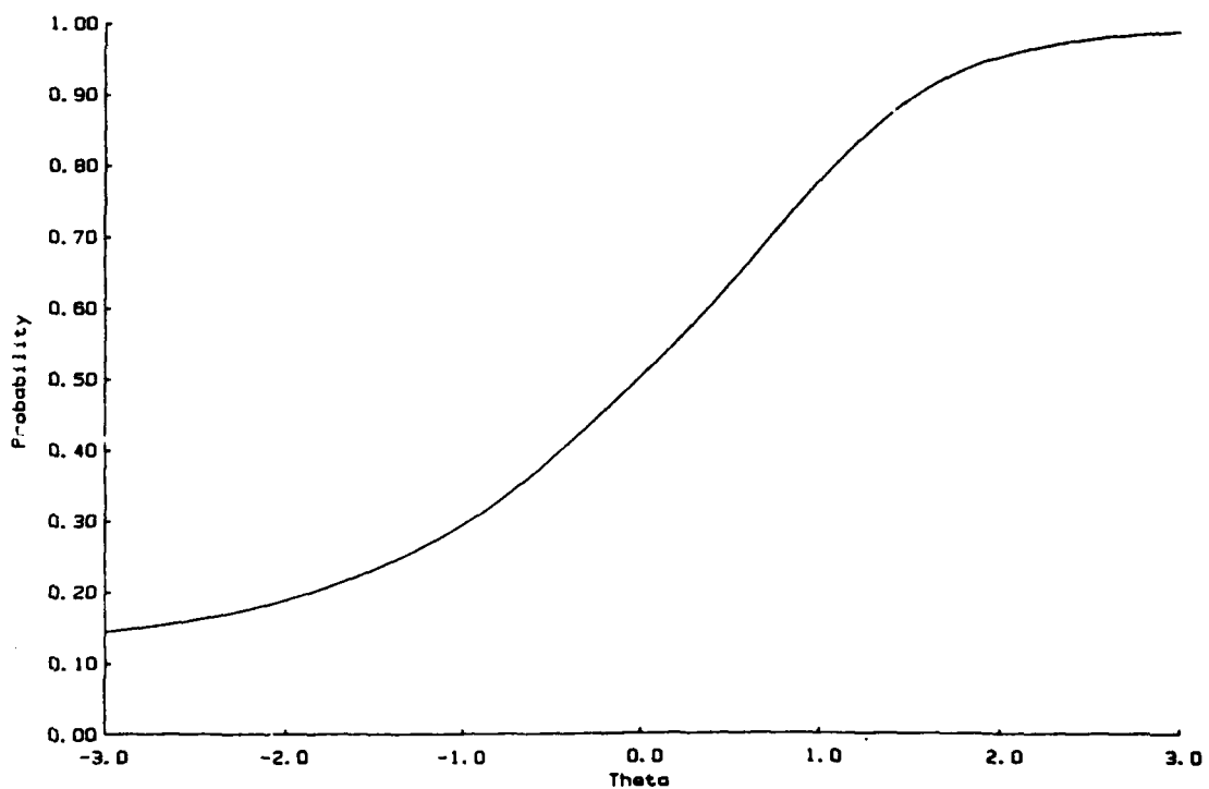
Figure B-40. Test Characteristic Curve for Mathematics Knowledge Subtest on ASVAB Form 13a (Total Sample).
