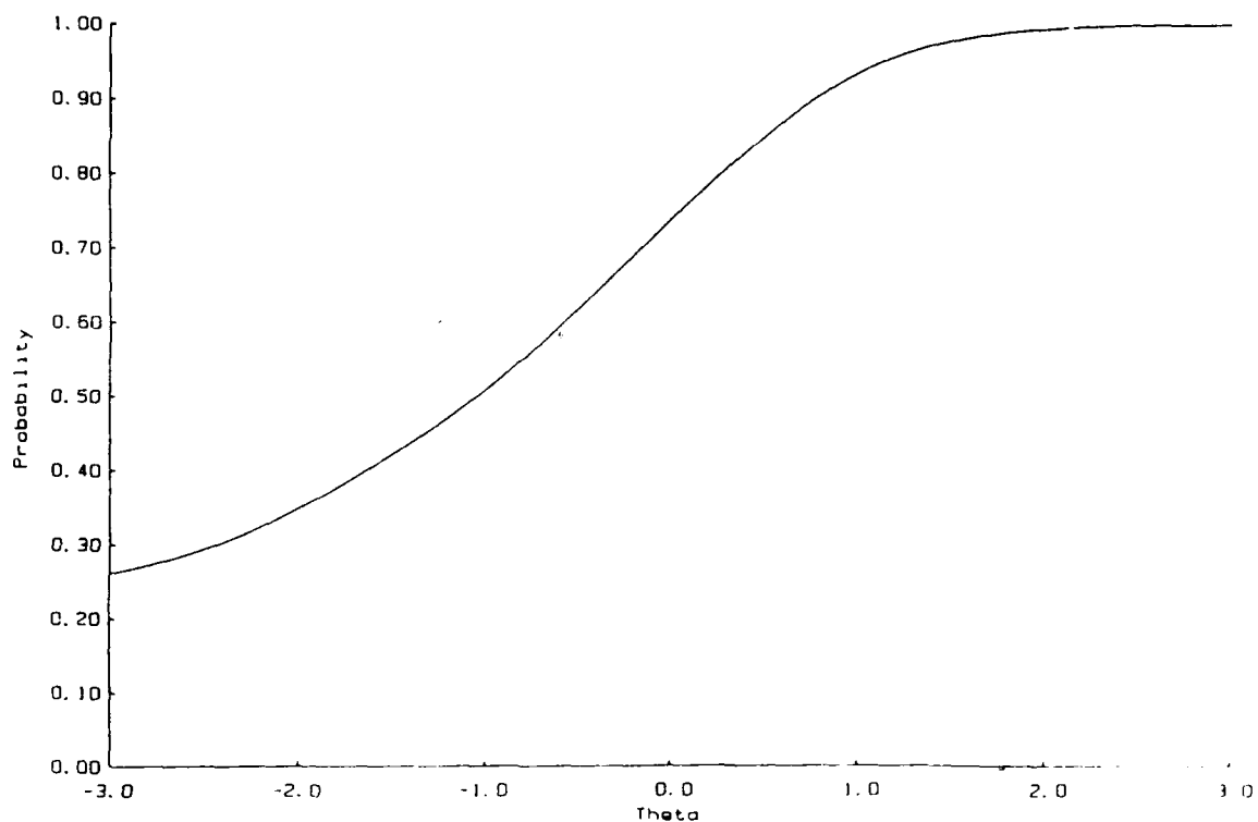
Figure B-75. Test Characteristic Curve for Word Knowledge Subtest on ASVAB Form 13a (Male Sample).
