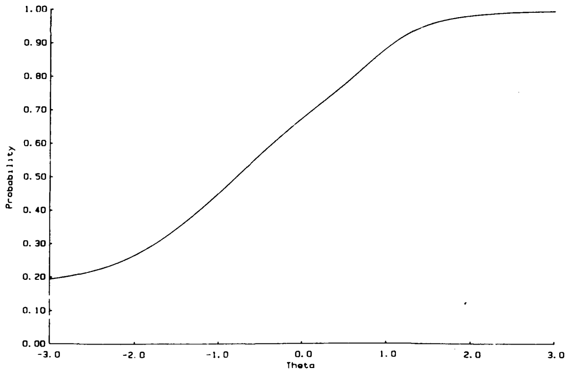
Figure 8-62. Test Characteristic Curve for General Science Subtest on ASVAB Form 13b (Male Sample).
