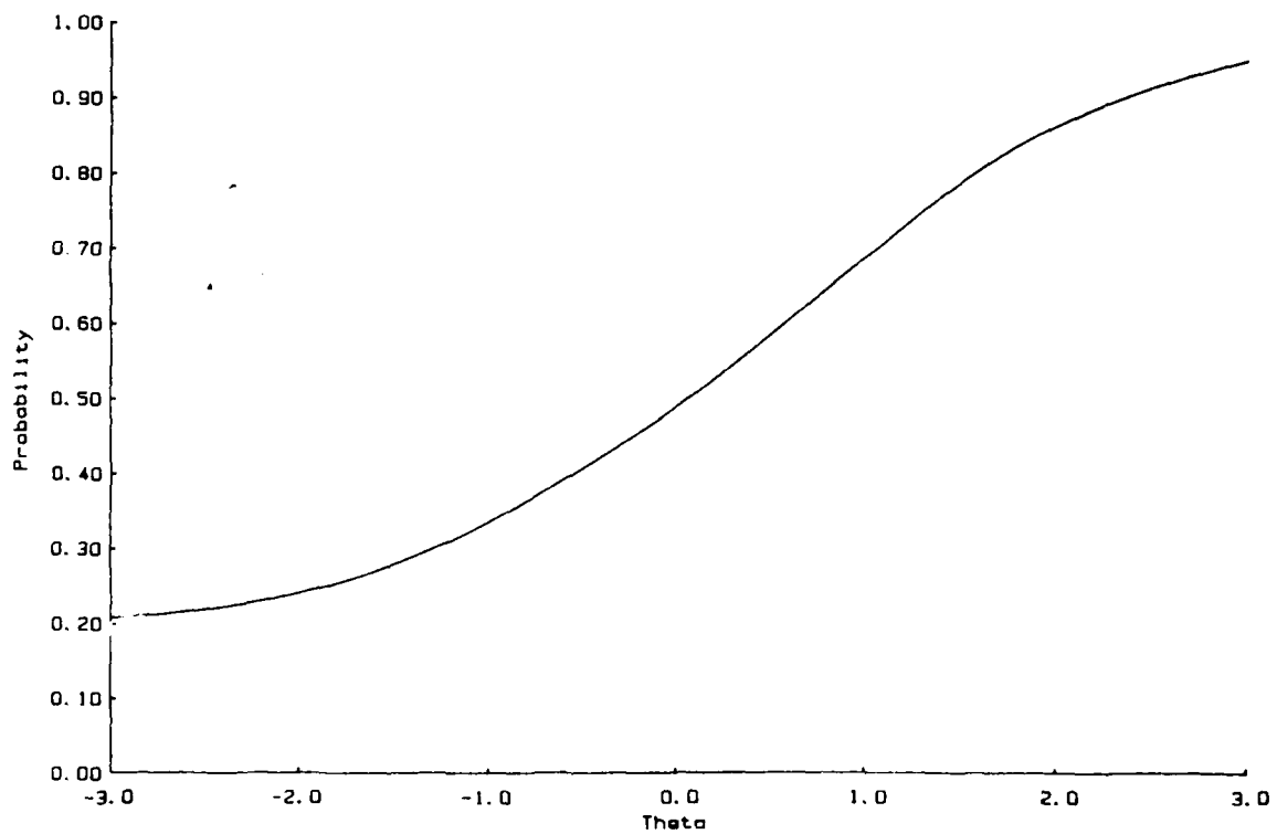
Figure 8-156. Test Characteristic Curve for Mechanical Comprehension Subtest on ASVAB Form 11b (Female Sample).
