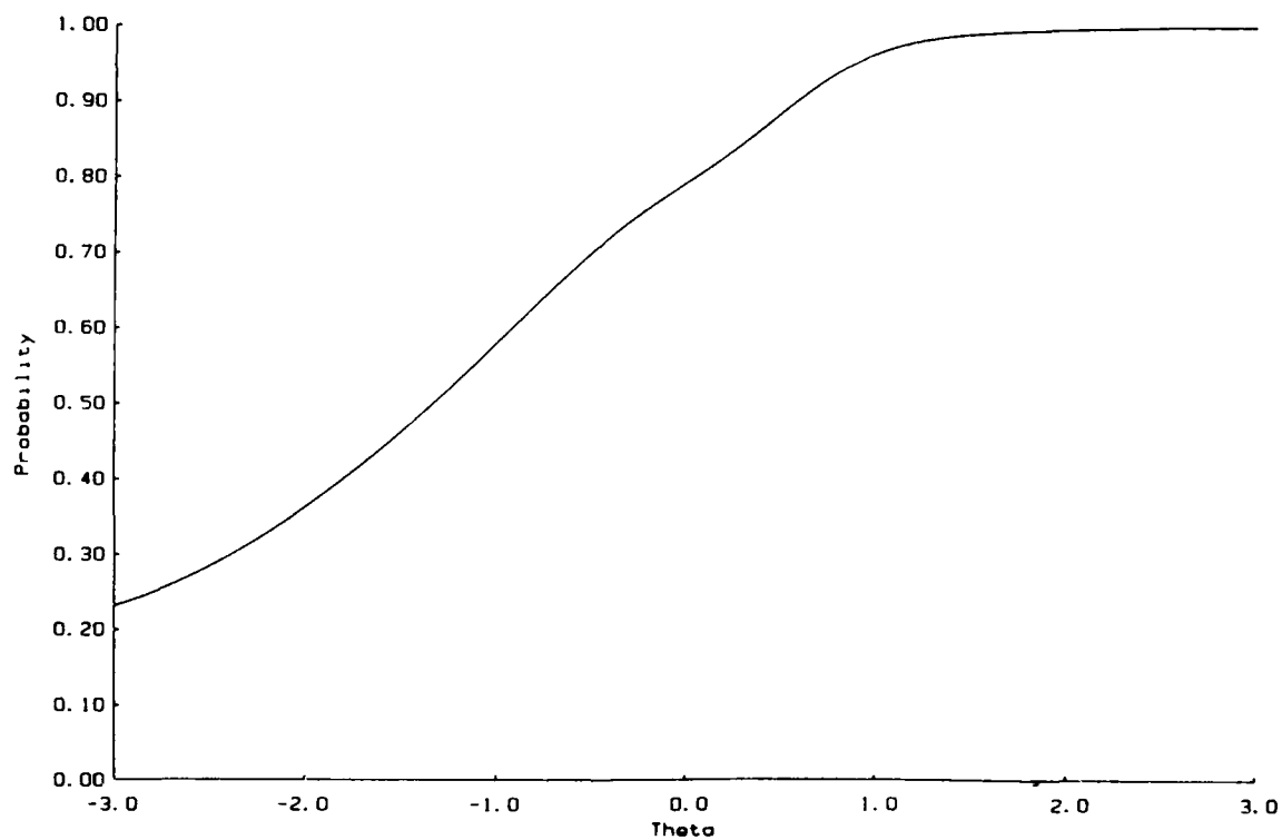
Figure B-82. Test Characteristic Curve for Paragraph Comprehension Subtest on ASVAB Form 13a (Male Sample).
