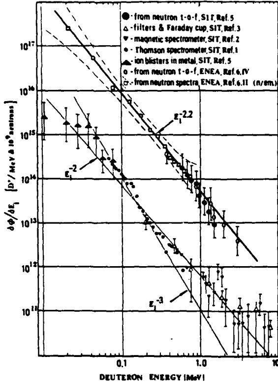
Fig. 2. D^+ energy spectrum d\phi/dE versus E for ejected D^+ ( \blacktriangle , \blacktriangledown , \triangle , \bullet ) and for trapped D^+ ( \circ , \bullet ) from time resolved data. Data from the skin thickness of ion-induced blisters in metals ( =D^+ -range in the metal) covers the range \sim 10 keV to 0.8 MeV. Thomson spectrometer data (from the parabolic pattern of etched ion tracks recorded on CR-39 plastic targets) cover the range 70 keV \leq E \leq 1 MeV. The other two methods cover the range 0.3 MeV \leq E \leq 8 MeV. D^+ spectra from different methods have been normalized to have a minimum-square difference in a chosen E interval. The spectrum from Frascati PF neutron data (trapped D^+ ) is reported for reference. The amplitude factor is normalized to fit SIT Y_n ( 10^9 neutron/shot).
