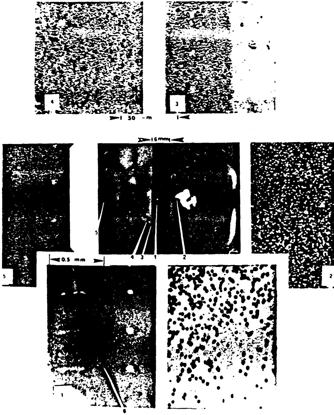
Fig. 2. Zero degree pinhole image of the plasma focus pinch. The central figure shows the typical diameter of the HEB ( = 1.5 \text{ MeV} of \text{D}^+ ) ejected at 0^\circ . Some magnification for 1,2,3,4,5,6 reporting details of center photograph; #1 reports ion tracks of central spots behind 25\mu\text{m} mylar screen.
