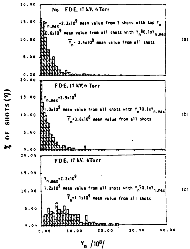
Fig. 3. A field distortion element (circular KE) sharpens the interelectrode current distribution by concentrating it in \geq 2 sheaths. Percentage \eta of shots with a neutron yield between Y_n and Y_n + \Delta Y_n ( \Delta Y_n = 5 \times 10^8 ) versus Y_n without knife edge (in (a)), with KE of length 7.5 mm in contact with the surface of the insulator (pyrex sleeve) at the breach of the PF (in (b)) and at a distance \Delta from the insulator surface (in (c)). Note the elimination of misfirings (i.e., of shots with Y_n < 5 \cdot 10^7 ) if a suitable spacing \Delta between KE and insulator is used as reported in Fig. 4.
