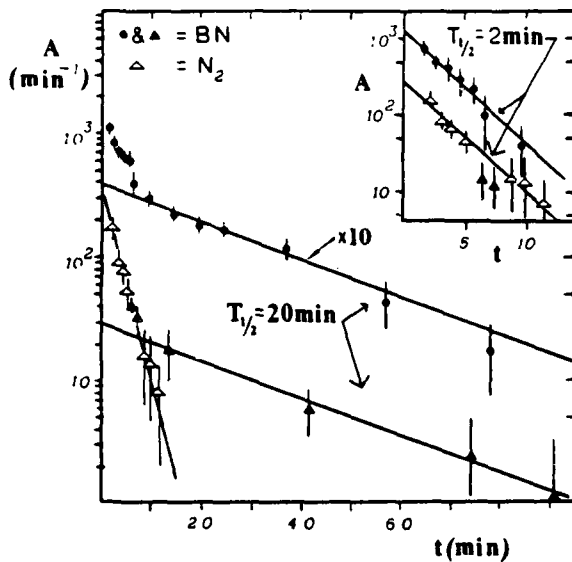
Fig. 1. \beta^- activity A versus \bar{t} (time of activity observation) from shot #1273 (upper line, Y_n = 1.2 \cdot 10^9 ) with solid BN target and pure D_2 filling, and from shot #1339 (lower line, Y_n = 6.8 \cdot 10^8 ) with BN target and N_2 doping (7 percent by pressure \eta = 0.07 ) of D_2 filling at a total pressure p = 6.5 torr ( W_0 = 7 kJ at 17 kV). The reported values of A lack the necessary normalization for different geometric factors involved in the activity measurements on the gas (volume) and on the solid target. The data points \bullet and \blacktriangle refer to the activity of the solid target, the symbol \Delta refers to the gas (volumetric) activity. The beam-induced activity from ^{10}B(d, n)^{11}C(\beta^-) is reported for both shots. In the upper right corner, the activity of ^{15}O from gas and solid target of shot #1339 (lower line) and solid target of shot #1273 ( \times 10 ) are reported with an expanded time axis. Refilling the discharge chamber after each shot (max Y_n = 2.7 \cdot 10^9 , \bar{Y}_n = 6 \cdot 10^8 with doping; max Y_n = 3.8 \cdot 10^9 , \bar{Y}_n = 1.1 \cdot 10^9 with pure D_2 ). Period of PF circuit 9.5 \mu s , discharge chamber \phi , diameter 15.3 cm, length h = 30 cm; center electrode \phi_c , diameter 3.4 cm, h = 13.8 cm; insulator \phi_0 , diameter 4.5 cm, h = 5.2 cm; outer electrode \phi_o , diameter 9.9 cm, h = 11.8 cm; distance Geiger counter window/exposed target surface 3 cm. C, D_n , instead of CH_4 , was used in many series of shots for gas C target activation, with the same results. The error bar is the statistical error.
