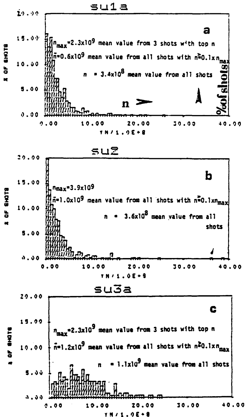
Fig. 5 Histograms with the percentage of shots with a neutron yield between n and n+\Delta n ( \Delta n = 5 \times 10^7 ) vs. n for three different initial configuration of the electric field in the interelectrode gap: (a) no ke; (b) ke touching the insulator surface; (c) ke with same length L = 7.5 mm but with a spacing between insulator surface and ke inner surface. The distribution of the data is substantially changed in (c) as compared to (a), (b) in that the misfirings are almost completely eliminated. Both (b) and (c) indicate a substantial increase of n and of \bar{n} with a record yield of n \sim 3.8 \times 10^9 /shot. All shots in the same conditions: p = 6 Torr, V_0 = 16.5 kV.
