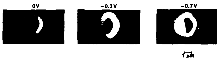
Figure 7. Unbiased and reverse-biased EBIC images of a TaSi 2 rod in a Si matrix.
