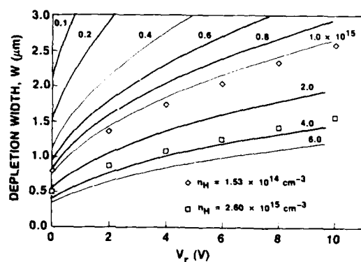
FIG. 4. The dependence of the depletion-zone width ( W ) on the applied reverse-bias voltage ( V_r ). The rod diameter is 1.0 \mu m. The solid lines represent the theoretical relationship calculated from Eq. (13) for different Si-matrix carrier concentrations. The points correspond to EBIC measurements made on two different wafers of widely differing Hall carrier concentration.
