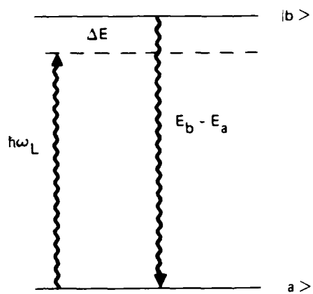
Figure 2. Collisional cooling scheme. The atom absorbs energy h\omega_L and emits energy E_b - E_a . The energy difference \Delta E is carried away by a collision process.
