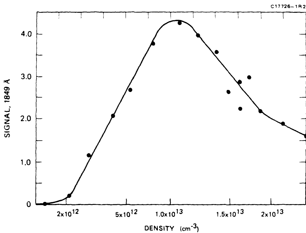
Figure 15. 1849 Å fluorescence as a function of mercury density.
