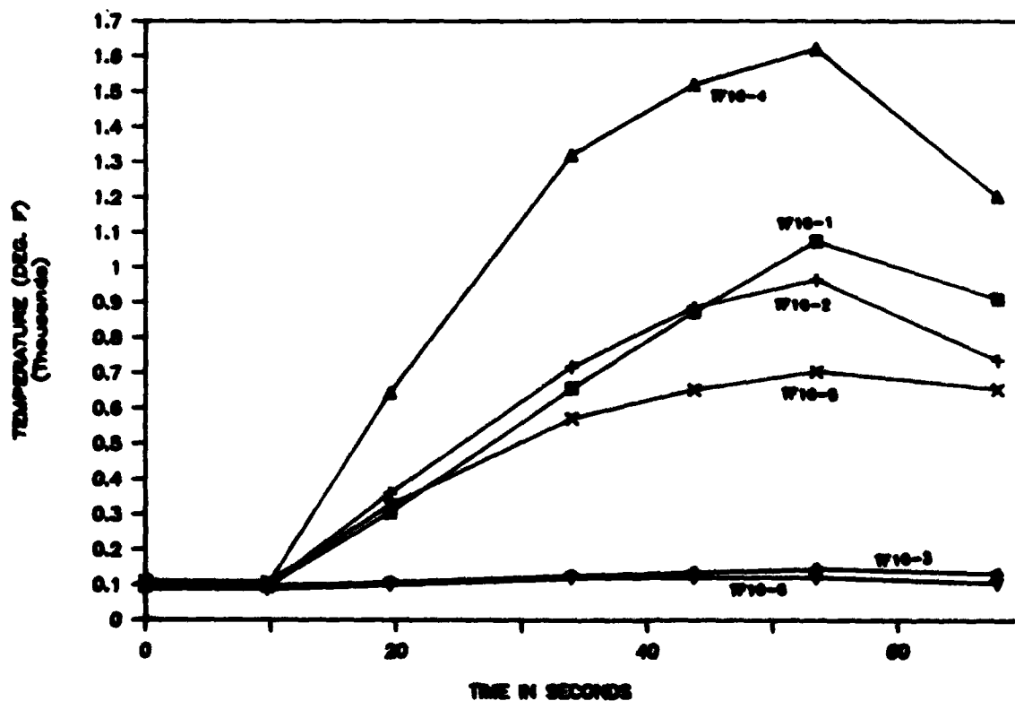
Figure 28. Surface Temperatures on Ribs of P-16 Nozzle Simulator During 0.52 gpm JP-4 Fire
