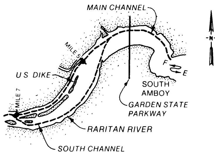
Figure 24. Raritan River Dike
