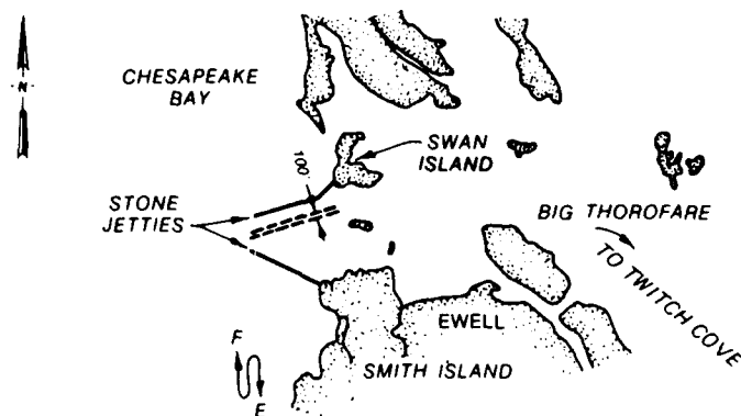
Figure 46. Entrance jetties at the Big Thorofare River
