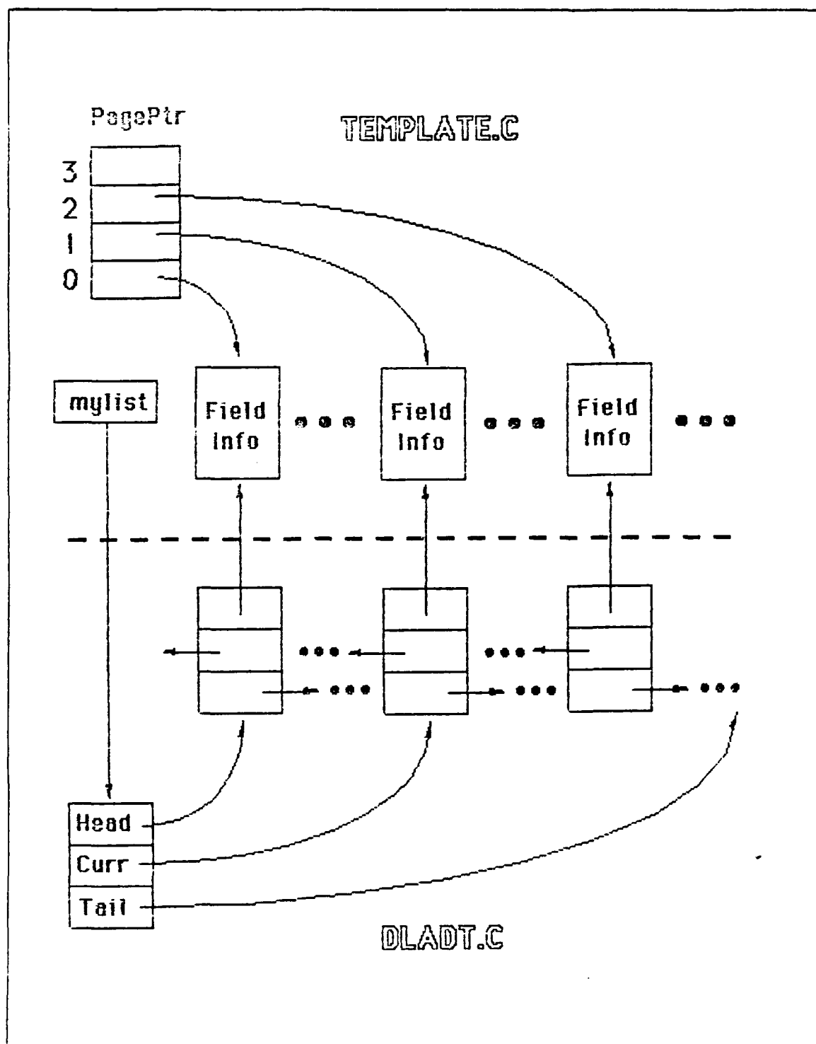
Figure 2. Data Structure for Template.C Program Module
