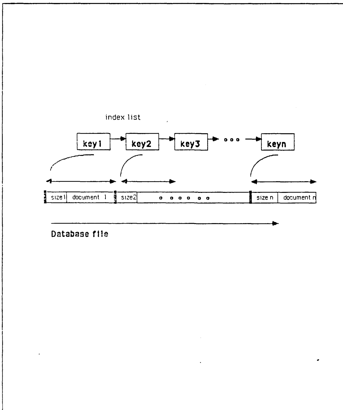
Figure 3. Data Structure for Dbase.C Program Module
