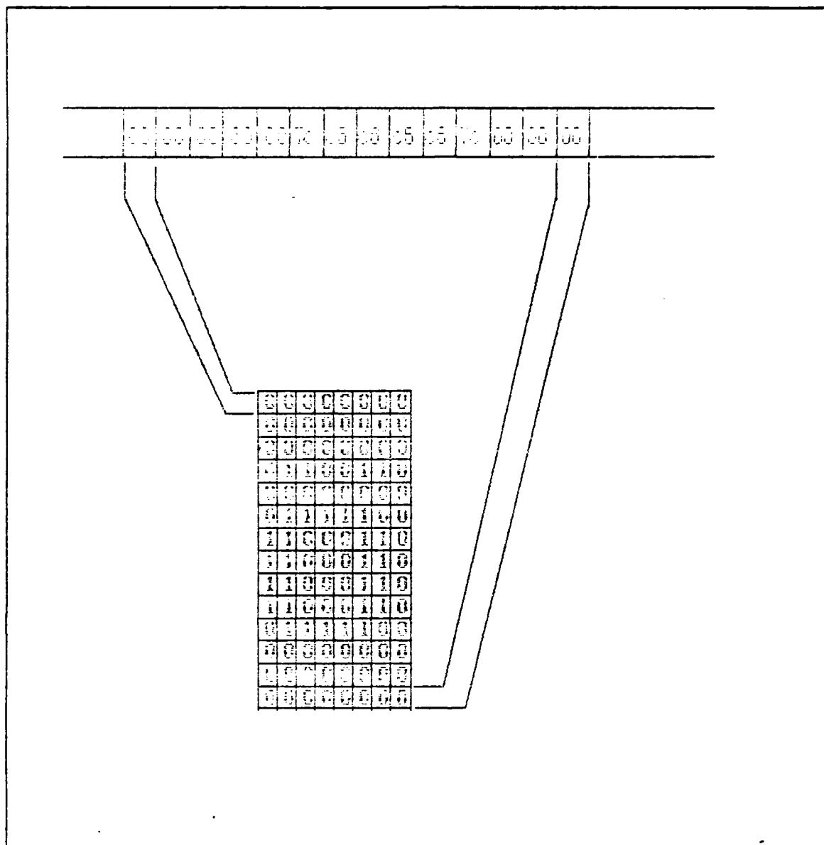
Figure 7. Memory and Screen Representation of Character for EGA
