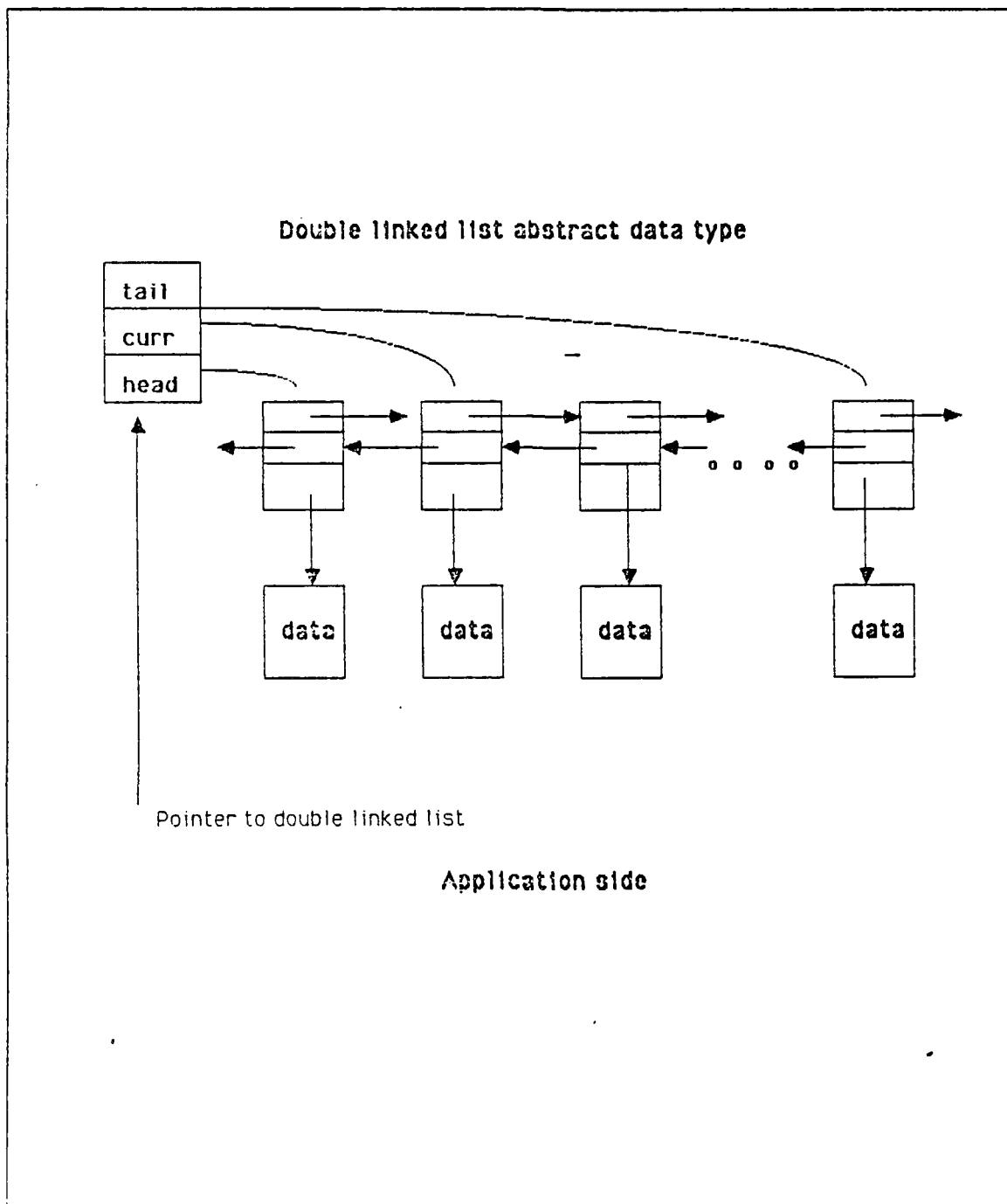
Figure -4. Data Structure for Double Linked List Abstract Data Type
