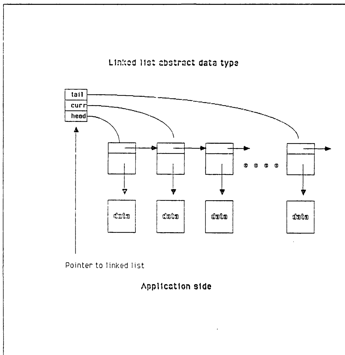
Figure 5. Data Structure for Linked List Abstract Data Type
