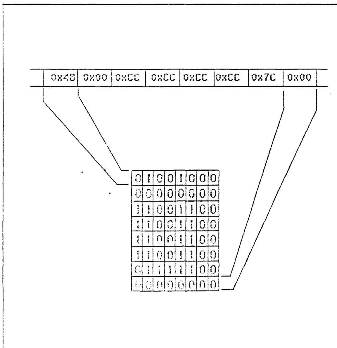
Figure 6. Memory and Screen Representation of Character for CGA
