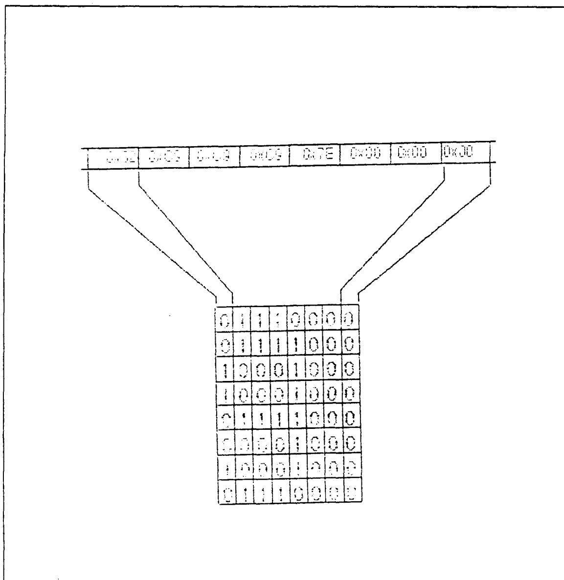
Figure 8. Character Representation for Printer
