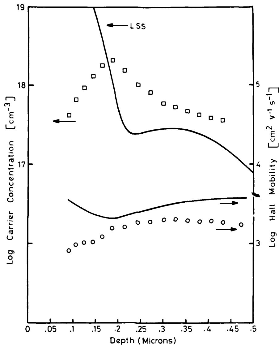
FIG 2 Electron concentration ( \square ) and mobility ( \circ ) depth profiles for 8E12\text{ cm}^{-2} , 360 keV and 4E14\text{ cm}^{-2} , 90 keV, bare implants, annealed at 850^\circ\text{C} for 20 minutes in \text{AsH}_3 overpressure. The calculated carrier concentration (LSS) and mobility profiles are also shown.
