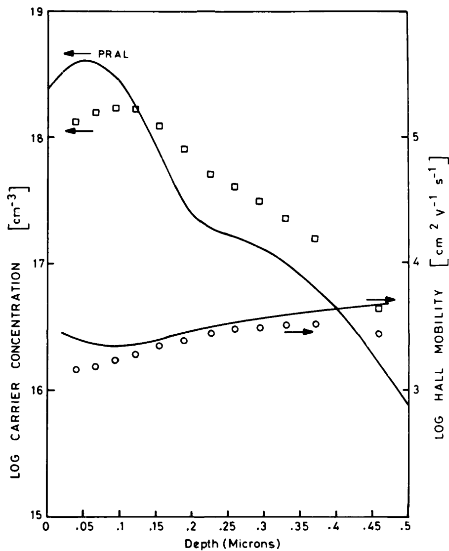
FIG 3 Electron concentration ( \square ) and mobility ( \circ ) depth profiles for 8 \times 10^{12} \text{ cm}^{-2} , 240 keV and 5 \times 10^{13} \text{ cm}^{-2} , 90 keV through 400 Å \text{SiN}_x implants, annealed at 850^\circ\text{C} for 20 minutes in \text{AsH}_3 overpressure. The calculated carrier concentration (PRAL) and mobility profiles are also shown.
