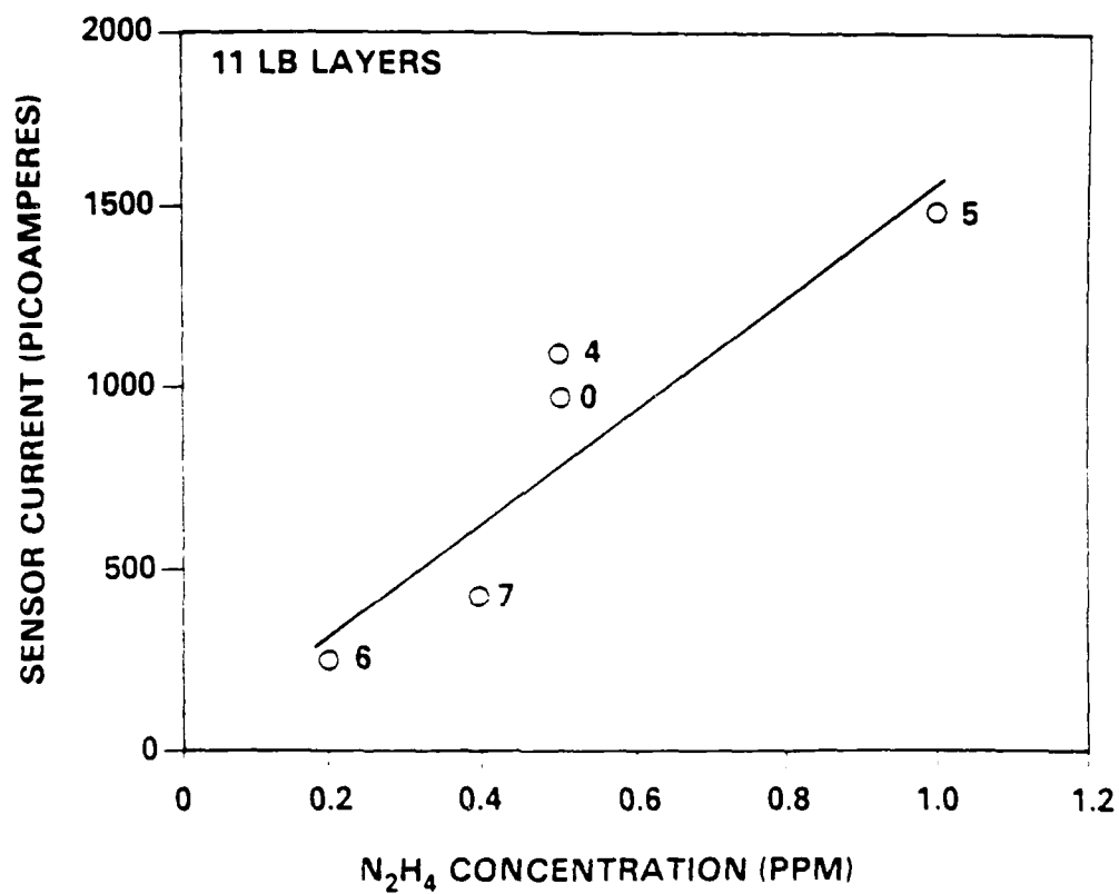
Figure 11. The influence of hydrazine concentration on equilibrium response currents for the 11 LB layer sensor plotted on a linear scale. Numbers next to the data points indicate the day of testing. Only those results from the first seven days of testing are shown.
