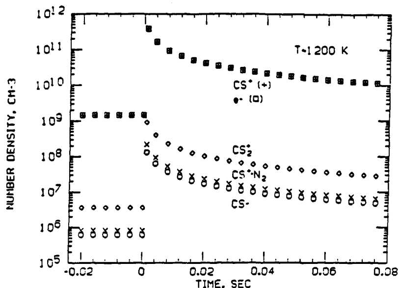
Fig. 1.13a. Species concentrations from numerical solution of kinetics equations for reactions (1.1)-(1.8). T = 1200 K. The following initial species concentrations remain roughly constant: [Cs] = 4.5 \times 10^{14} \text{ cm}^{-3} ; [N_2] = 10^{19} \text{ cm}^{-3} ; [H_2O] = 10^{13} \text{ cm}^{-3} . Two distinct regimes are shown: t < 0 , complete equilibrium; t > 1 \text{ ms} , plasma relaxation. Photoionization occurs between these regimes.
