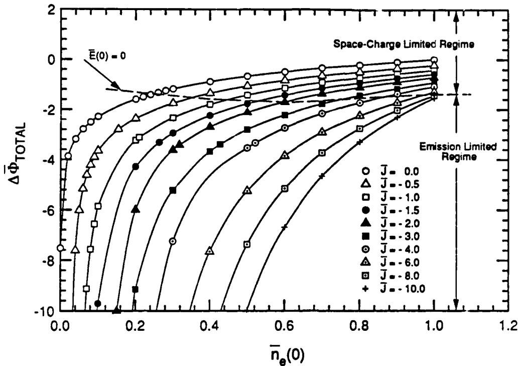
Fig. 2.9. Cathode potential fall \Delta\bar{\Phi}_{\text{total}} versus \bar{n}_e(0) with current \bar{J} as a parameter, showing the distinction between the space-charge-limited and emission-limited regimes.
