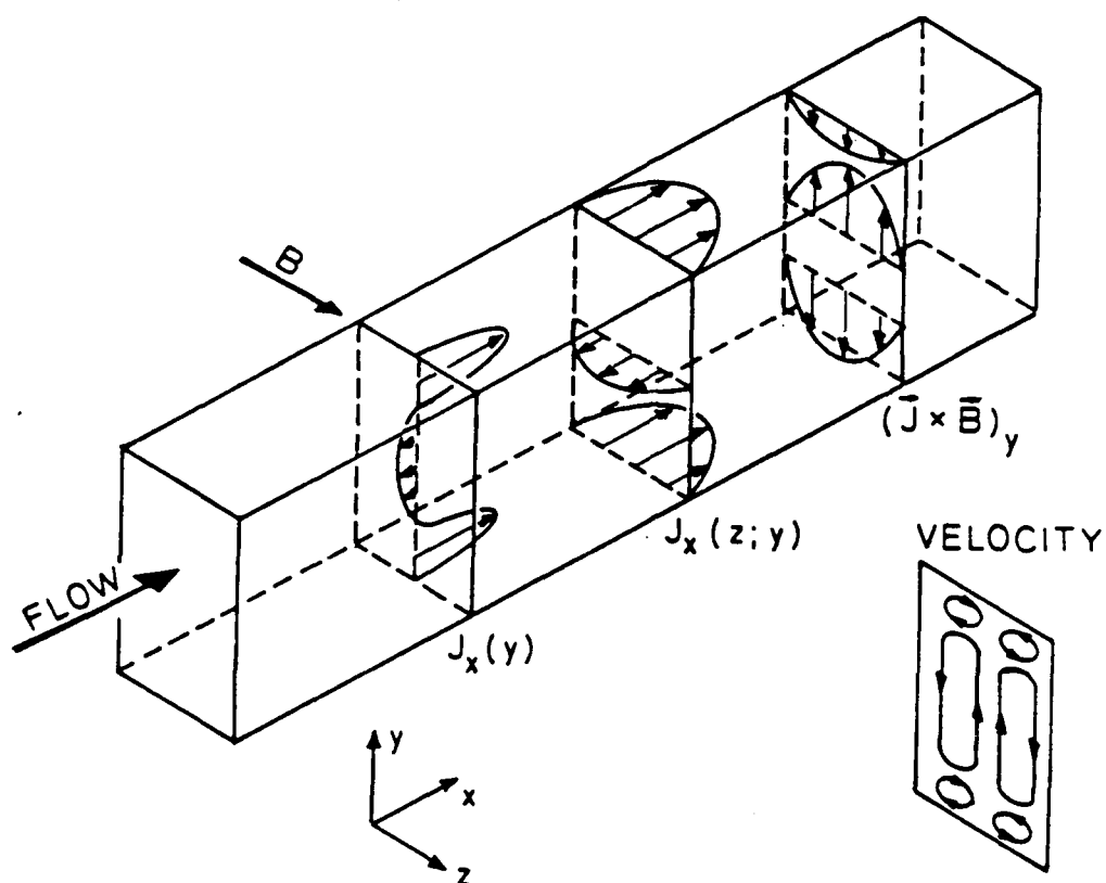
Fig. 3.3. Secondary flow mechanism for a segmented Faraday generator (zero net Hall current).
