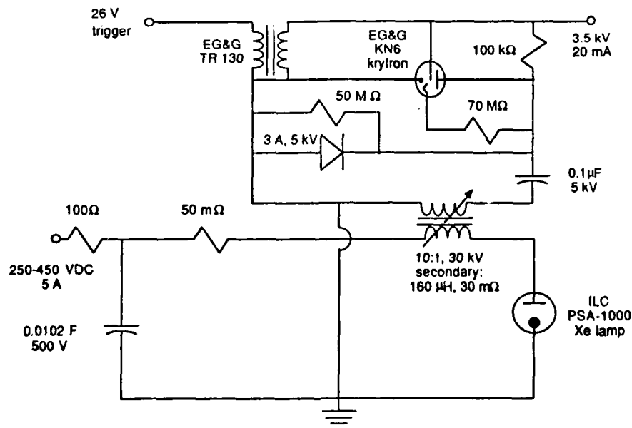
Fig. 1.17. Flashlamp circuit.
