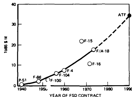
FIGURE 1. RECURRING FLYAWAY COST OF FIGHTER AIRCRAFT
