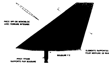
FIG. 18 - ACE/RAFALE - FOREPLANE (SPF-DB)
