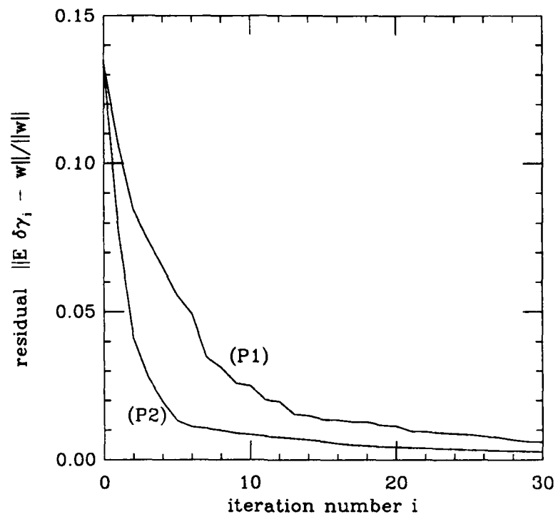
Figure 10a Reduction in the relative problem residual versus number of iterations.
