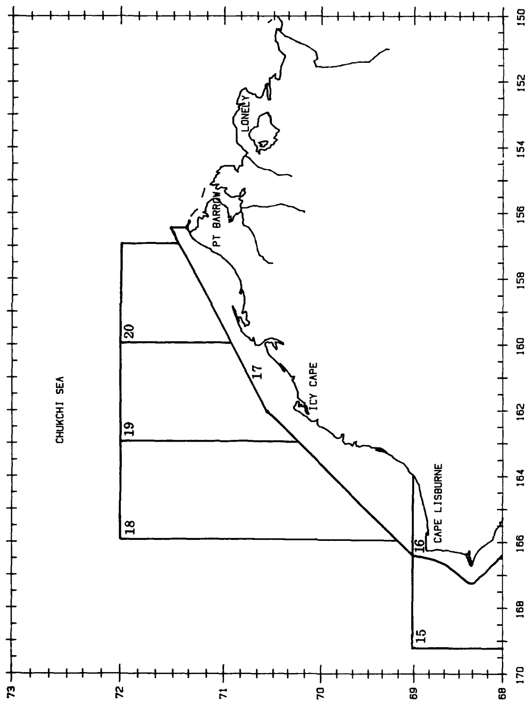
Figure B-5. Map depicting coastal survey regions 16 and 17 and offshore regions 15, 18, 19 and 20.
