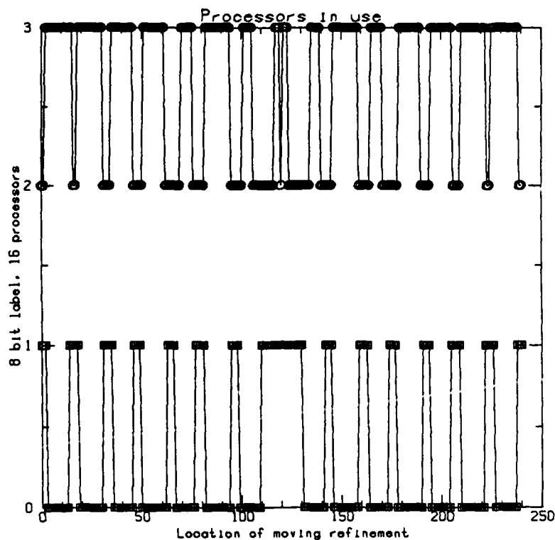
Figure 4: Processor load for 16 processors and an 8 bit label. The refinement is 16 cells long. The top line is the maximum number of cells per processor; the bottom line is the minimum number of cells per processor.
