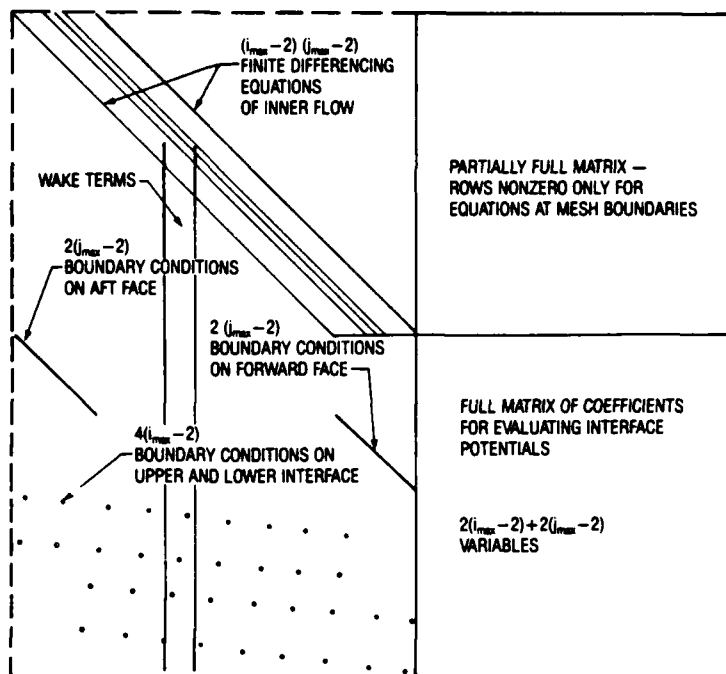
Figure 7. Schematic of the Coefficient Matrix Used in Combining Inner and Outer Solutions.
