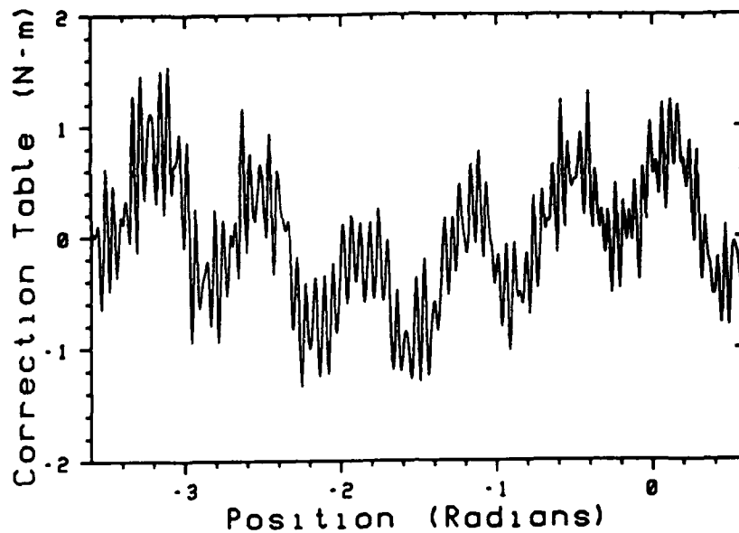
Figure 6.6 Lookup Table Correction to Torques Applied at Joint Two of the PUMA 560.
