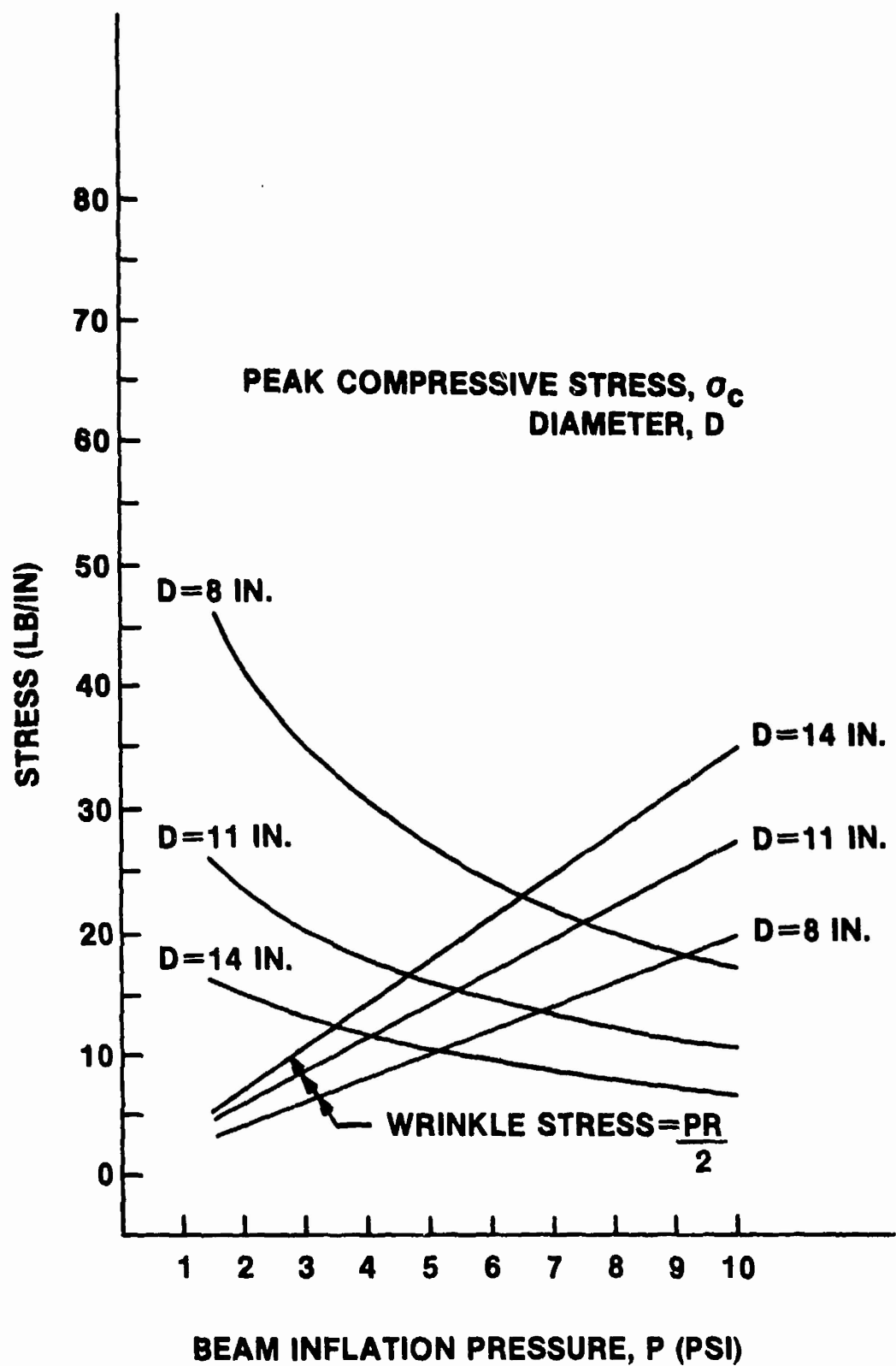
FIGURE C.3: Peak compressive and wrinkle stress vs. inflation pressure for 400 sq ft Leaning Arch BAS, 30 mph wind load
