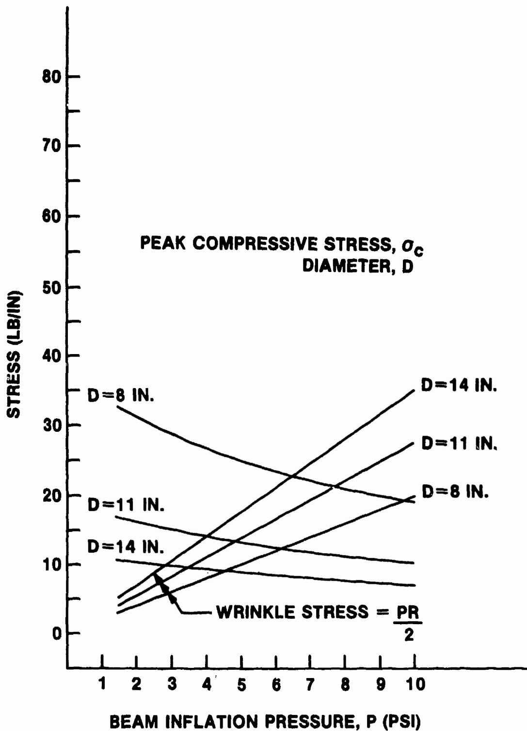
FIGURE C.20: Peak compressive and wrinkle stress vs. inflation pressure for 300 sq ft Vertical Arch BAS, 5 psf snow load.
