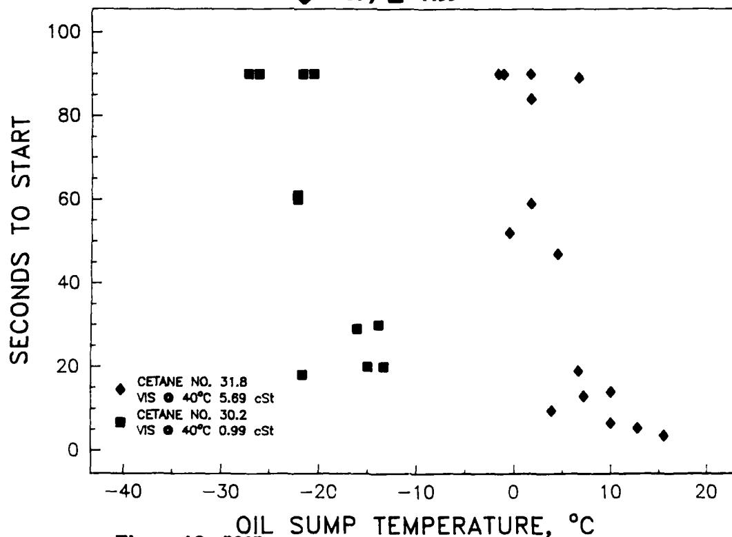
Figure 12. "30" cetane number fuels - GM 6.2L engine
