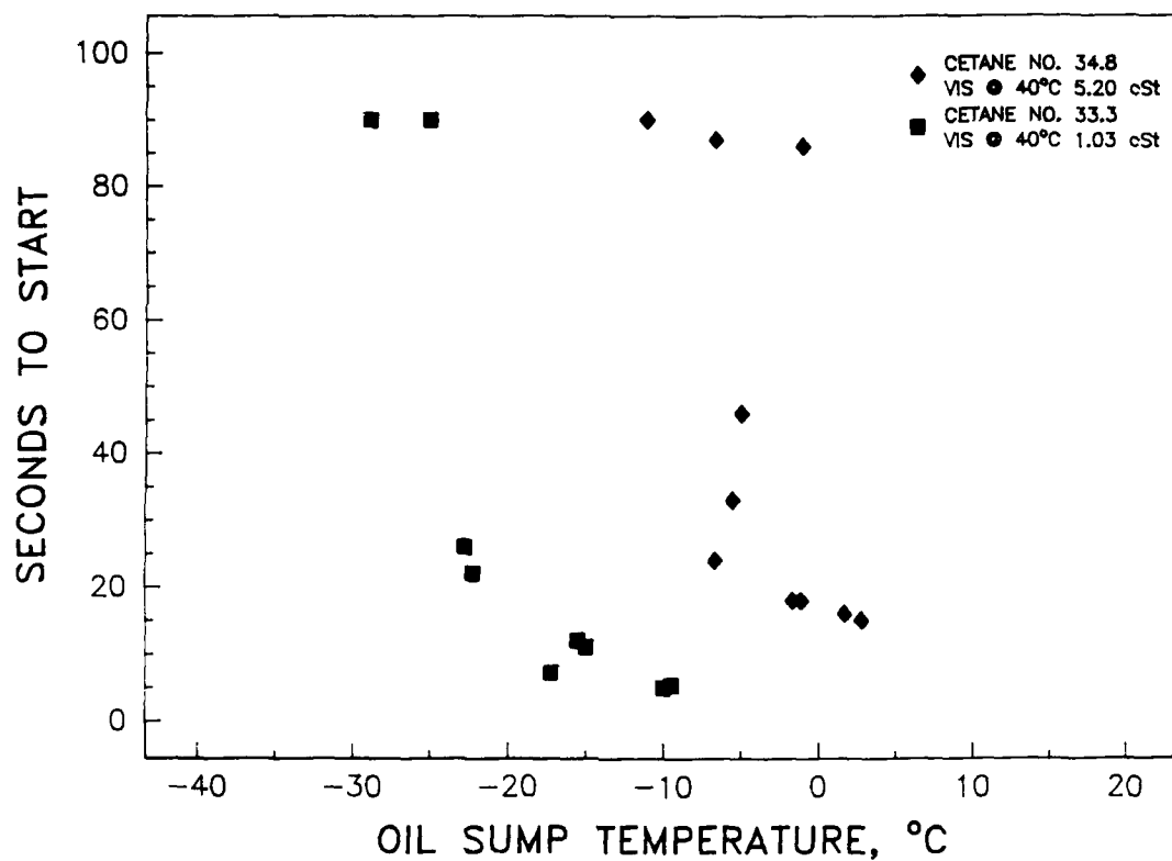
Figure 11. "35" cetane number fuels - GM 6.2L engine
