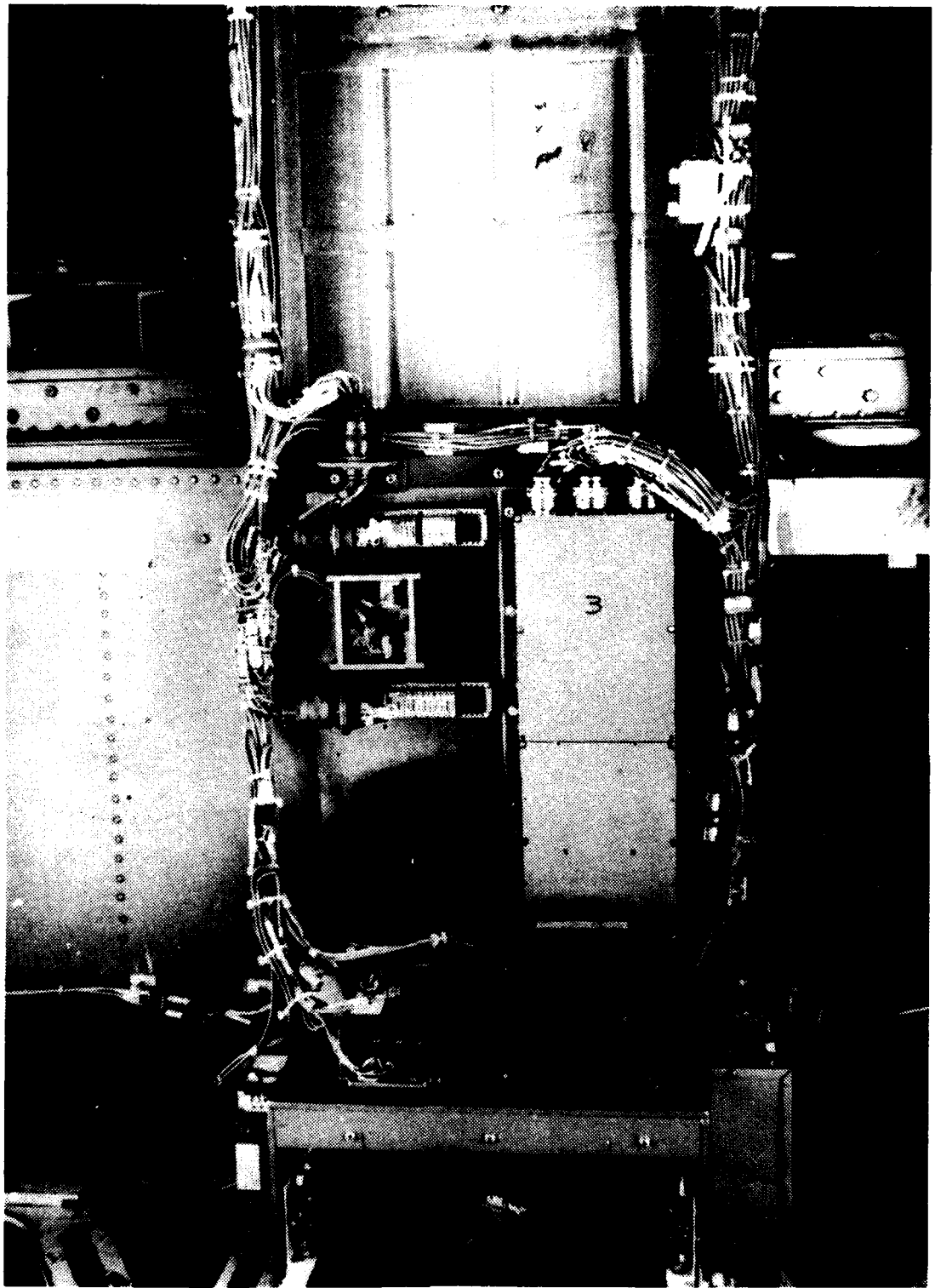
Figure C-5. Instrumentation Package (Aft Cabin - Center)
