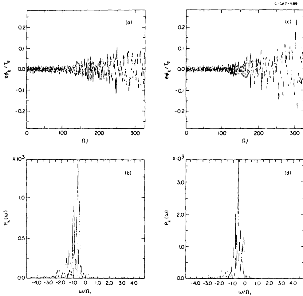
Fig. 14. The time evolution of perturbation of electrostatic potential ((a), (c)) and their power spectrum ((b), (d)) in the case of \alpha = E_{ox}^2 / 4\pi n_e T_e = 2.24 , v_E^0 = 2.0v_{it} , k_{||}\lambda_{ell} = 0.005 \times 2\pi \times 2/32 = 1.96 \times 10^{-3} , and k_y\lambda_{ell} = 2\pi/32 = 0.393 .
