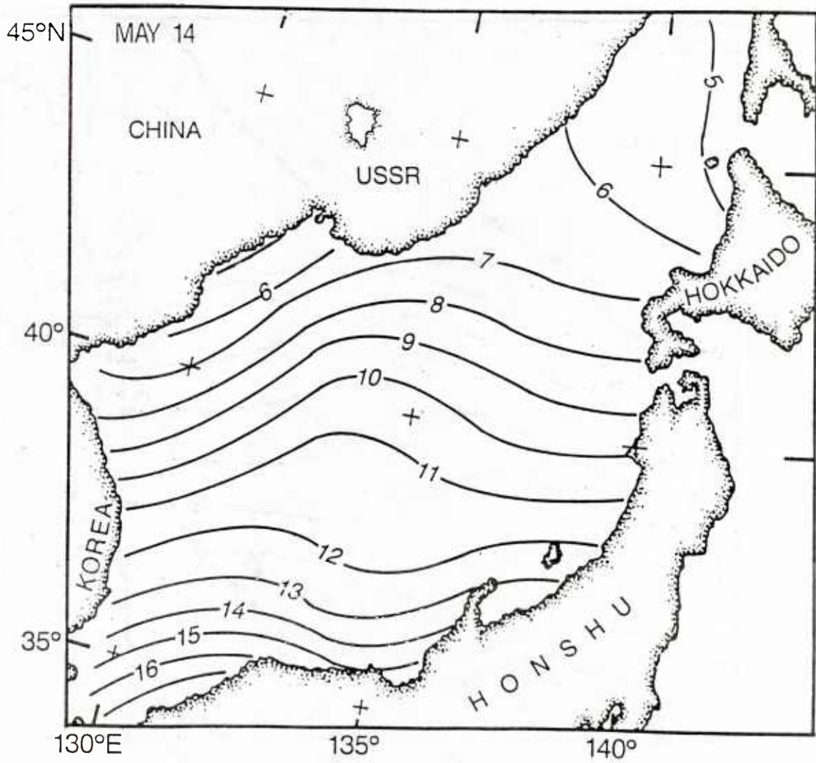
Figure 12. Zoomed EOTS SST ( ^{\circ}\text{C} ) for May 14, 1984.
