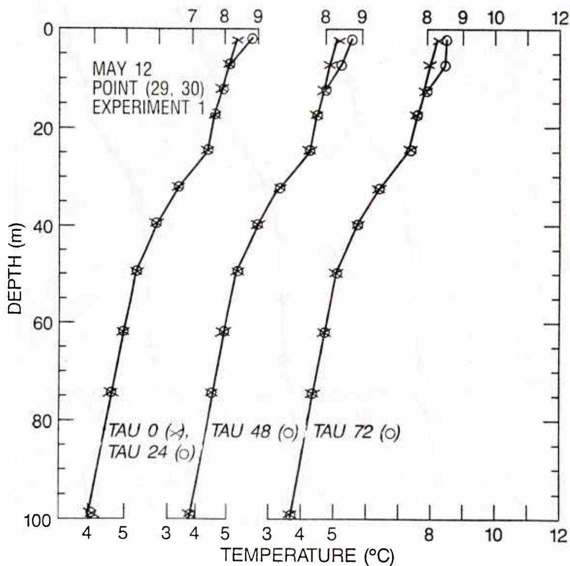
Figure 57. Experiment 1 temperature vs. depth for May 12, 1984, frontal point (29,30), (x) TAU 0, (o) TAU 24, TAU 48, and TAU 72.
