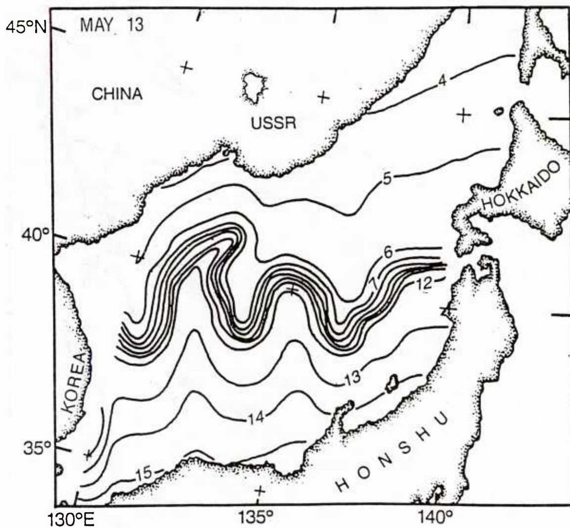
Figure 22. Synthetic SST ( ^{\circ}\text{C} ) field for May 13, 1984.
