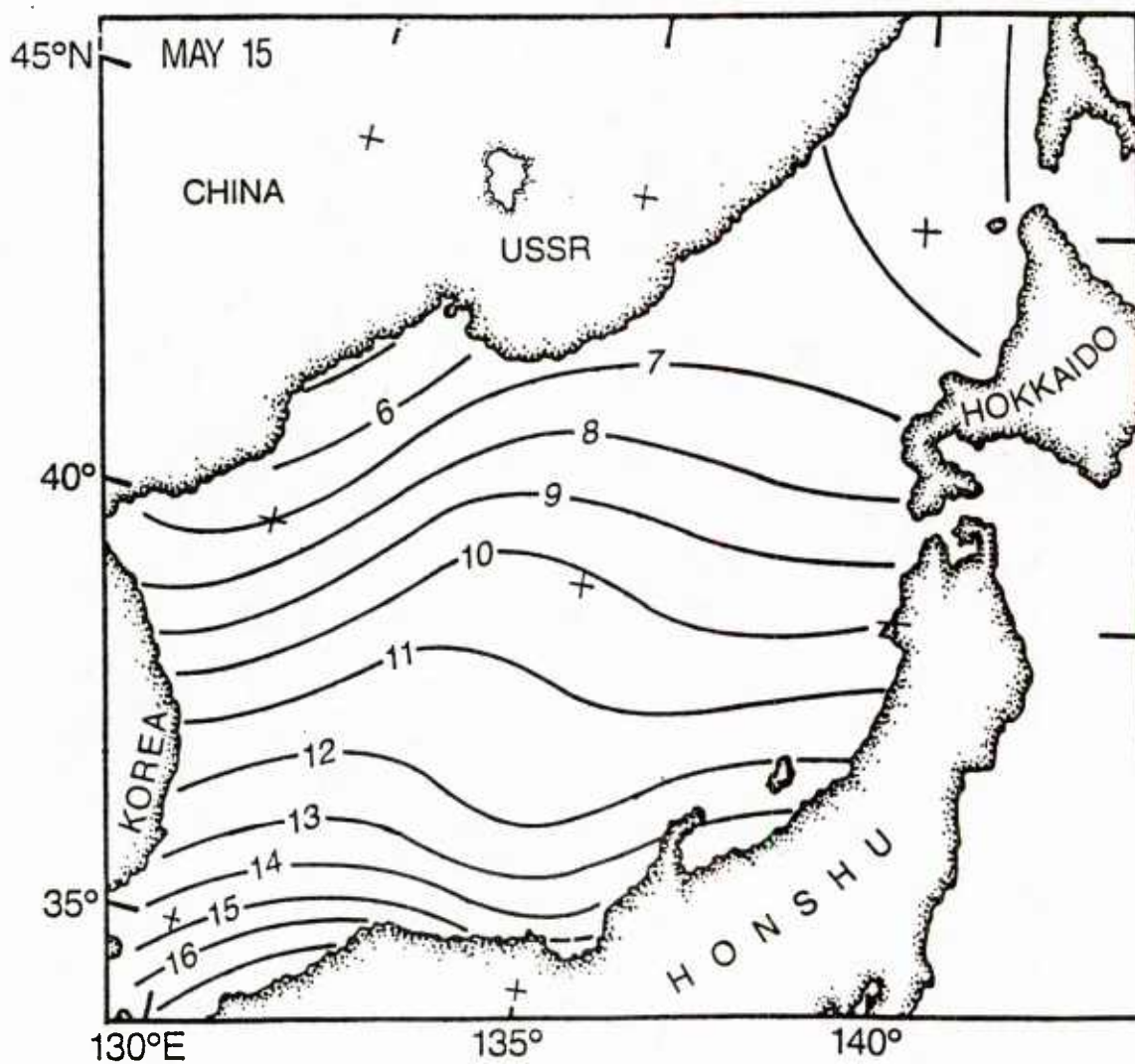
Figure 13. Zoomed EOTS SST ( ^{\circ}\text{C} ) for May 15, 1984.
