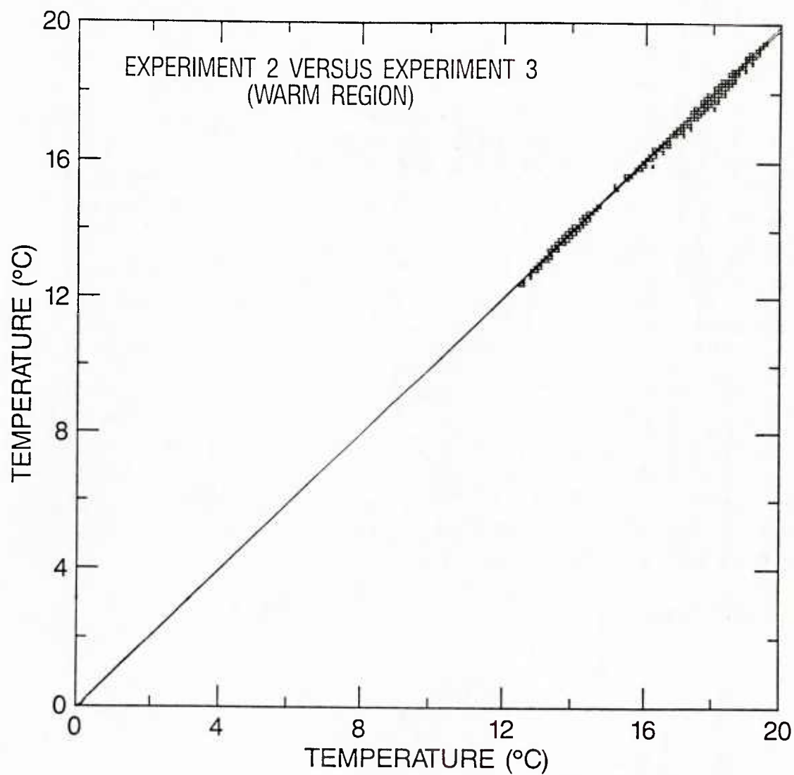
Figure D3a. Scatter plot of TAU 72 SST (°C) forecasts covering May 8 - June 4, 1984, for experiment 2 vs. experiment 3 (warm side).
