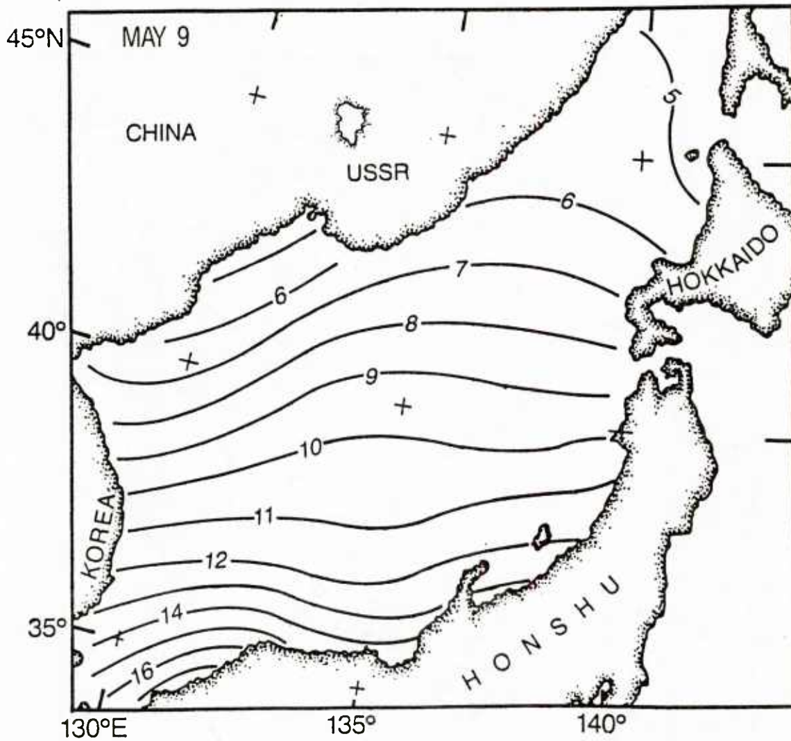
Figure 7. Zoomed EOTS SST ( ^{\circ}\text{C} ) for May 9, 1984.
