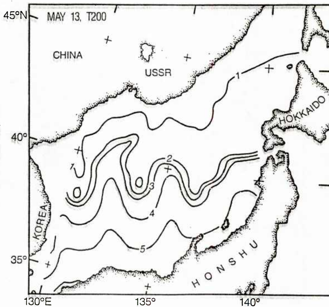
Figure 29. Frontally modified, daily, EOTS temperature ( ^{\circ}\text{C} ) at 200 m for May 13, 1984,
