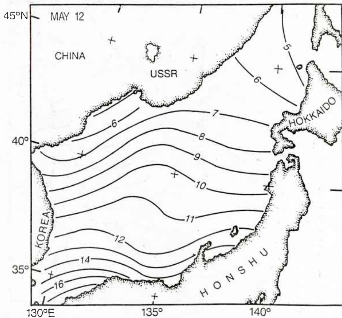
Figure 10. Zoomed EOTS SST ( ^{\circ}\text{C} ) for May 12, 1984.
