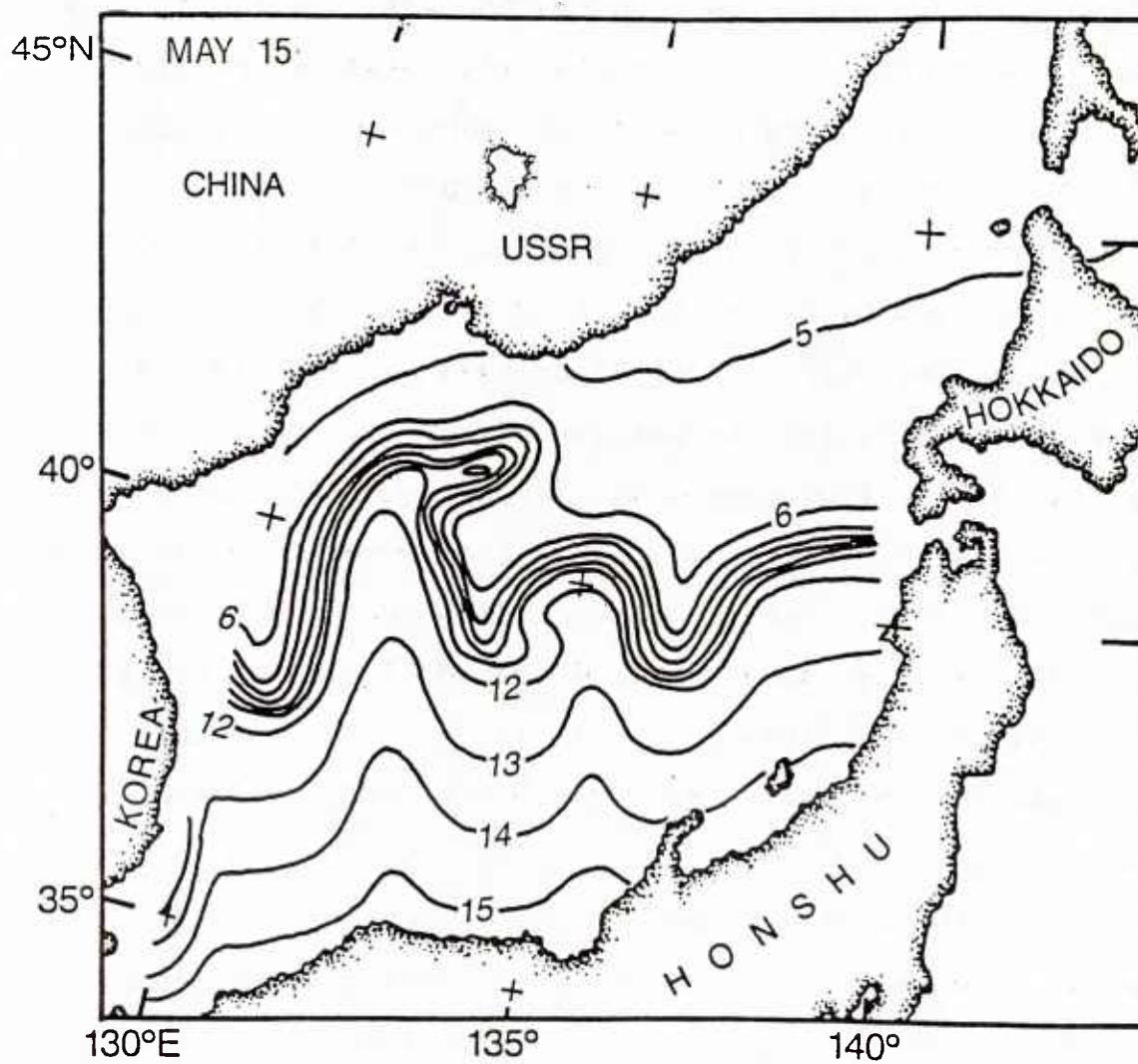
Figure 24. Synthetic SST ( ^{\circ}\text{C} ) field for May 15, 1984.
