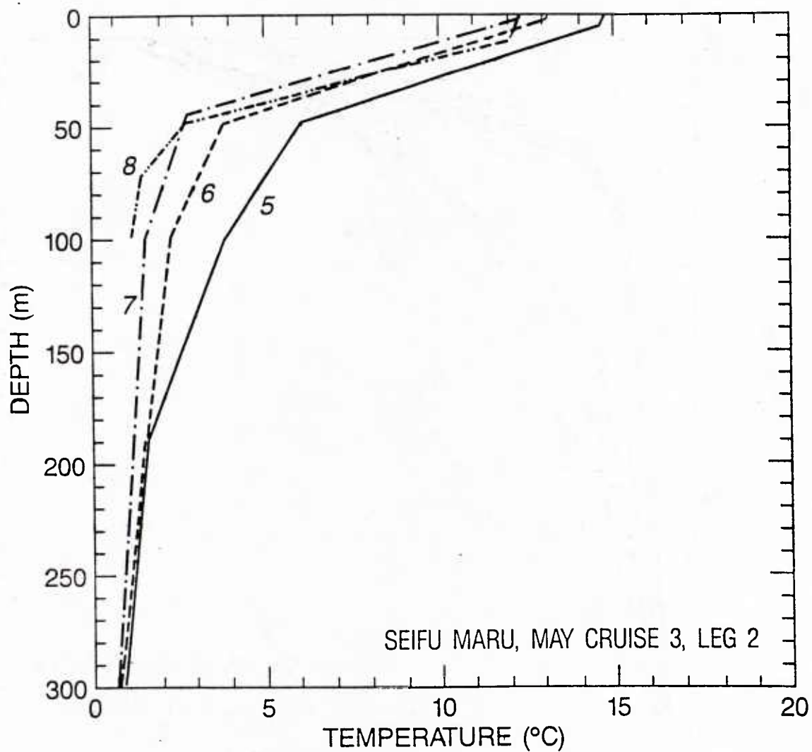
Figure 38b. Temperature profiles for leg 2 of May 25-27, 1984, Seifu Maru cruise.
