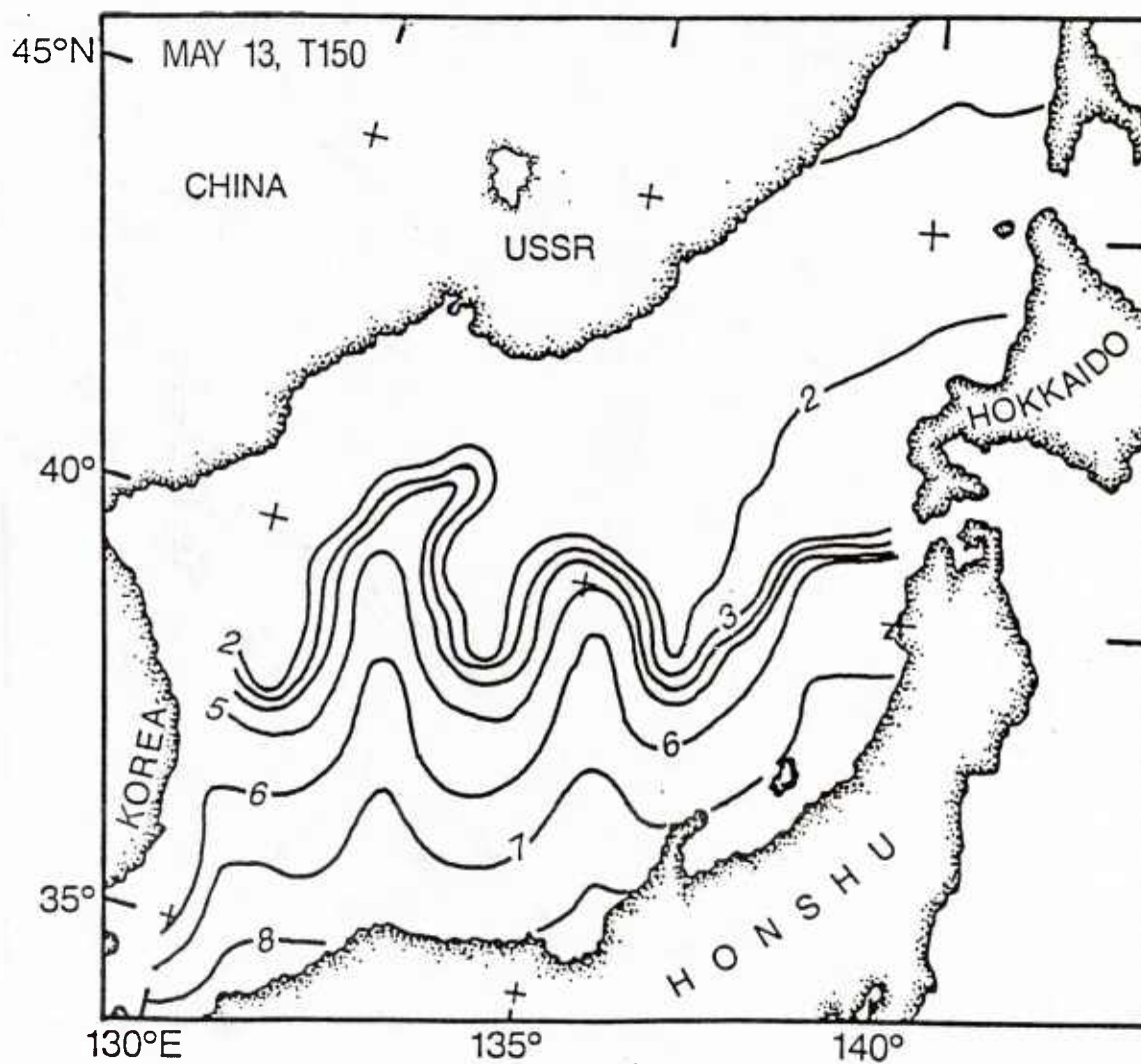
Figure 28. Frontally modified, daily, EOTS temperature ( ^{\circ}\text{C} ) at 150 m for May 13, 1984.
