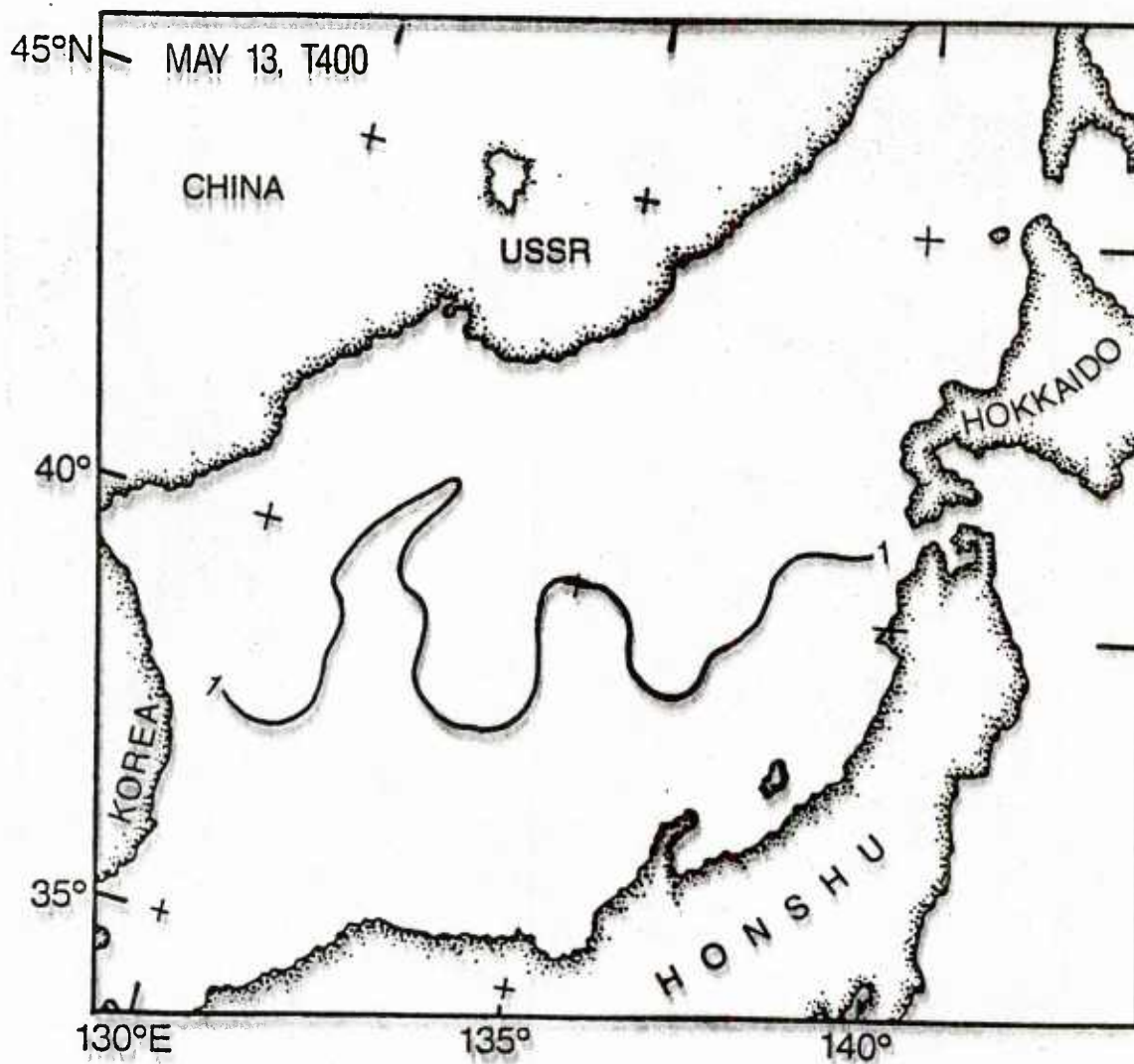
Figure 31. Frontally modified, daily, EOTS temperature ( ^{\circ}\text{C} ) at 400 m for May 13, 1984.
