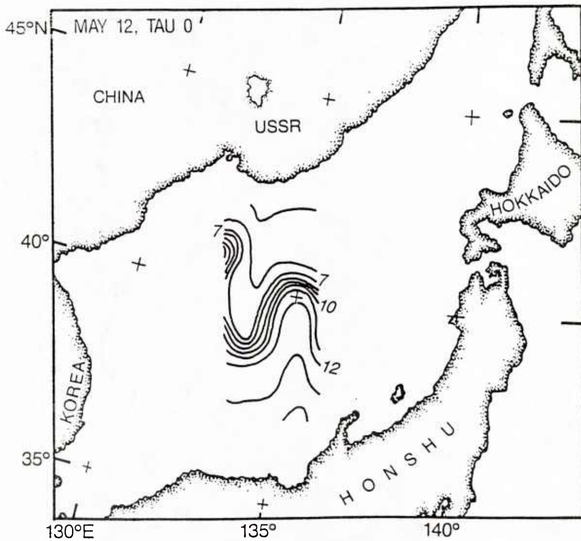
Figure 48. Initial condition SST (contour interval = 1°C), for May 12, 1984, forecast.
