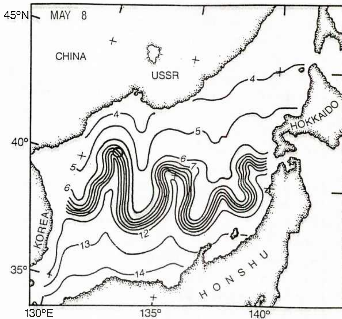
Figure 17. Synthetic SST ( ^{\circ}\text{C} ) field for May 8, 1984.
