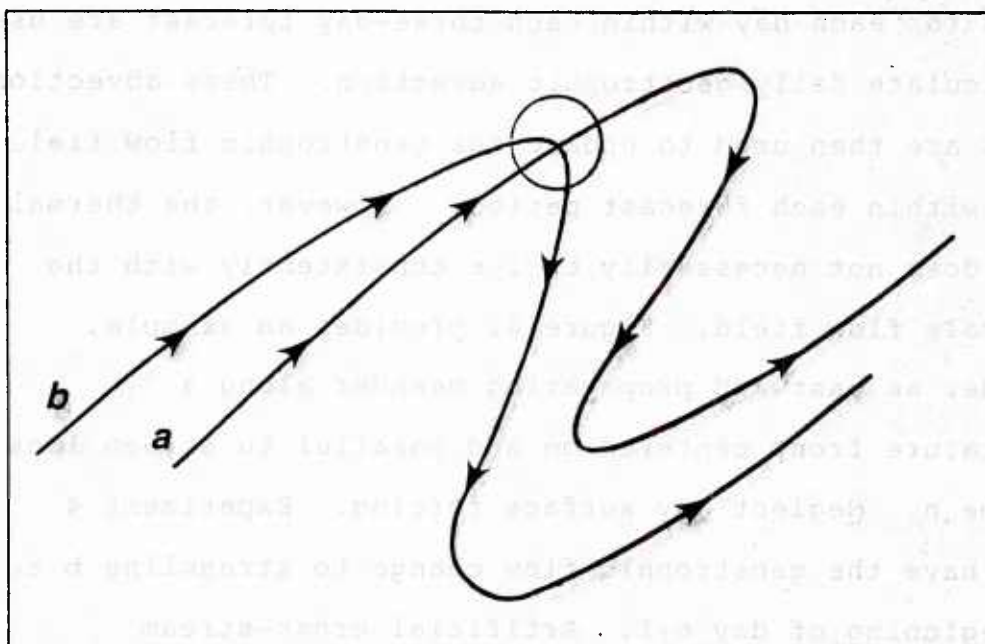
Figure 42. Schematic illustrating potential for artificial cross-frontal advection in experiment 4.
