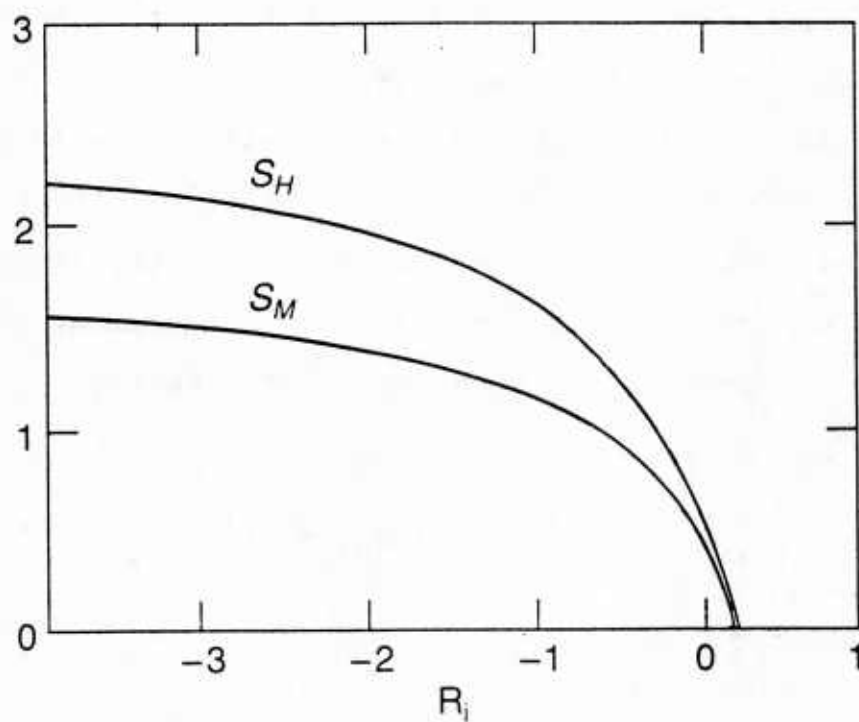
Figure 4. Stability functions, S_H and S_M , as a function of gradient Richardson number.
