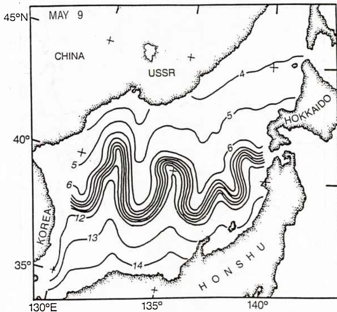
Figure 18. Synthetic SST ( ^{\circ}\text{C} ) field for May 9, 1984.
