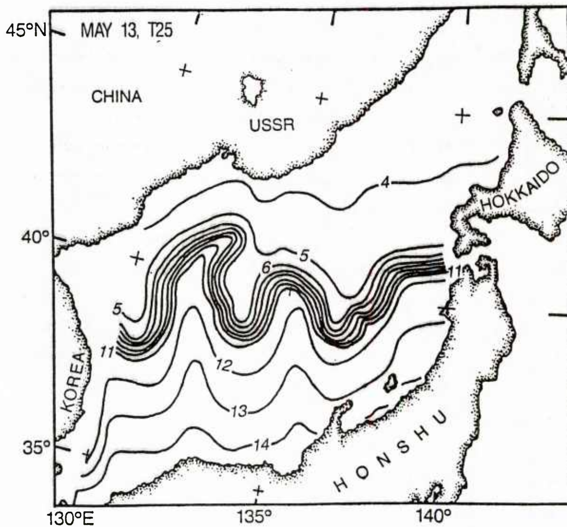
Figure 25. Frontally modified, daily, EOTS temperature ( ^{\circ}\text{C} ) at 25 m for May 13, 1984.
