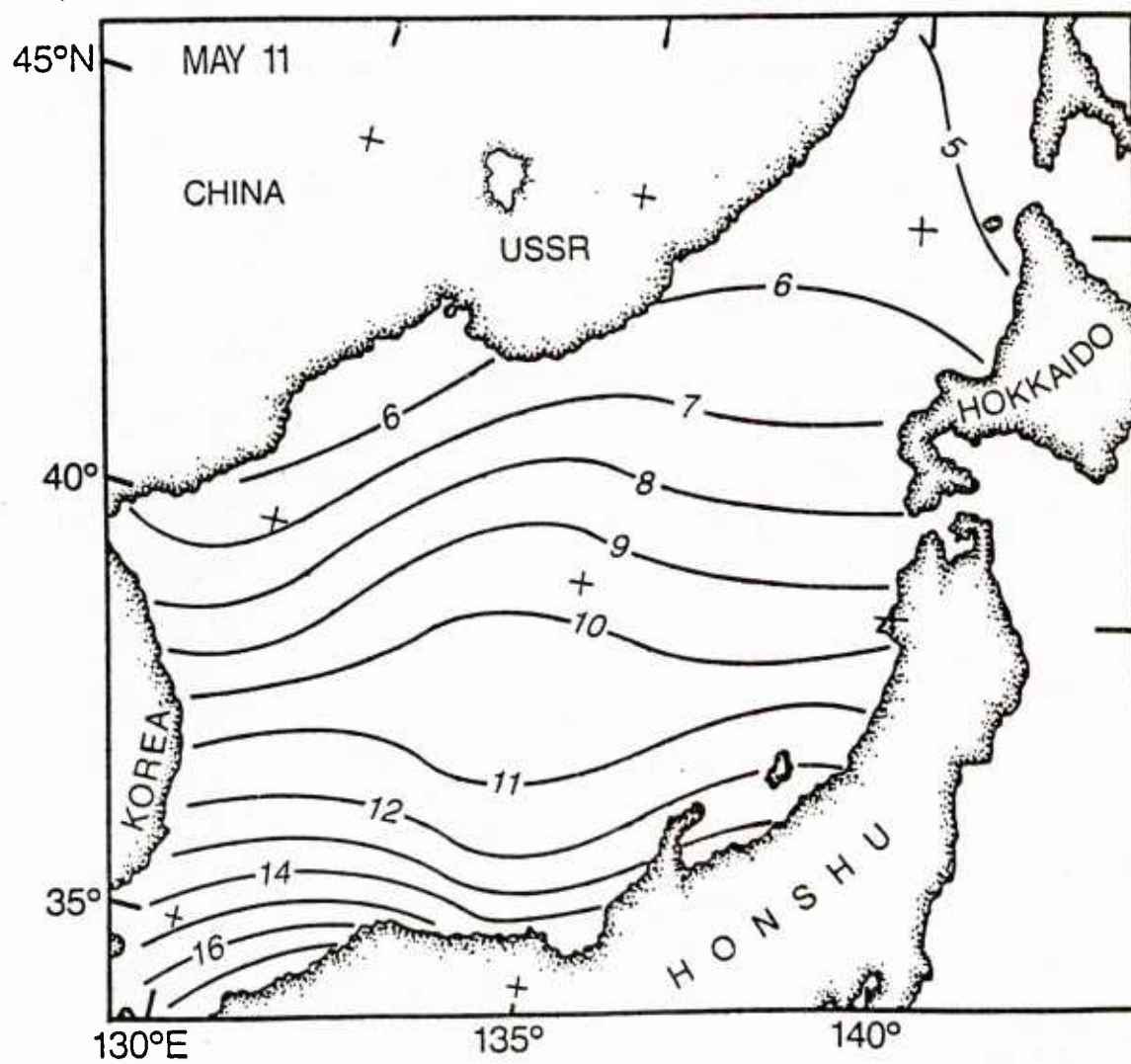
Figure 9. Zoomed EOTS SST ( ^{\circ}\text{C} ) for May 11, 1984.
