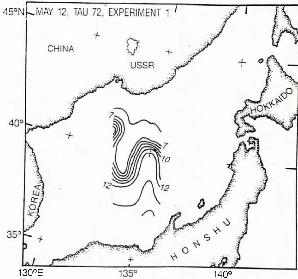
Figure 49a. Forecast SST ( ^{\circ}\text{C} ), experiment 1, May 12, 1984, TAU 72.
