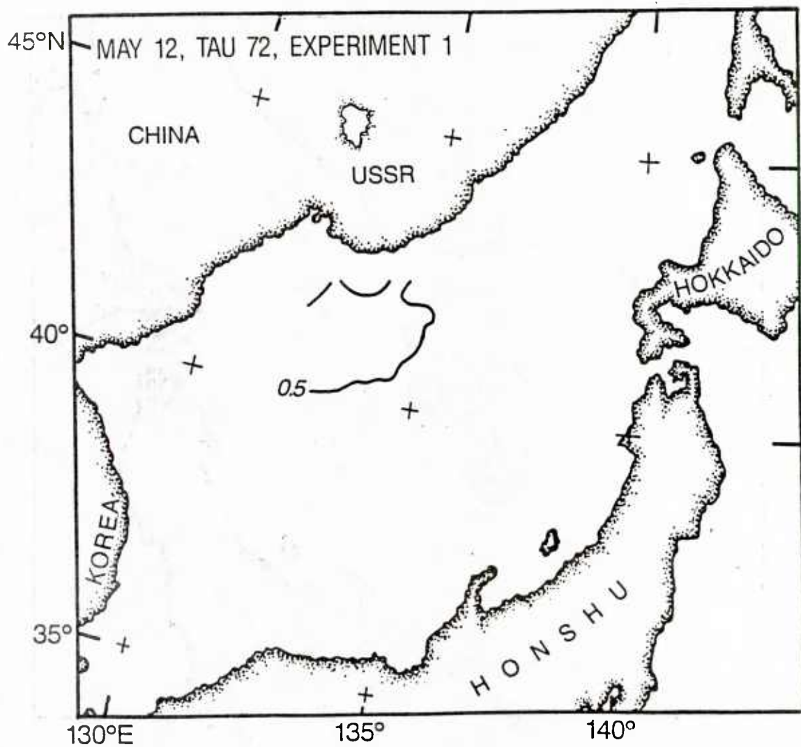
Figure 51a. Forecast SST change (contour = 0.5^{\circ}\text{C} ), experiment 1, May 12, 1984, TAU 72.
