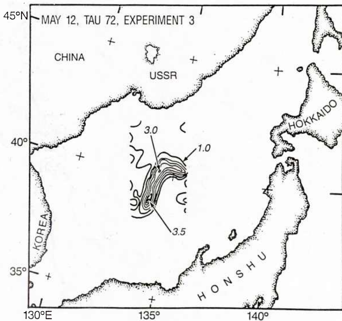
Figure 51c. Forecast SST change (contour = 0.5°C), experiment 3, May 12, 1984, TAU 72.
