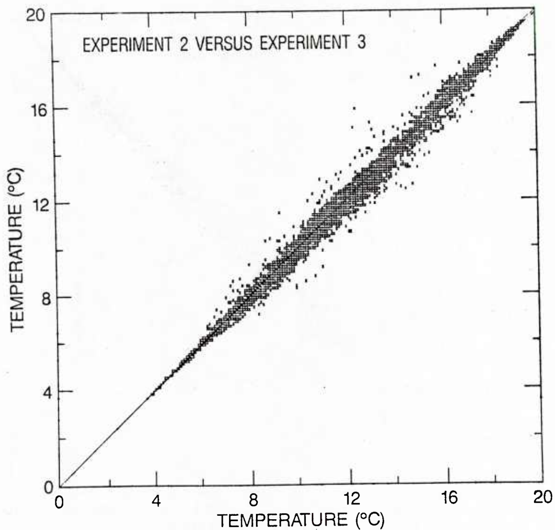
Figure 46c. Scatter plot of TAU 72 SST ( ^{\circ}\text{C} ) forecasts covering May 8 - June 4, 1984, for experiment 2 vs. experiment 3.
