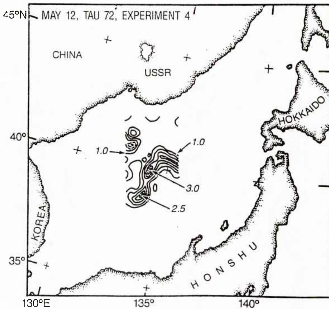
Figure 51d. Forecast SST change (contour = 0.5°C), experiment 4, May 12, 1984, TAU 72.
