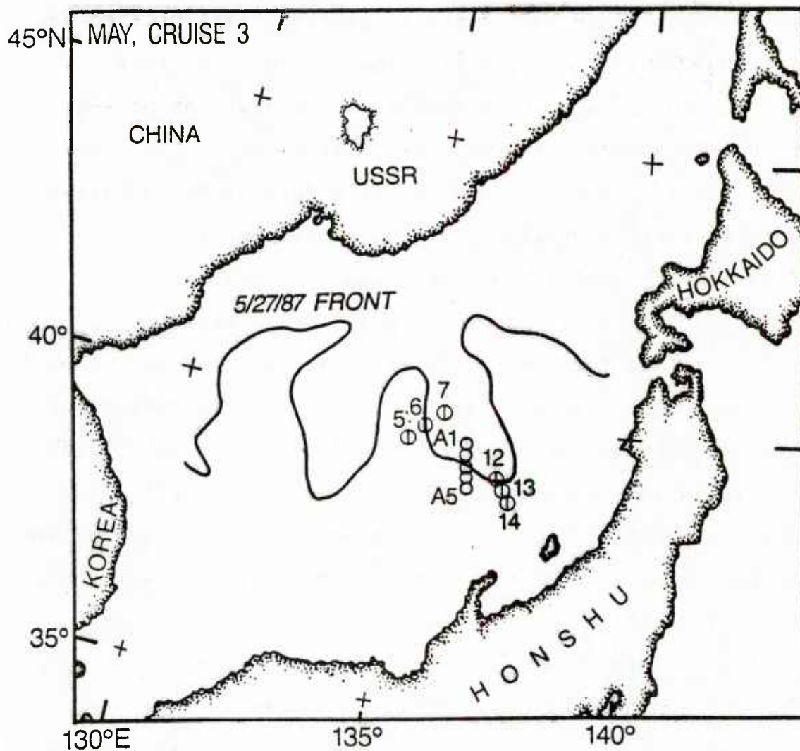
Figure 39. May 27, 1984, interpolated frontal position with appropriate Seifu Maru cross-frontal stations marked. A1-A5 denote model cross-frontal grid points.
