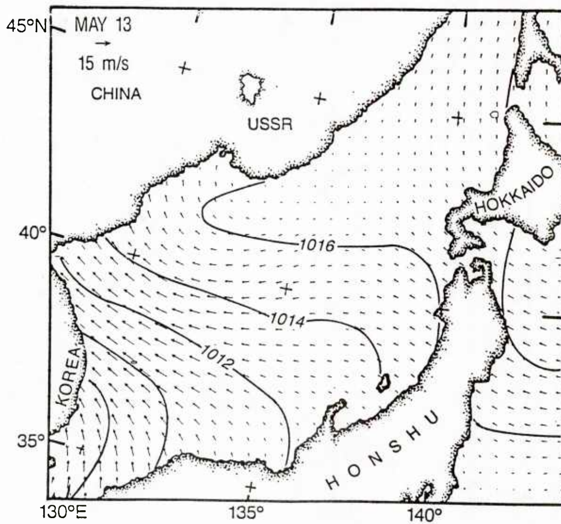
Figure 50b. Wind vectors ( \text{ms}^{-1} ) and sea level pressure (mb) from NOGAPS, May 13, 1984.
