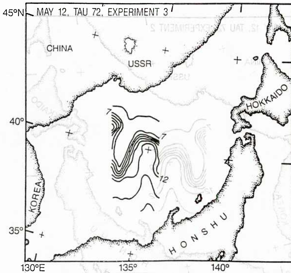
Figure 49c. Forecast SST ( ^{\circ}\text{C} ), experiment 3, May 12, 1984, TAU 72.
