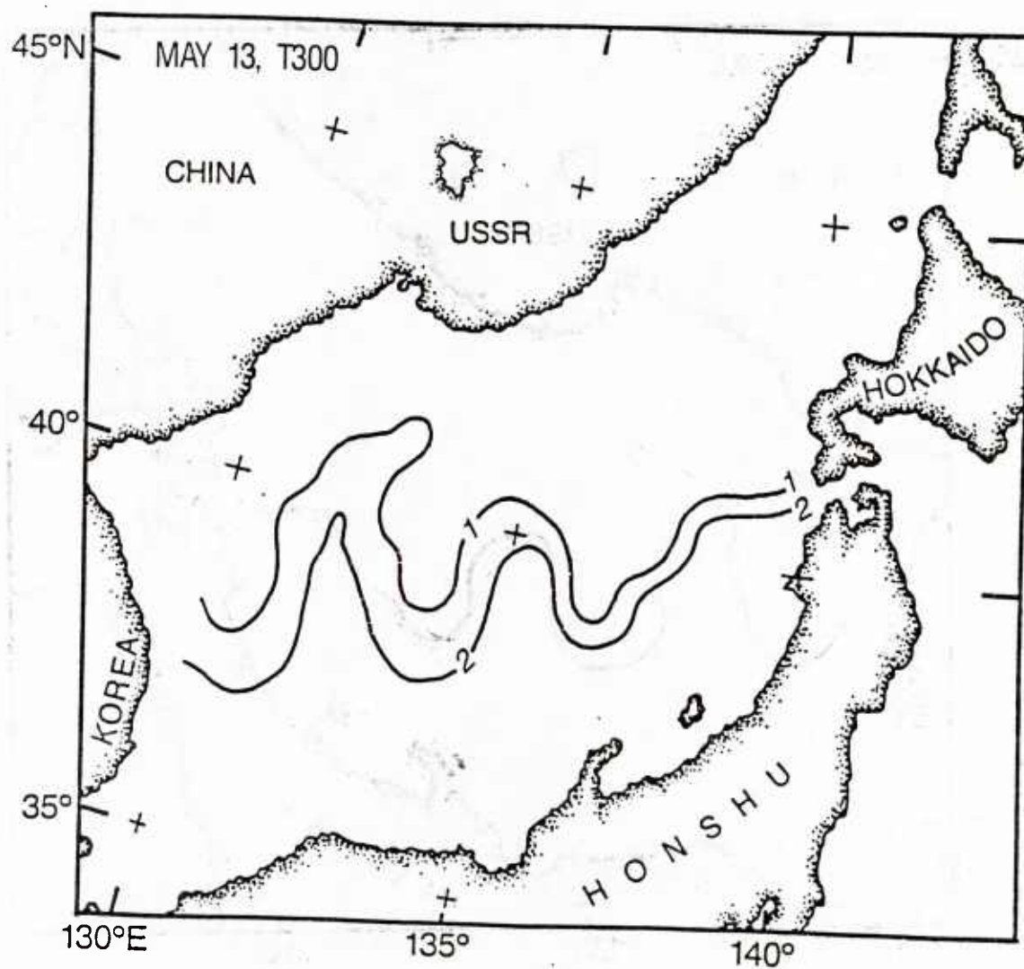
Figure 30. Frontally modified, daily, EOTS temperature ( ^{\circ}\text{C} ) at 300 m for May 13, 1984.
