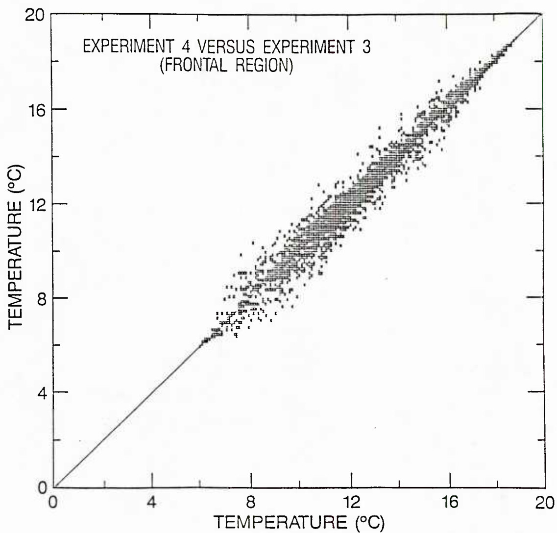
Figure D4b. Scatter plot of TAU 72 SST ( ^{\circ}\text{C} ) forecasts covering May 8 - June 4, 1984, for experiment 4 vs. experiment 3 (frontal region).
