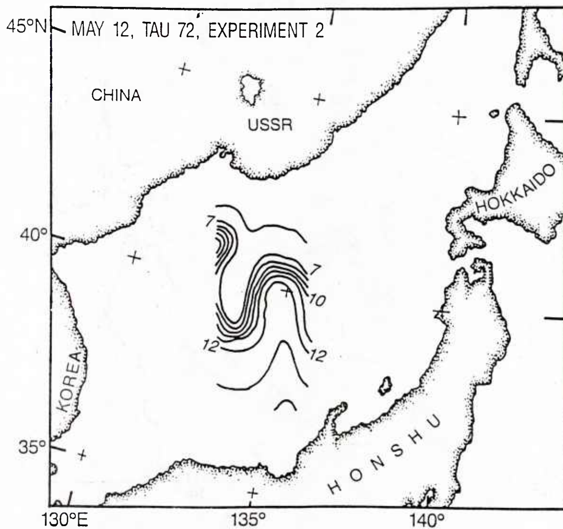
Figure 49b. Forecast SST ( ^{\circ}\text{C} ), experiment 2, May 12, 1984, TAU 72.
