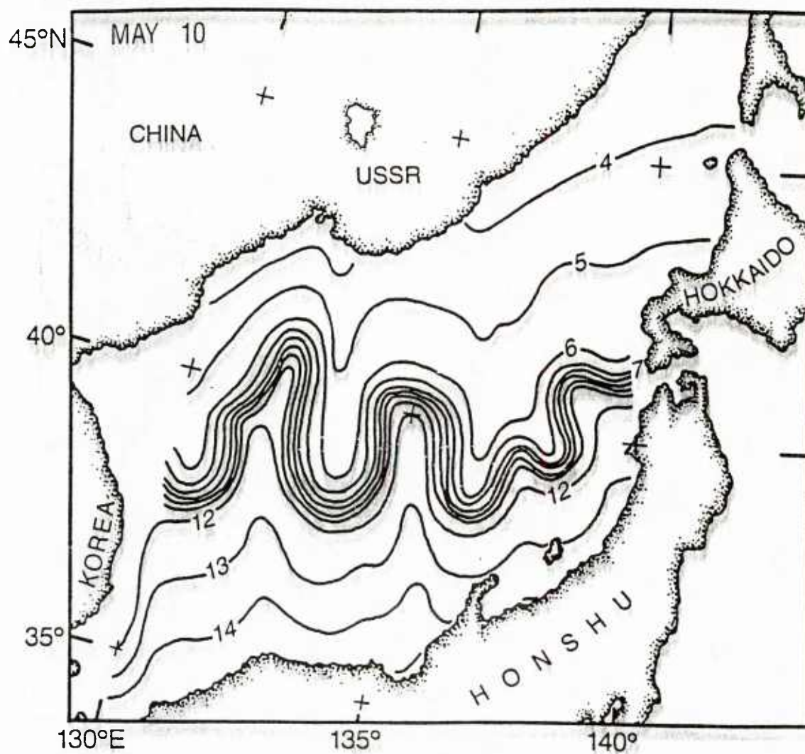
Figure 19. Synthetic SST ( ^{\circ}\text{C} ) field for May 10, 1984.
