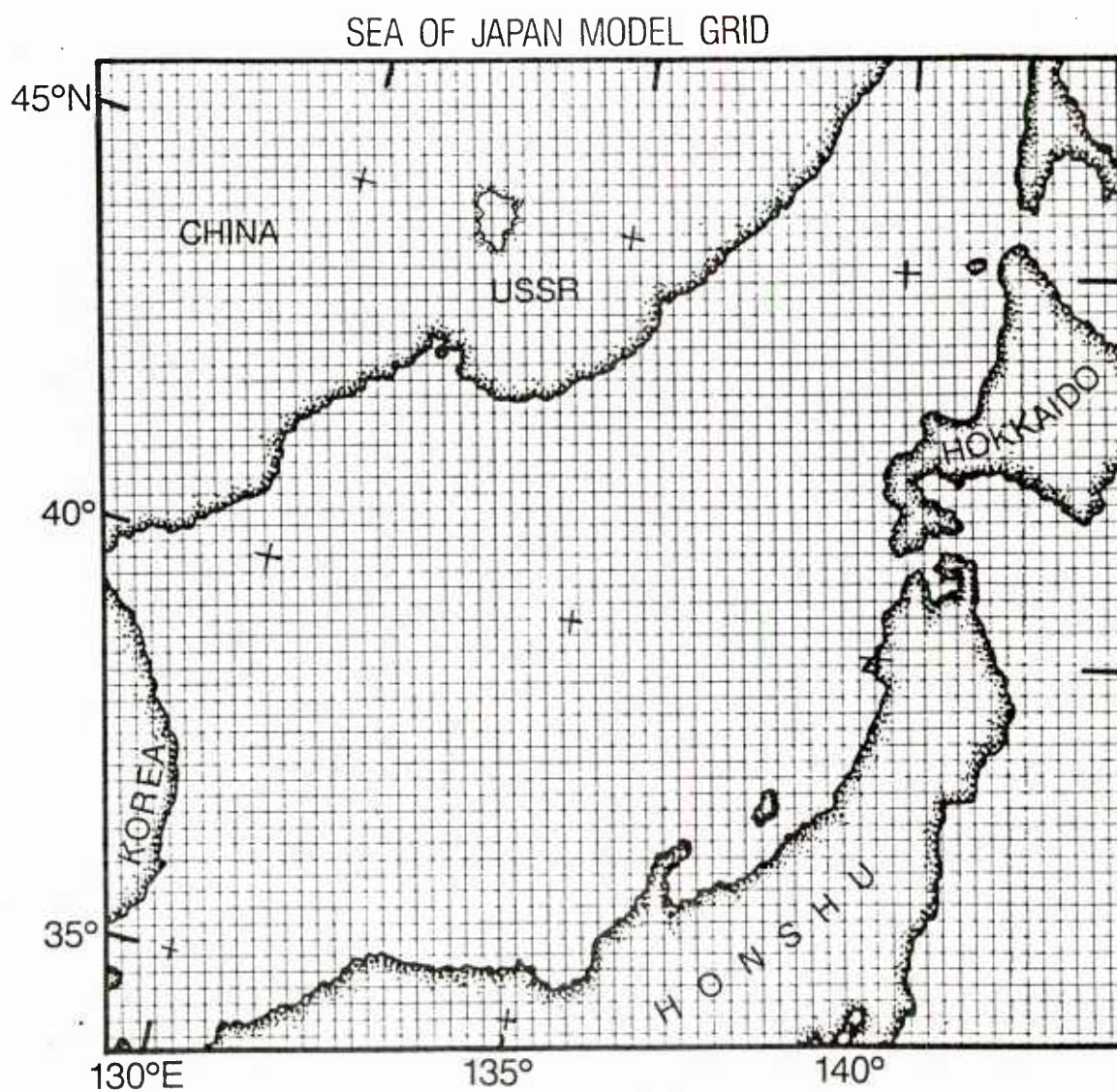
Figure 5. The Sea of Japan model grid.
