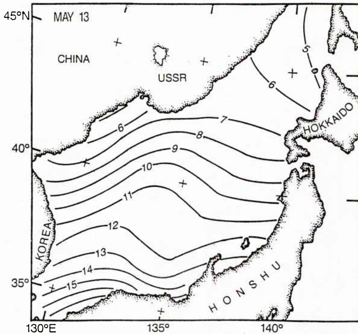
Figure 11. Zoomed EOTS SST ( ^{\circ}\text{C} ) for May 13, 1984.
