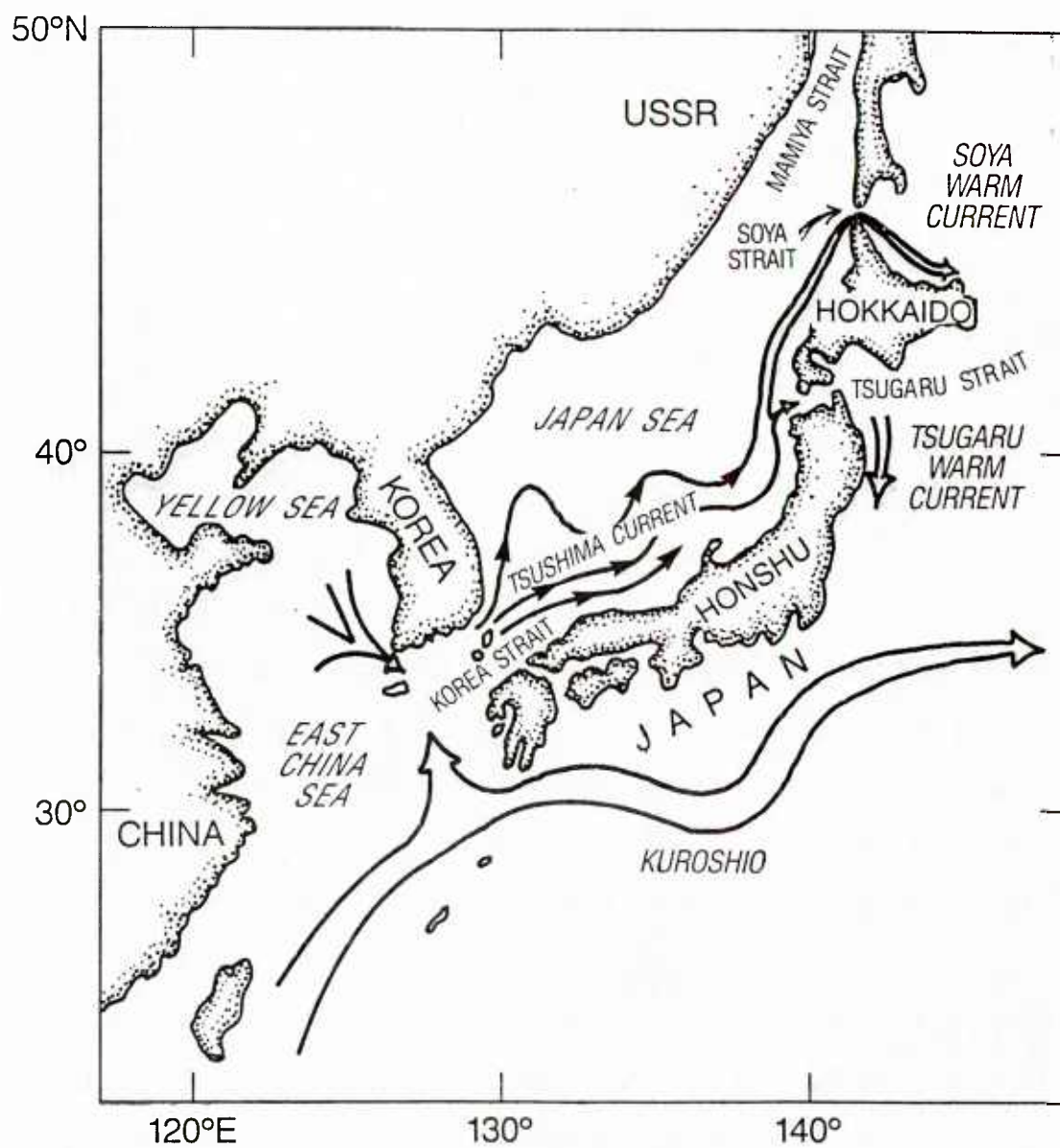
Figure 3. Schematic of flow in the Sea of Japan [adapted from CONLON(1981)].
