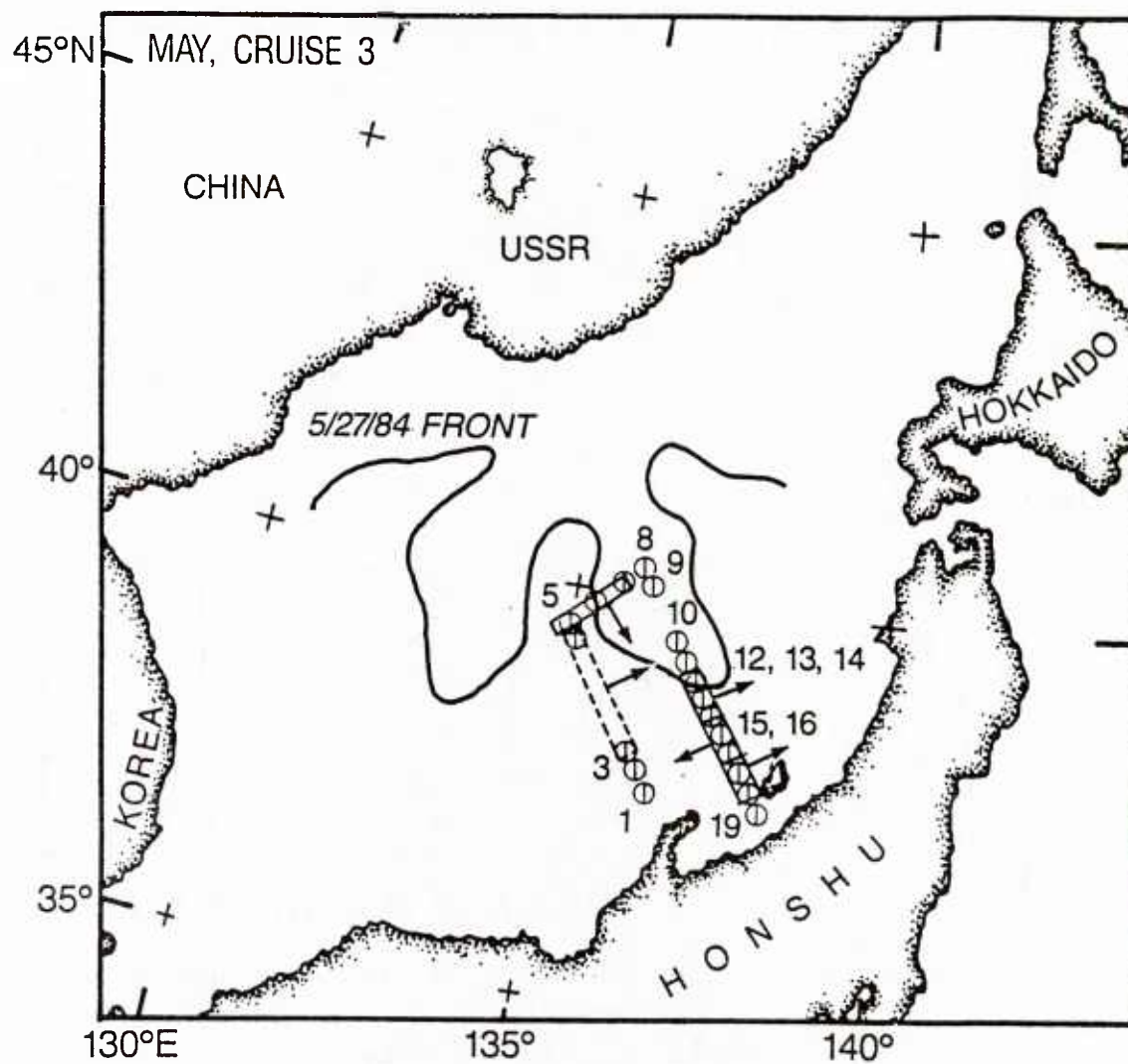
Figure 37. Stations occupied and resultant inferred flow during May 25-27, 1984, cruise of the Seifu Maru . May 27 interpolated frontal location superimposed.
