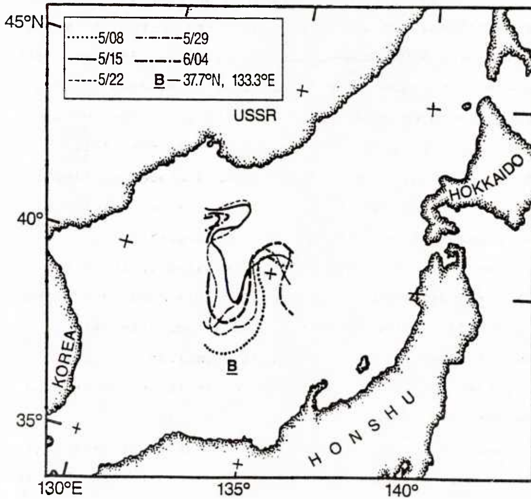
Figure 45. Weekly frontal positions derived from the NOCC Guam subjective SST analyses for May 8 - June 4, 1984. Rectangular area denotes model subregion over which section 7 statistical analyses are performed.
