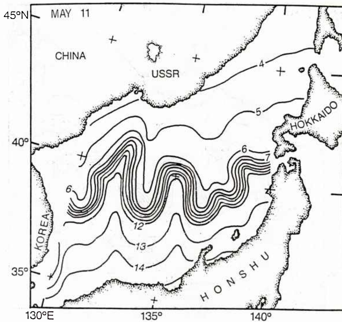
Figure 20. Synthetic SST ( ^{\circ}\text{C} ) field for May 11, 1984.
