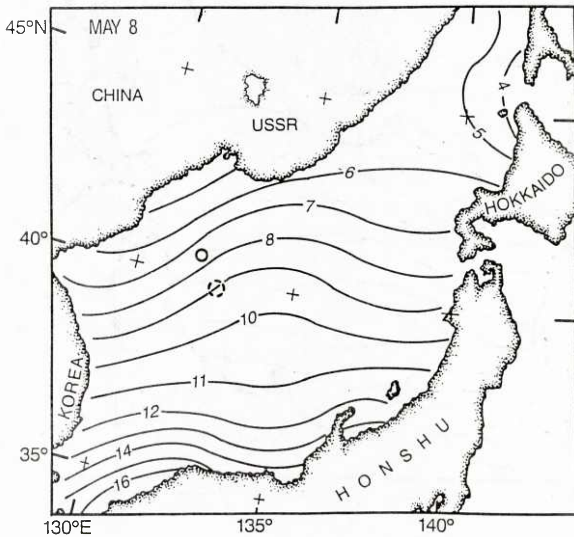
Figure 6. Zoomed EOTS SST ( ^{\circ}\text{C} ) for May 8, 1984.
