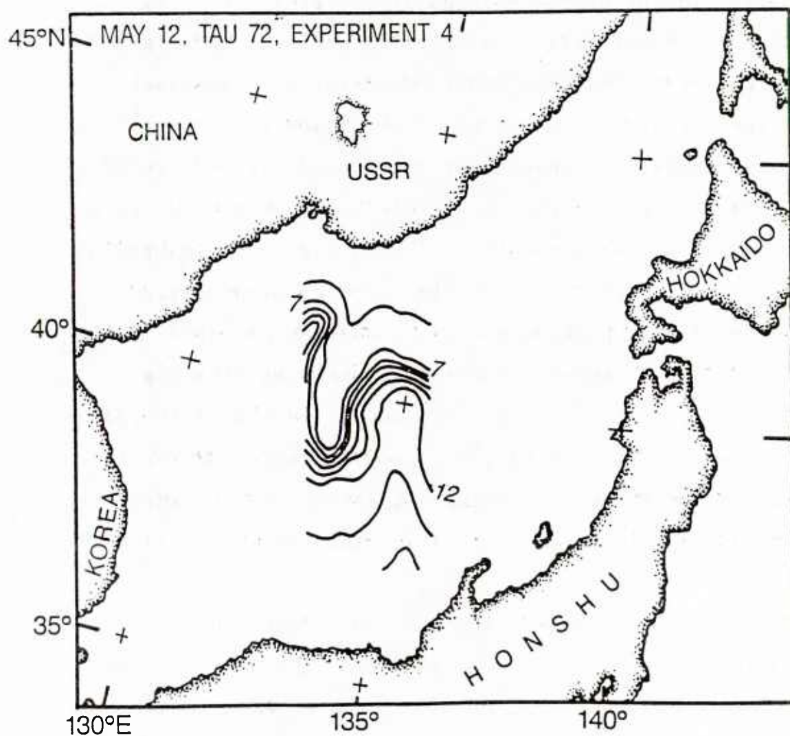
Figure 49d. Forecast SST ( ^{\circ}\text{C} ), experiment 4, May 12, 1984, TAU 72.
