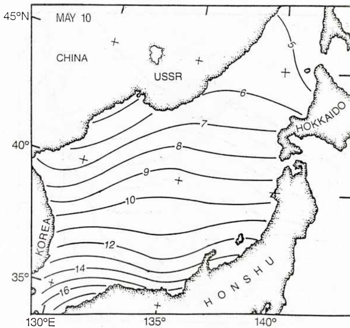
Figure 8. Zoomed EOTS SST ( ^{\circ}\text{C} ) for May 10, 1984.
