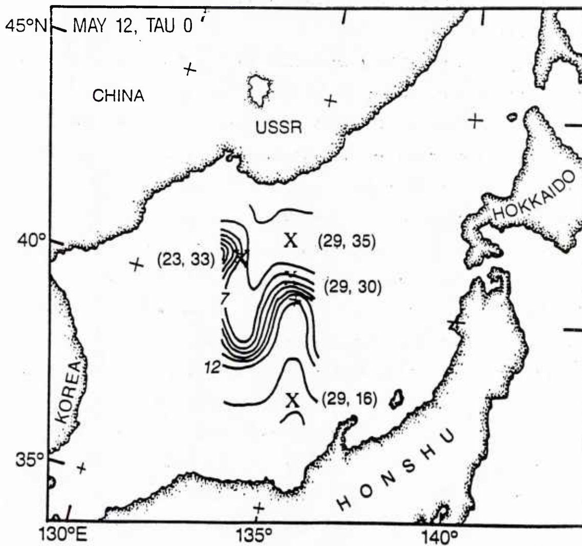
Figure 52. Initial condition SST ( ^{\circ}\text{C} ) for May 12, 1984, forecast identifying four specific grid point locations.
