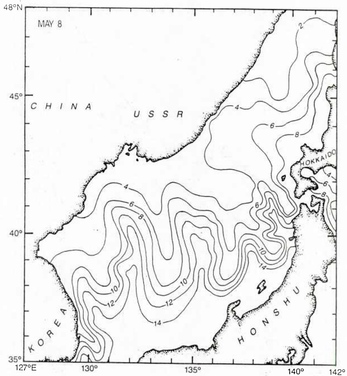
Figure 14. Sea of Japan subset of NOCC Guam weekly Pacific Ocean SST ( ^{\circ}\text{C} ) analysis for May 8, 1984.
