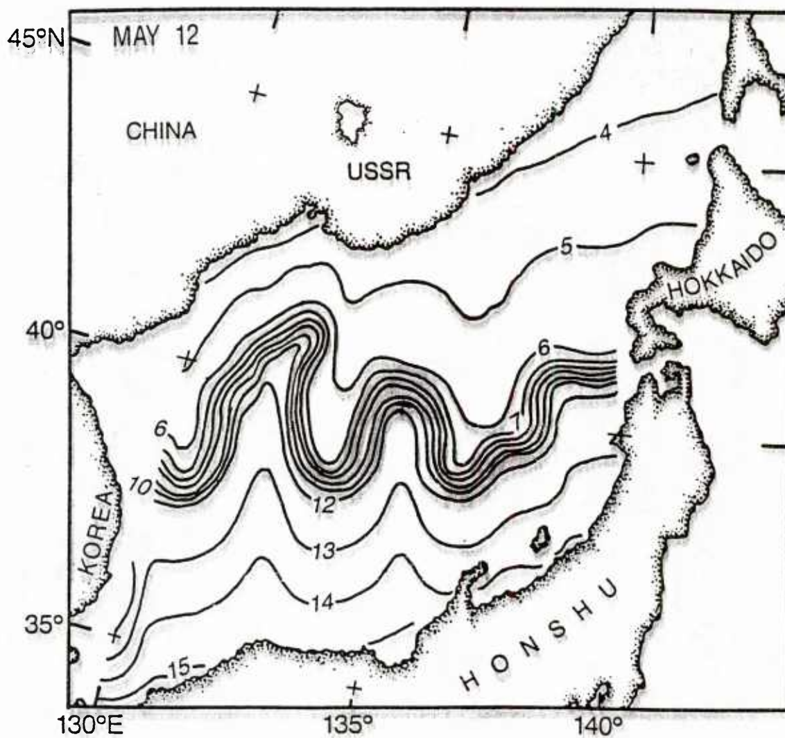
Figure 21. Synthetic SST ( ^{\circ}\text{C} ) field for May 12, 1984.
