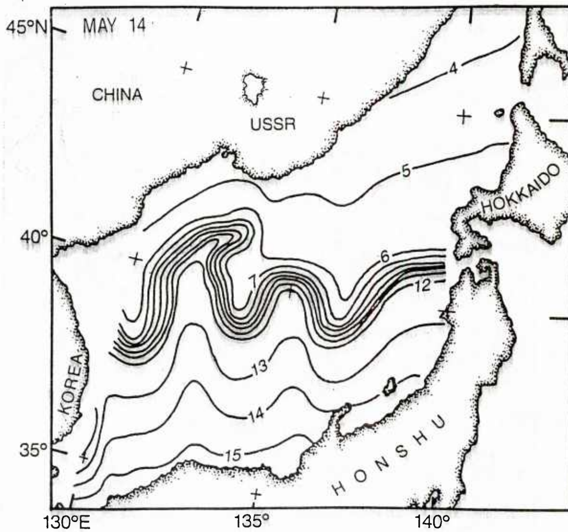
Figure 23. Synthetic SST ( ^{\circ}\text{C} ) field for May 14, 1984.
