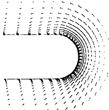
Fig. 8 Vector plots of transverse velocities (normalized by the free-stream velocity) in the tip region at several streamwise stations
