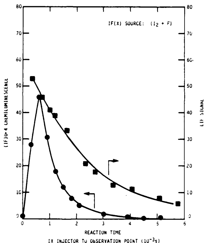
Figure 30. Plot of temporal evolutions of IF^+ and IF(B+X) chemiluminescence intensity. IF(X) produced by I_2 + F reaction. ■ -LIF signal from excitation of IF^+(X; v''=10) ; ● - IF(B+X) chemiluminescence intensity (data are normalized at one point)
