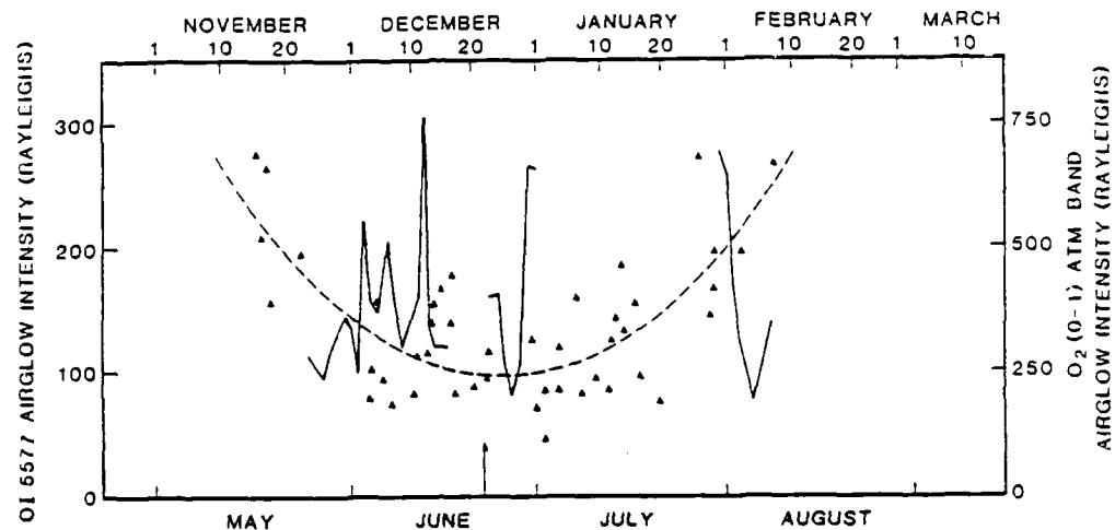
Figure 4 The daily averages of the O_2 (0-1) atm band intensities as obtained from Longyearbyen ( 78^\circ N ) during the 1983/84 season. The intensities of the OI 5577 Å line from Antarctica observations (ISIS 2 data) during winter solstice conditions are also plotted (filled triangles). The dashed line indicates the seasonal trend for the Antarctica data. Antarctica data is from Ismail and Cogger (1982)
