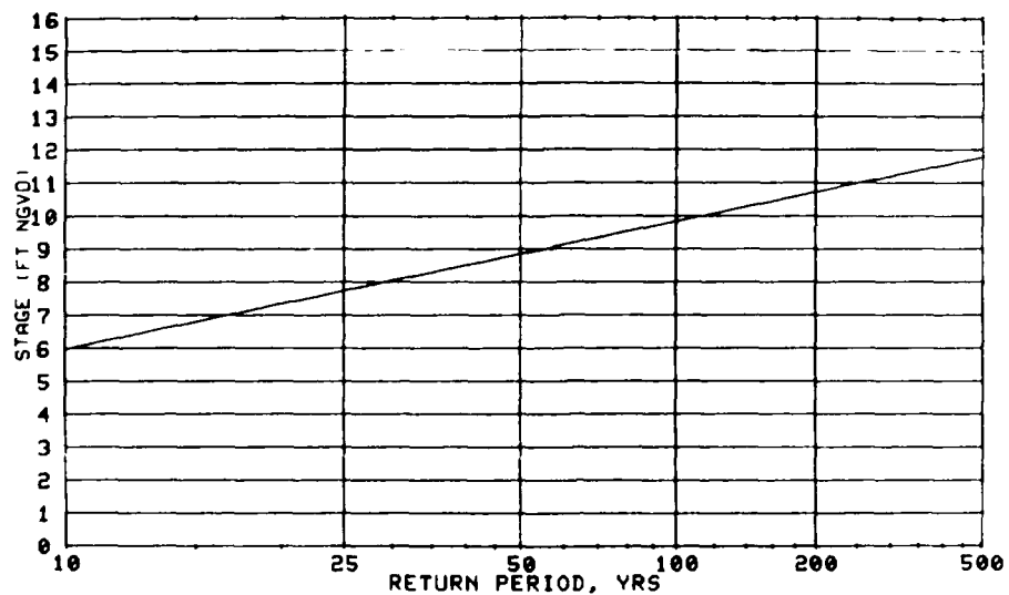
STAGE FREQUENCY STILL WATER LEVEL HURRICANE GAGE 10 (E OF NORMANDIE)
