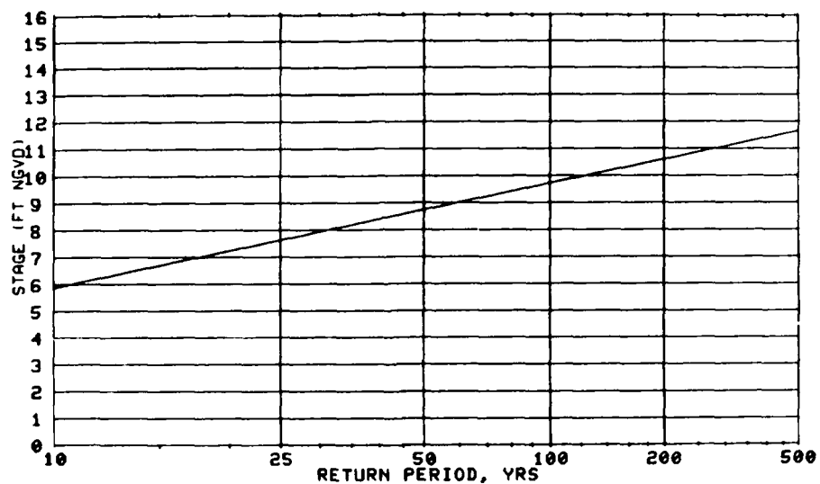
STAGE FREQUENCY STILL WATER LEVEL HURRICANE GAGE 9 (ENTRANCE OF CLAYPIT CREEK)
