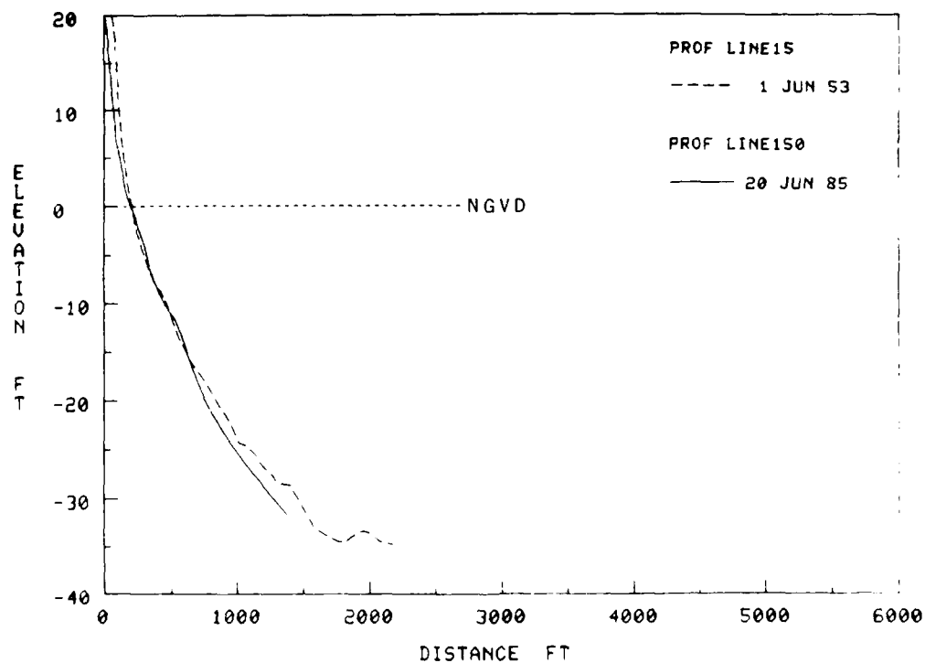
Figure D15. Profile comparisons 1953-1985, lines 14 and 15 (140 and 150)
