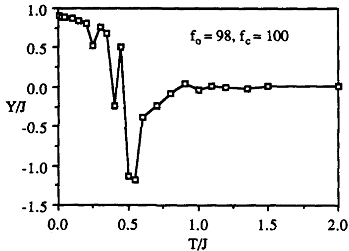
Figure 4.6 An example of pathological behavior in the helicity modulus vs. temperature, for a single realization of a 16 \times 16 sample with f_o = 98 and f_c = 100 .
