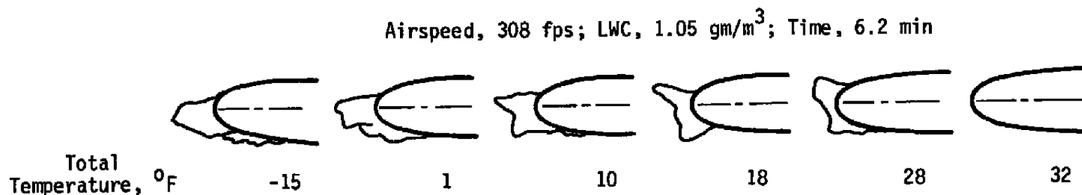
FIGURE 9. EFFECT OF TOTAL TEMPERATURE ON ICE SHAPE; (\text{LWC} \times \text{V} \times \text{TIME}) = \text{CONSTANT} ; MVD, 20 \text{ } \mu\text{M} ; AIRFOIL, NACA 0012 WITH 21-IN. CHORD AT 4-DEG ANGLE OF ATTACK (REF. 3).
