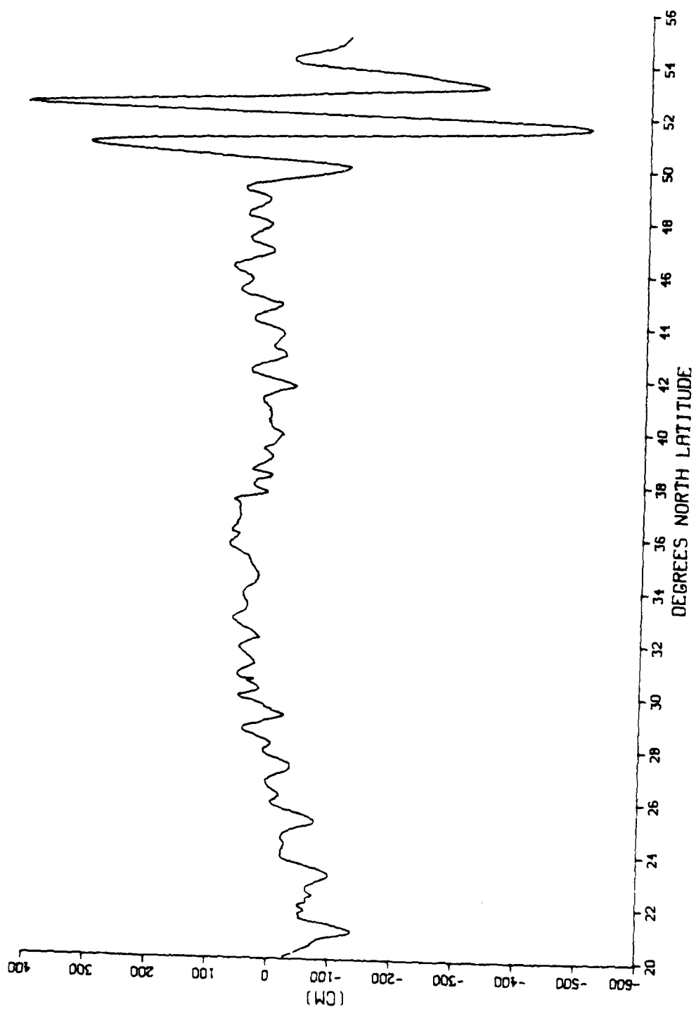
Fig. 2.2 Mean sea surface height profile along arc 209. No corrections applied. The large
