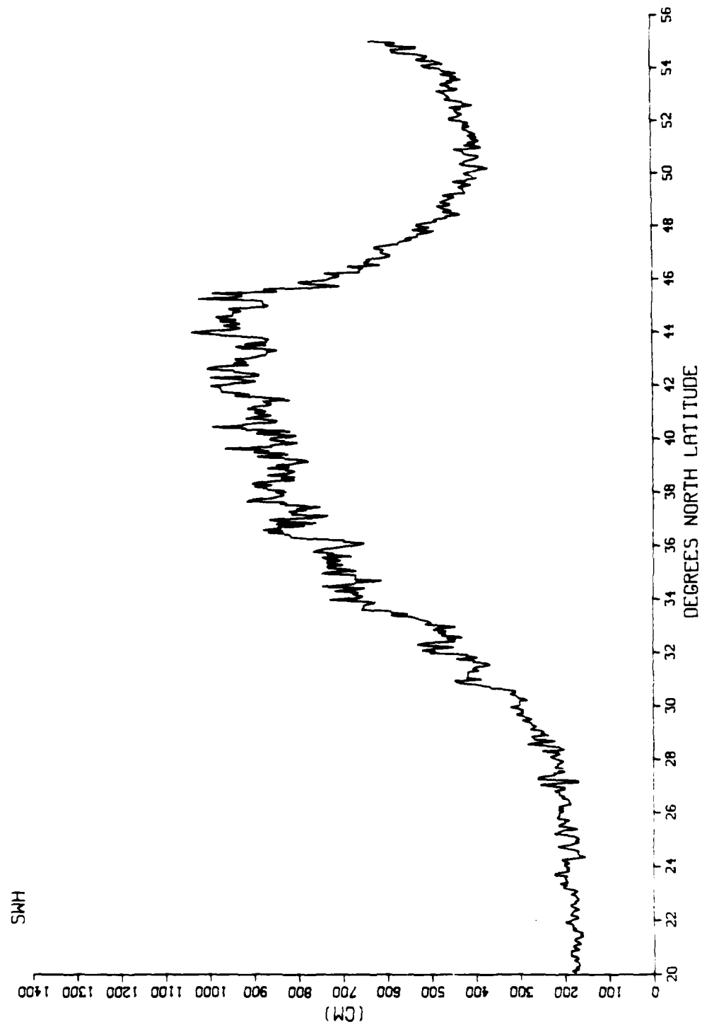
Fig. 1.7 Significant wave height along repeat 4 on arc 82. The electromagnetic bias correction is 2% of the SWH.
