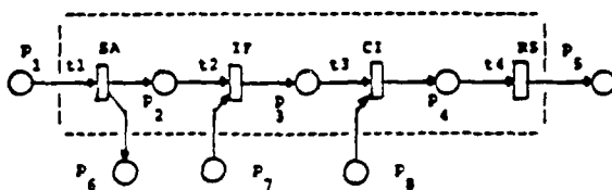
Figure 3: A Single Interacting Decisionmaker
