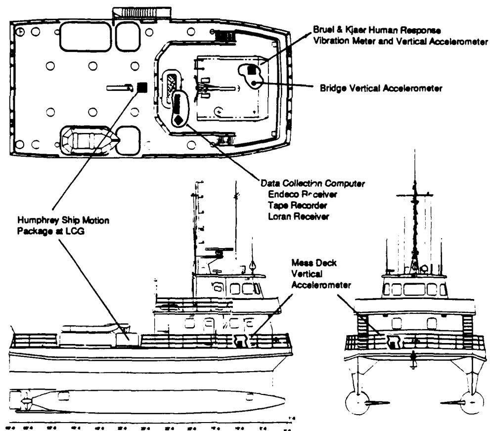
FIGURE 6. Sensor Locations (from Reference 6)
