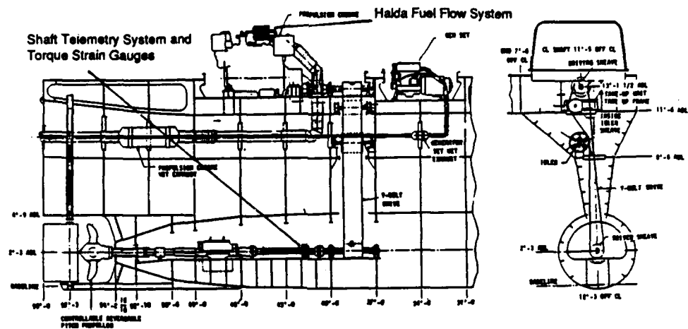
FIGURE 5. Machinery Arrangement and Shaft HP Measurement (from reference 6)
