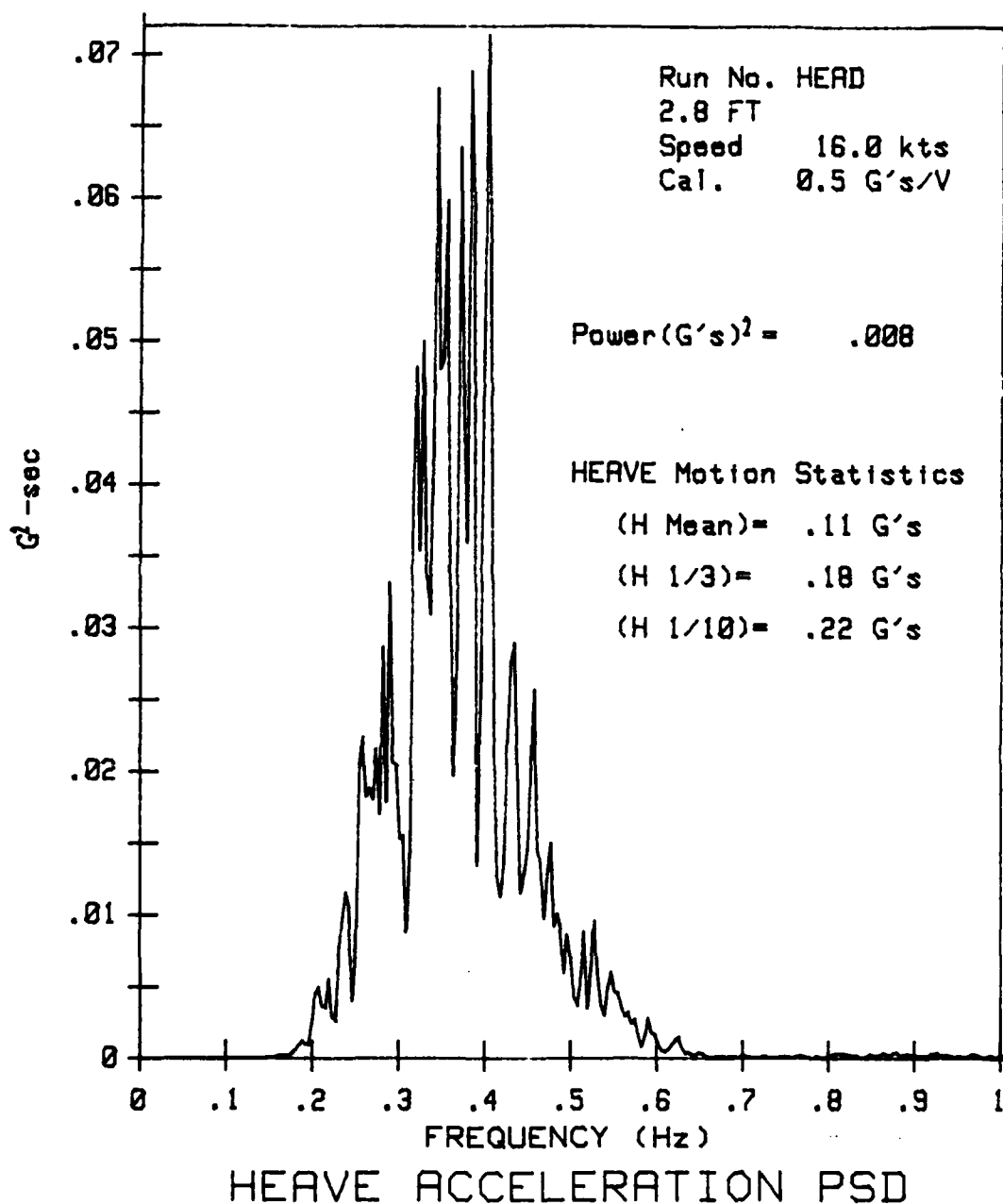
FIGURE C-28. PT KNOLL Heave PSD Plot, 2.8 Ft Head Seas
