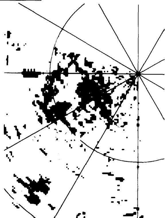
Figure VI-8. Radial velocity fields from pencil beam weather radar and ASR during microburst at 20:34 (UT), 1 August 1987. Range rings are at 10 km intervals.
