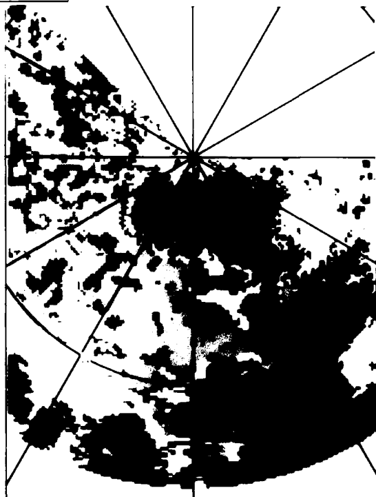
Figure V/1-6. Radial velocity fields from pencil beam weather radar and ASR during microburst at 20:46 (UT), 21 June 1987. Range ring is at 10 km.
