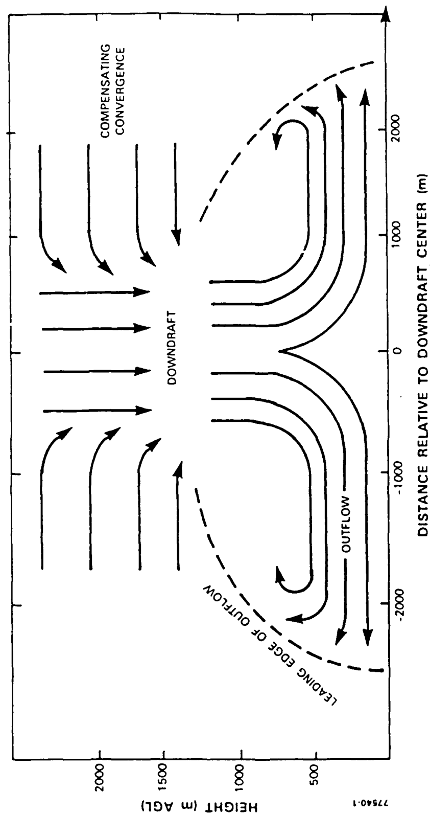
Figure I-1(a) Vertical cross section of microburst wind field.
