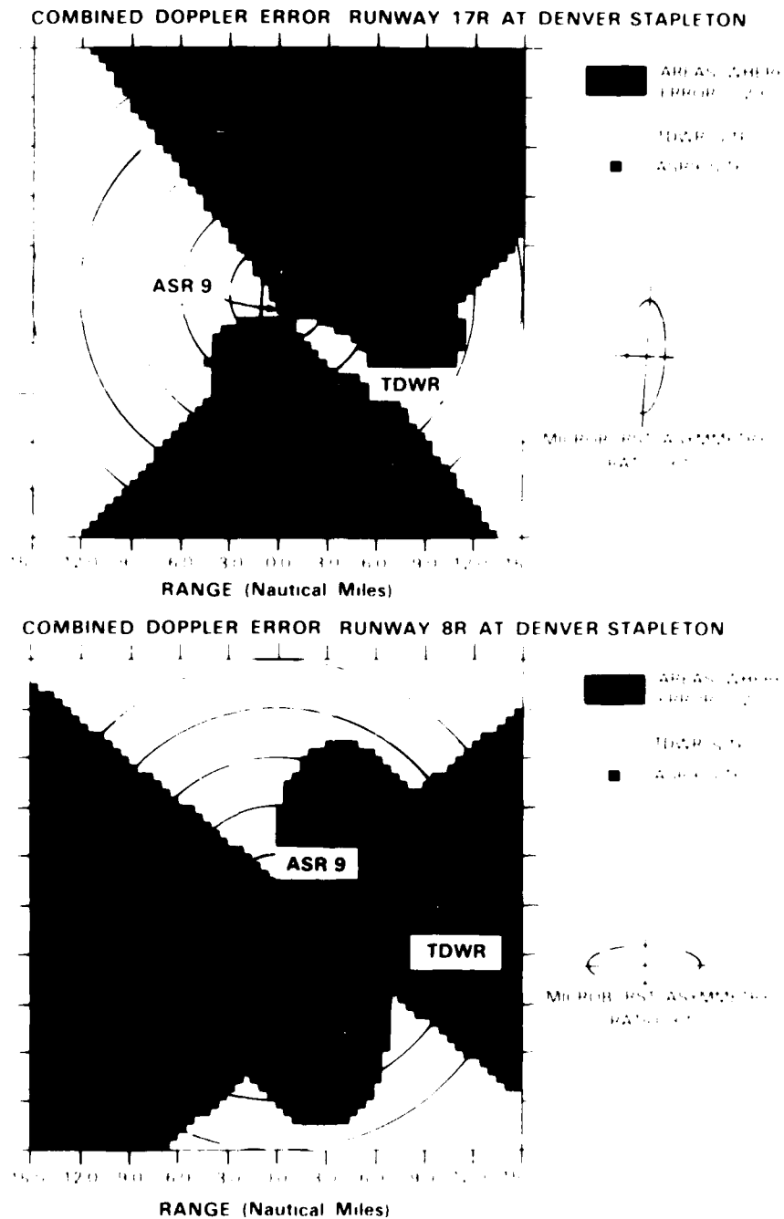
Figure A-3. Areas at Denver-Stapleton Airport where combined TDWR and ASR measurements of headwind-tailwind shear along runway directions would be within 20 percent of true shear under severe microburst asymmetry conditions.
