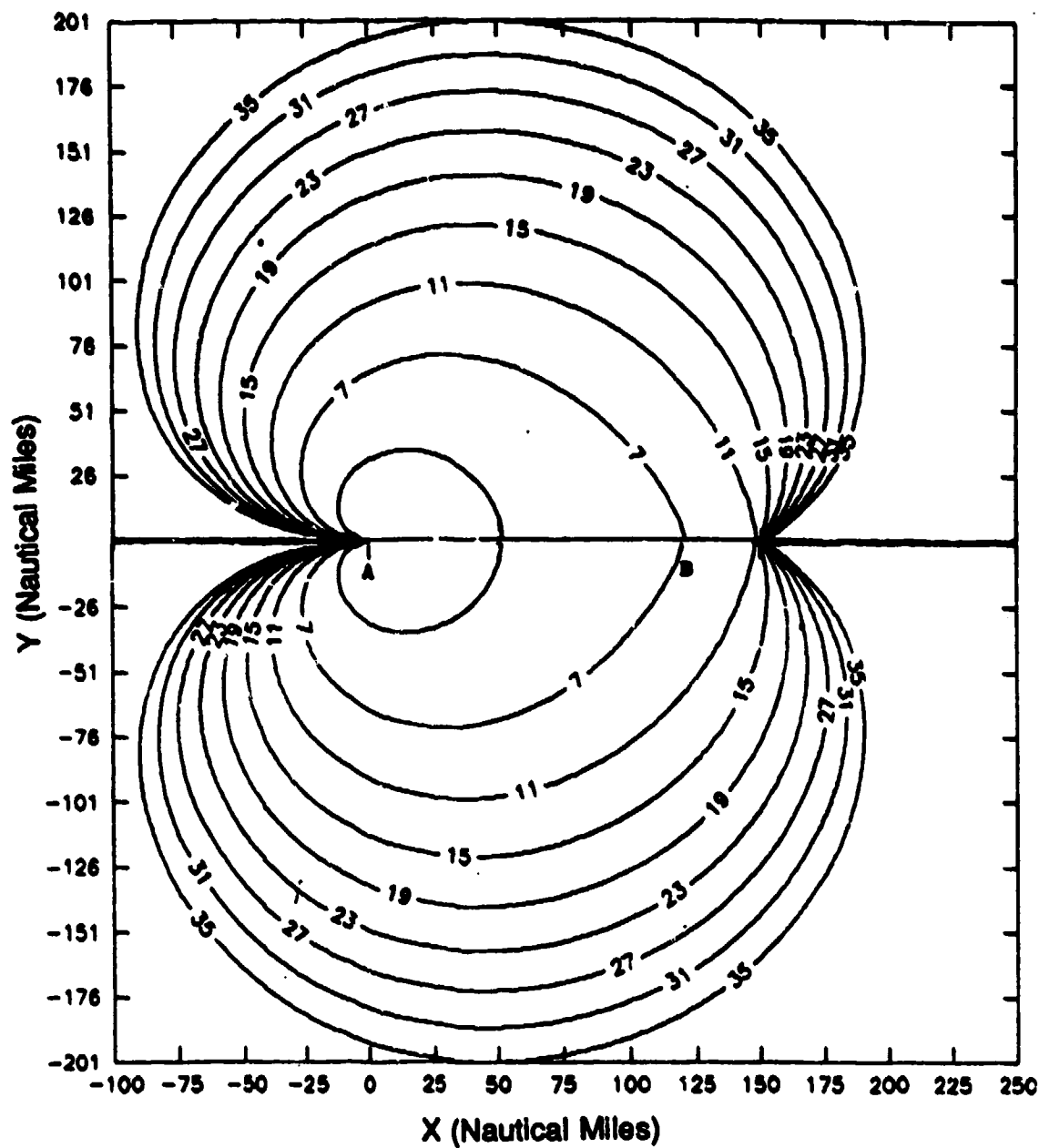
Figure 7. Case 2: CEP Contours for One Bearing Angle and a TD0A (Hyperbola)
