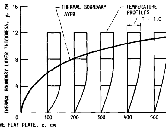
FIGURE 9. - EXPONENTIAL FINITE DIFFERENCE RESULTS FOR BOUNDARY LAYER EQUATIONS WITH CONDITIONS U(0, y) = 1.0 , U(x, 0) = 0 , V(x, 0) = 0 , V(x, L) = 0 , T(x, 0) = 0.0 , T(0, y) = 1.0 ; \nu = 0.0072 \text{ cm}^2/\text{s} ; \alpha = 0.01 \text{ cm}^2/\text{s} .
