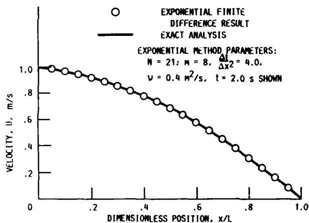
FIGURE 5. - COMPARISON OF STEADY STATE SOLUTIONS COMPARING THE EXACT RESULTS TO THE EXPONENTIAL FINITE DIFFERENCE SOLUTION U(0, t) = 1.0 ; U(L, t) = 0.0 .
