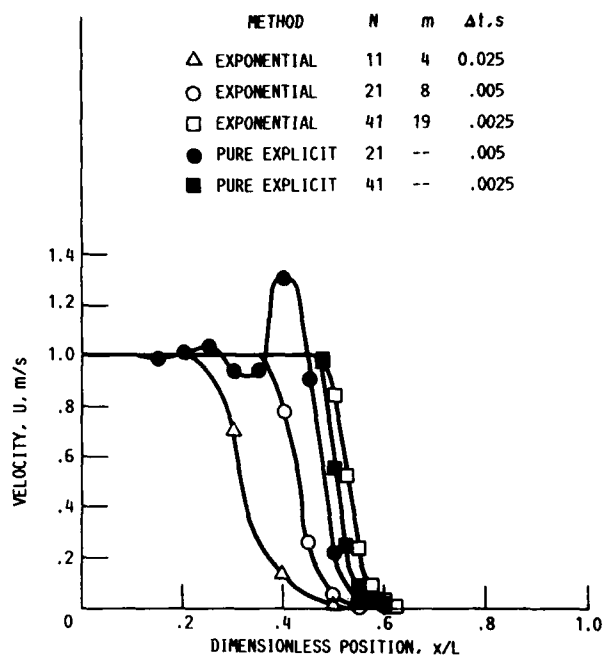
FIGURE 7. - COMPARISON OF EXPONENTIAL AND PURE EXPLICIT FINITE DIFFERENCE METHODS. ALL RESULTS SHOWN FOR \nu = 0.01 \text{ m}^2/\text{s} , t = 1.0 \text{ s} , U(0, t) = 1.0 , AND U(L, t) = 0.0 .
