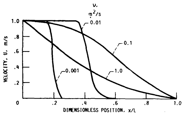
FIGURE 6. - EXPONENTIAL FINITE DIFFERENCE RESULTS FOR VARYING KINEMATIC VISCOSITY. ALL VELOCITIES ARE SHOWN FOR M = 21 , m = 8 , \Delta t / \Delta x^2 = 4.0 , t = 1.0 s, U(0, t) = 1.0 , U(L, t) = 0.0 .
