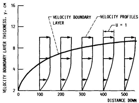
FIGURE 9. - EXPONENTIAL FINITE DIFFERENCE RESULTS FOR BOUNDARY LAYER EQUATIONS WITH CONDITIONS U(0, y) = 1.0 , U(x, 0) = 0 , V(x, 0) = 0 , V(x, L) = 0 , T(x, 0) = 0.0 , T(0, y) = 1.0 ; \nu = 0.0072 \text{ cm}^2/\text{s} ; \alpha = 0.01 \text{ cm}^2/\text{s} .
