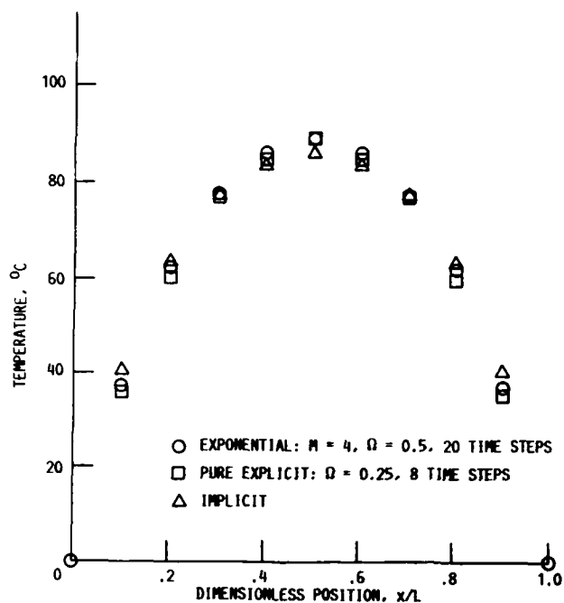
FIGURE 3. - COMPARISON OF METHODS FOR TEMPERATURE-VARYING CONDUCTIVITY, SHOWING TEMPERATURE FIELD AT t = 0.02 s. k(T) = k_R(1 + \beta T) WHERE k_R = 1.0 , \beta = 0.01 , T(x, 0) = 100 , AND T(0, t) = T(L, t) = 0 ; \alpha = 1 .
