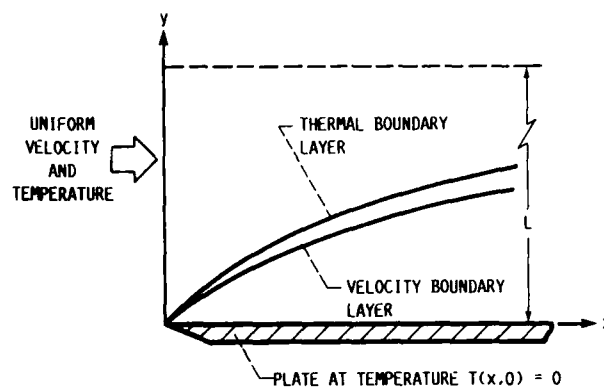
FIGURE 8. - BOUNDARY LAYER DEVELOPMENT ALONG A COOLED FLAT PLATE. CONDITIONS: U(x, 0) = 0 , V(x, 0) = 0 , V(x, L) = 0 , U(0, y) = 1.0 , T(0, y) = 1.0 .
