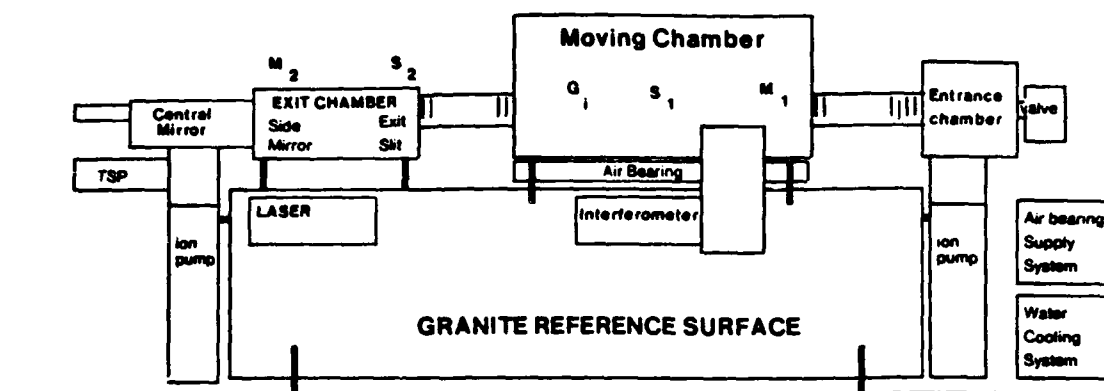
Fig 11 Schematic side view of the Locust Monochromator showing the major assemblies. The details are given in the text. A perspective view of the Moving Chamber is shown in figure 12. The exit chamber contains the exit slit and the refocusing mirrors.
