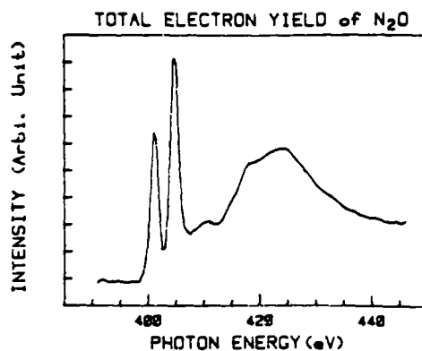
Fig. 7. Total ion yield of N 2 O as a function of photon energy around the nitrogen absorption threshold. The bound state transitions for the terminal nitrogen atom (N T ) and central nitrogen atom (N C ) are observed at 401 eV and 405 eV and marked accordingly.
