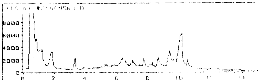
Figure 4. Total Ion Chromatogram from RDX + K_2B_{12}H_{12} Decomposed 20 sec at 400°C
