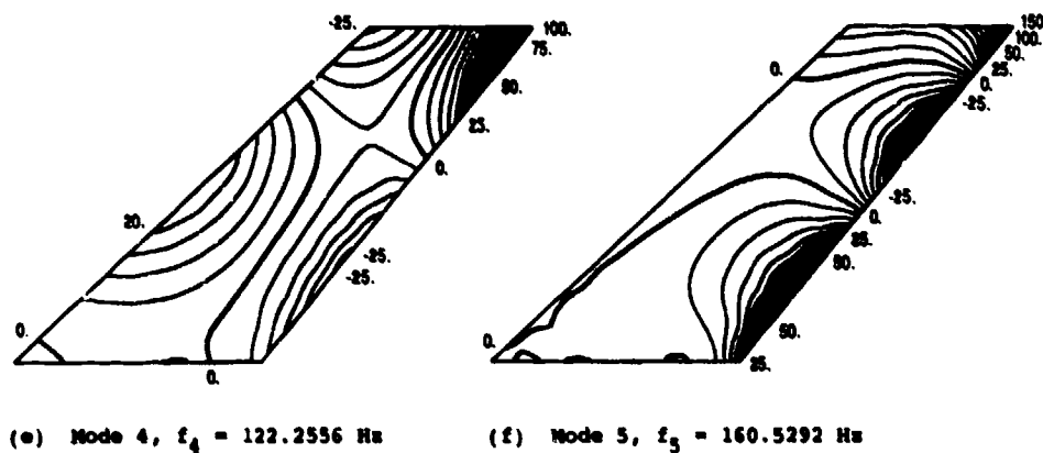
Figure 1.- Joint locations and contours of calculated modal deflections for 2.5-foot solid model 2. Contour interval is 5.00.
