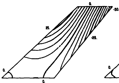
(c) Node 2, f_2 = 38.1650 Hz
