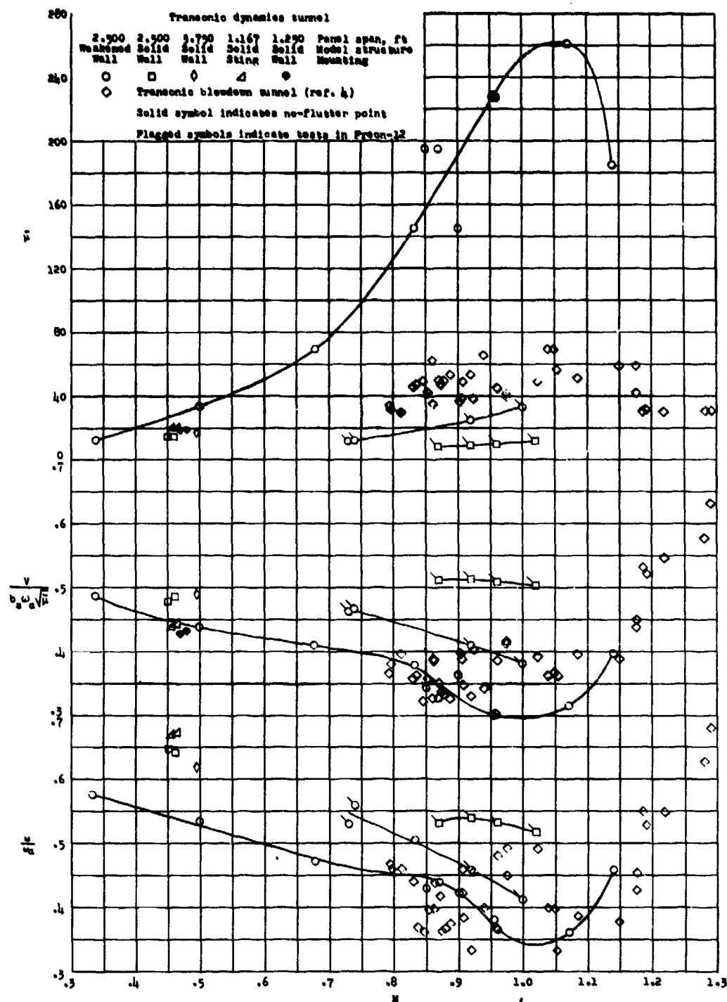
Figure 22.- Comparison of flutter characteristics measured in the transonic dynamics tunnel and in the transonic blowdown tunnel.
