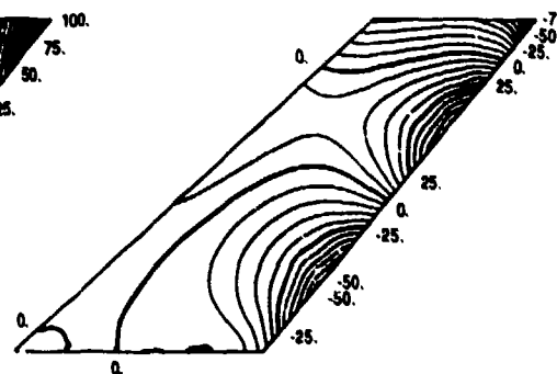
(f) Node 5, f_5 = 118.113 Hz
