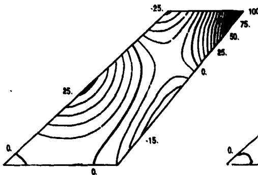
(e) Node 4, f_4 = 91.5448 Hz
