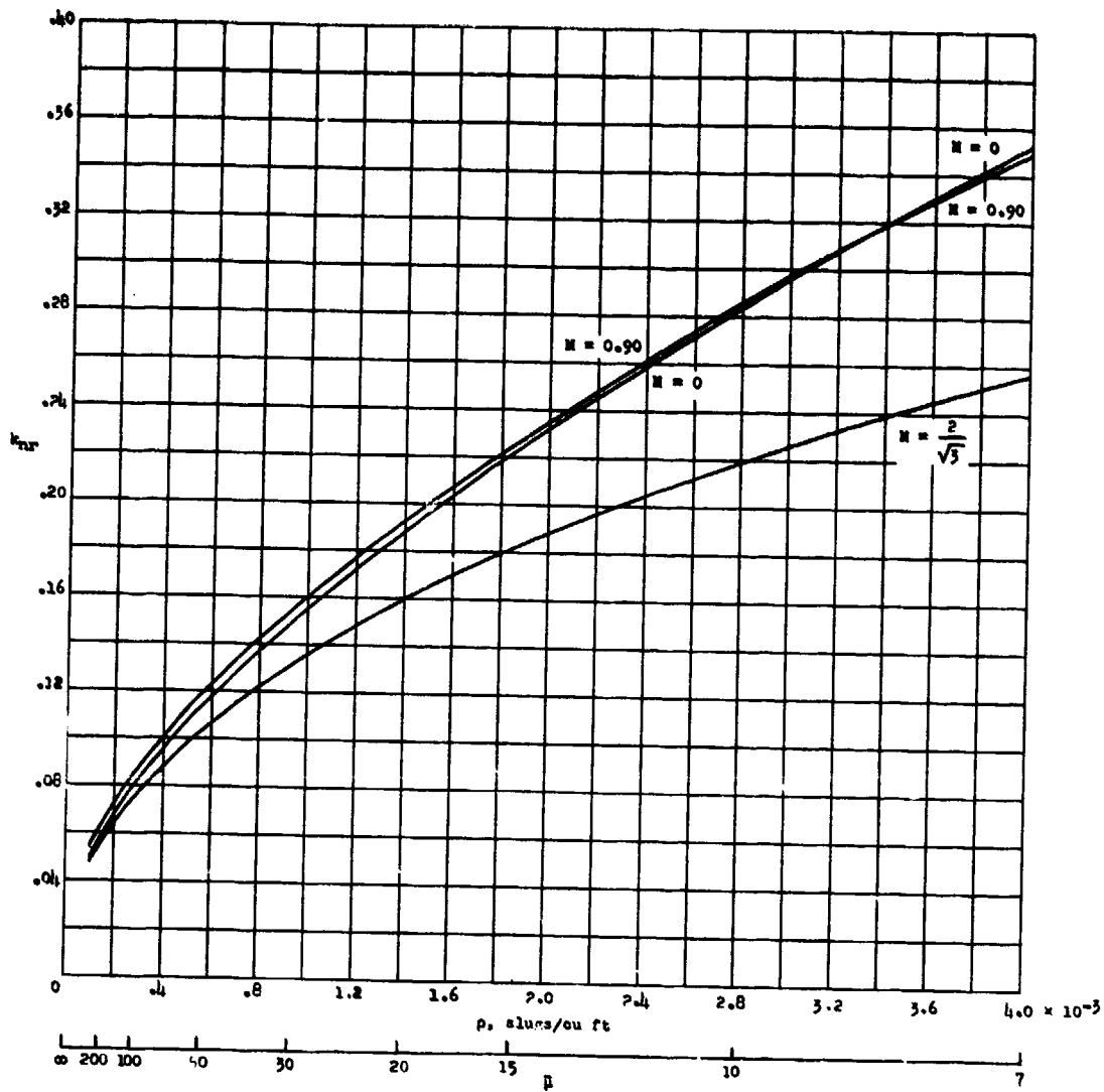
Figure 21.- Effect of density (or mass ratio) on the flutter reduced frequency calculated for weakened 2,500-foot wall-mounted wings in air.
