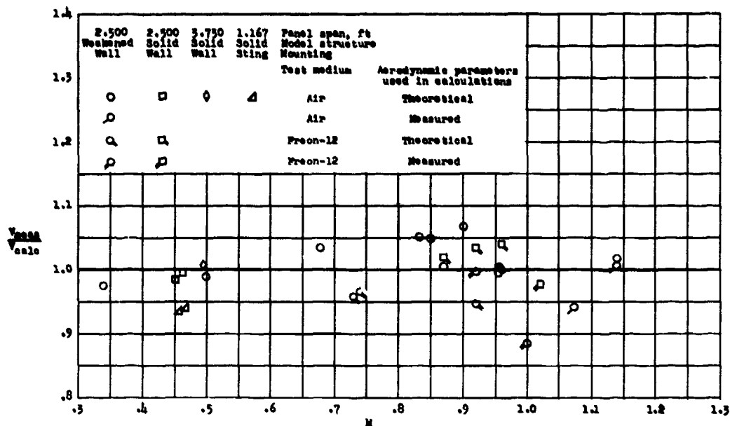
(a) Flutter speeds.
