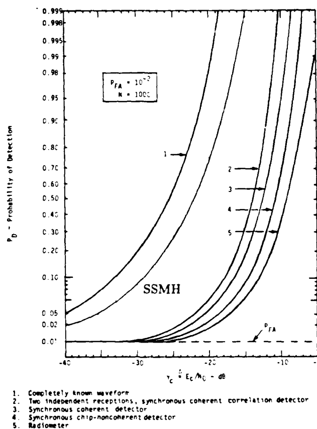
Figure 10.6: DS/BPSK Detectability
