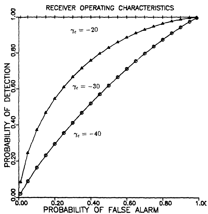
Figure 9.6: Conventional \frac{1}{2} , \frac{5}{8} Code SSMH Receiver Operating Characteristics
