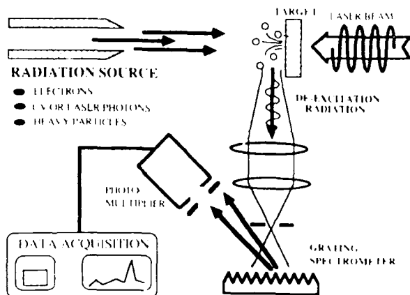
Fig. 1. Schematic of electron- and photon-stimulated desorption experiments using optical spectroscopy to identify desorbing neutral ground- and excited-state alkali atoms
