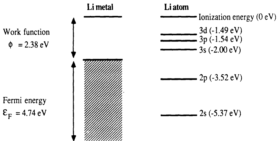
Fig. 5. Schematic energy level diagram of a lithium atom near lithium metal.
