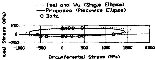
(Note: 1 MPa = 0.145 Ksi) Fig. 7. Correlations of the Quadratic Strength Tensor Theories with the Biaxial Fracture Data of a Unidirectional Glass Epoxy Laminate. 16
