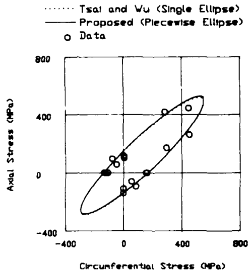
(Note: 1 MPa = 0.145 Ksi) Fig. 10. Correlations of the Quadratic Strength Tensor Theories with the Biaxial Fracture Data of a Helically Wound Glass Epoxy Laminate. 17
