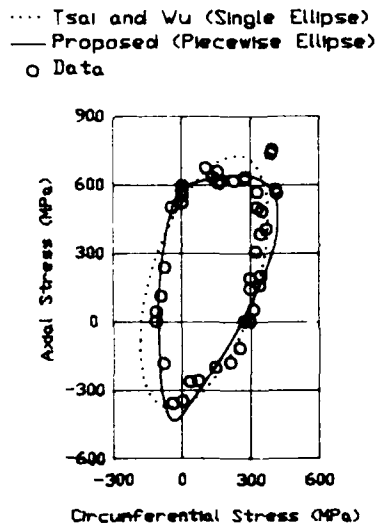
(Note: 1 MPa = 0.145 Ksi) Fig. 8. Correlations of the Quadratic Strength Tensor Theories with the Biaxial Fracture Data of a [90 \pm 30 90] Glass Epoxy Laminate. 16
