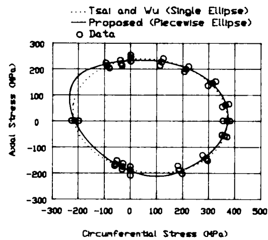
Fig. 6 Correlations of the Quadratic Strength Tensor Theories with the Biaxial Fracture Data of a Finen-Weave Glass-Reinforced Plastic 15
