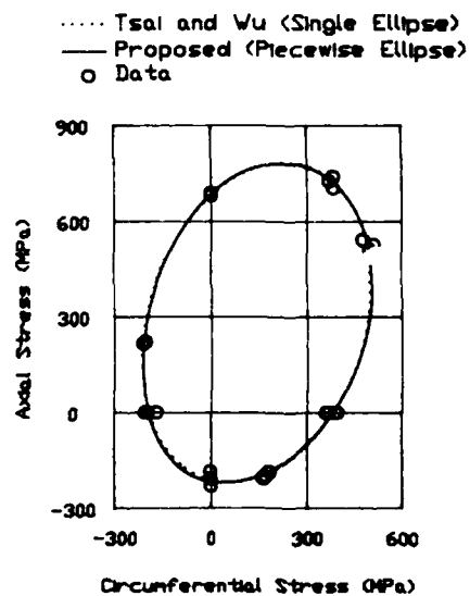
(Note: 1 MPa = 0.145 Ksi) Fig. 11. Correlations of the Quadratic Strength Tensor Theories with the Biaxial Fracture Data of an Organic Textolite. 18
