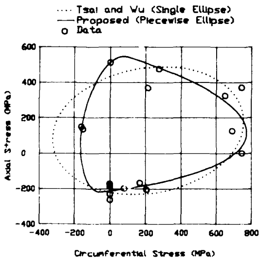
(Note: 1 MPa = 0.145 Ksi) Fig. 9. Correlations of the Quadratic Strength Tensor Theories with the Biaxial Fracture Data of a Cross-Ply Glass Epoxy Laminate. 17
