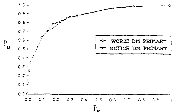
FIGURE 7 TEAM ROC CURVES
