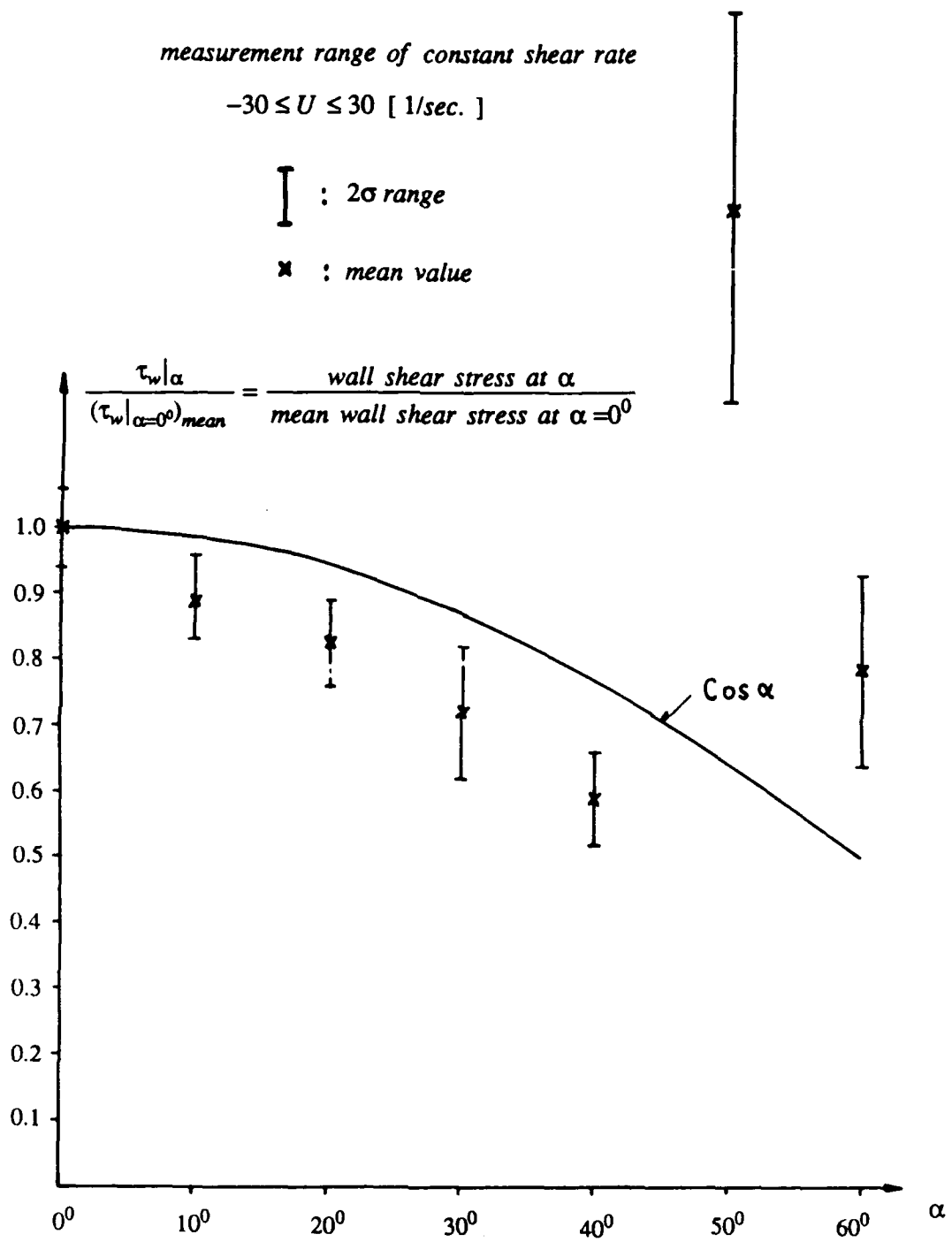
Figure (20). Directivity curve
