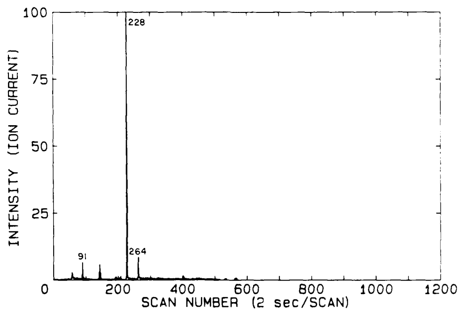
FIGURE 17: RIC showing the compounds released from Derakane 510A resin after heating for 7 minutes at 300°C in a reactive atmosphere.
