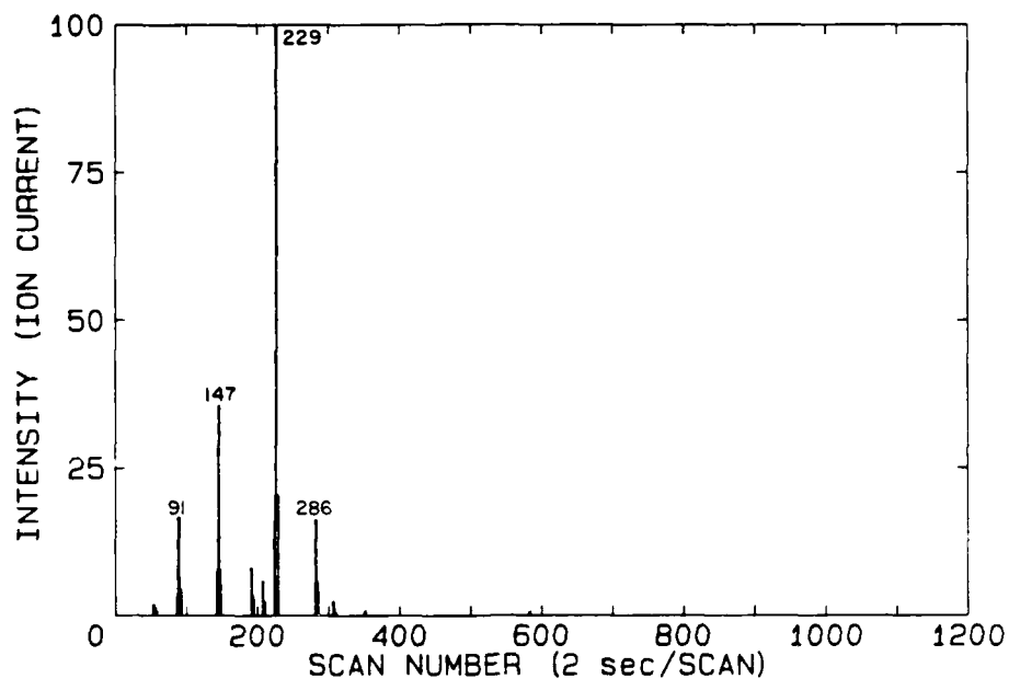
FIGURE 6: RIC showing the compounds released from Derakane 510A resin after heating for 7 minutes at 400 C in an inert atmosphere.
