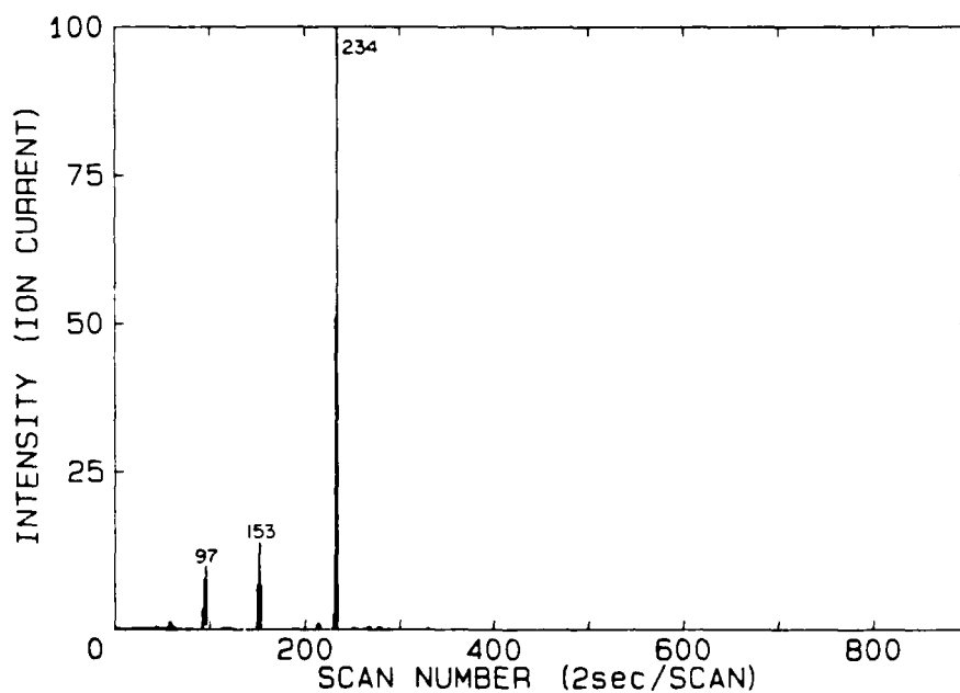
FIGURE 21: RIC showing the compounds released from Vibrin F1029 resin after heating for 7 minutes at 400°C in a reactive atmosphere.
