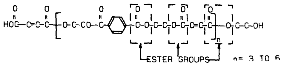
FIGURE 3: Structure of a typical isophthalic acid polyester.
