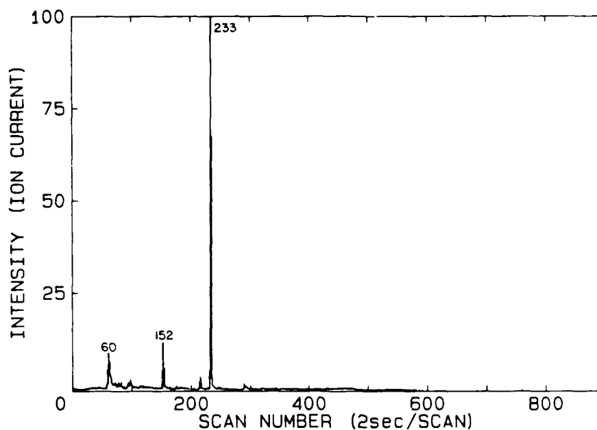
FIGURE 20: RIC showing the compounds released from Vibrin F1029 resin after heating for 7 minutes at 300°C in a reactive atmosphere.
