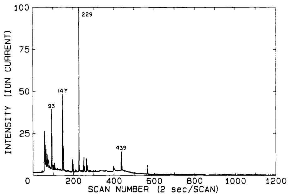
FIGURE 23: RIC showing the compounds released from Hetron 197AT resin after heating for 7 minutes at 300°C in a reactive atmosphere.
