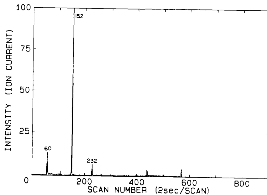
FIGURE 19: RIC showing the compounds released from Vibrin F1029 resin after heating for 7 minutes at 200°C in a reactive atmosphere.
