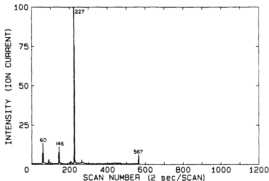
FIGURE 4: RIC showing the compounds released from Derakane 510A resin after heating for 7 minutes at 200 C in an inert atmosphere.
