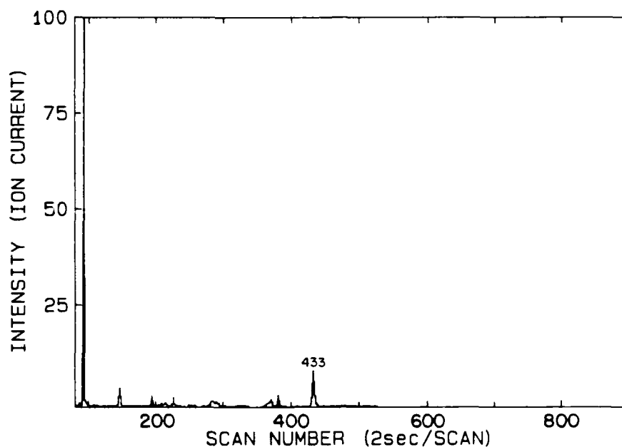
FIGURE 30: RIC showing the compounds released from the polyester portion of Vibrin F1029 resin after heating at 400°C for 10 minutes in an inert atmosphere.
