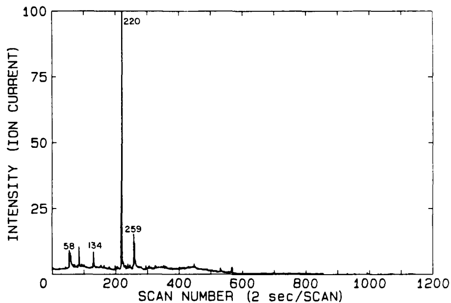
FIGURE 26: RIC showing the compounds released from Hetron 99P resin after heating for 7 minutes at 300°C in a reactive atmosphere.
