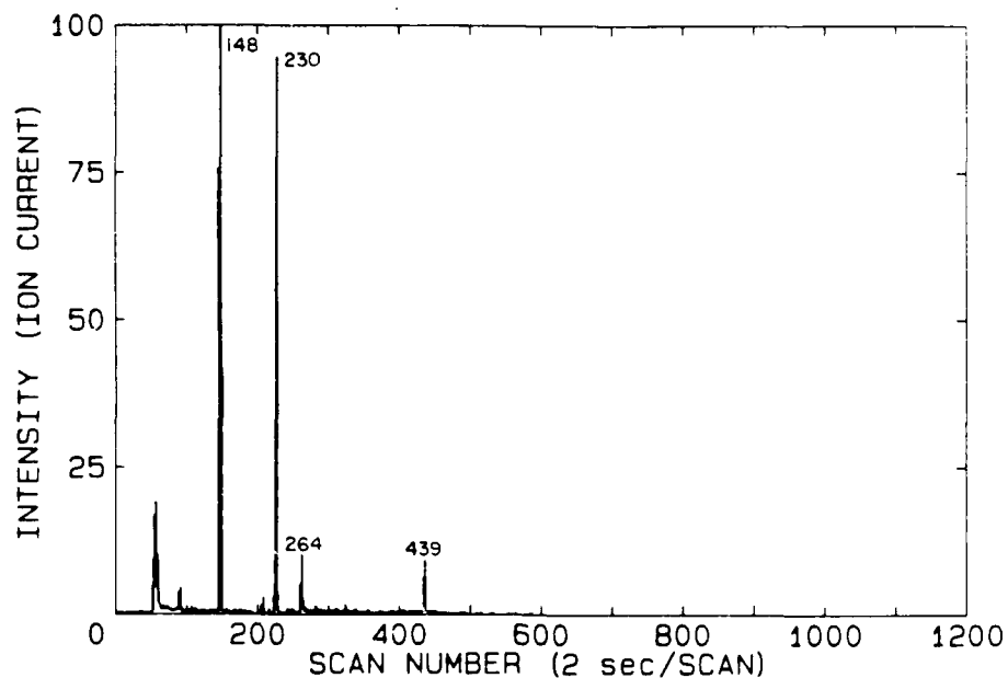
FIGURE 14: RIC showing the compounds released from Hetron 99P resin after heating for 7 minutes at 300°C in an inert atmosphere.
