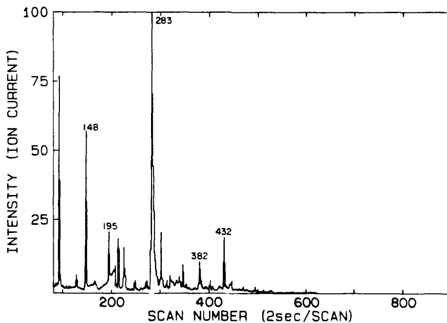
FIGURE 29: RIC showing the compounds released from the vinyl ester portion of Derakane 510A resin after heating at 400°C for 10 minutes in an inert atmosphere.
