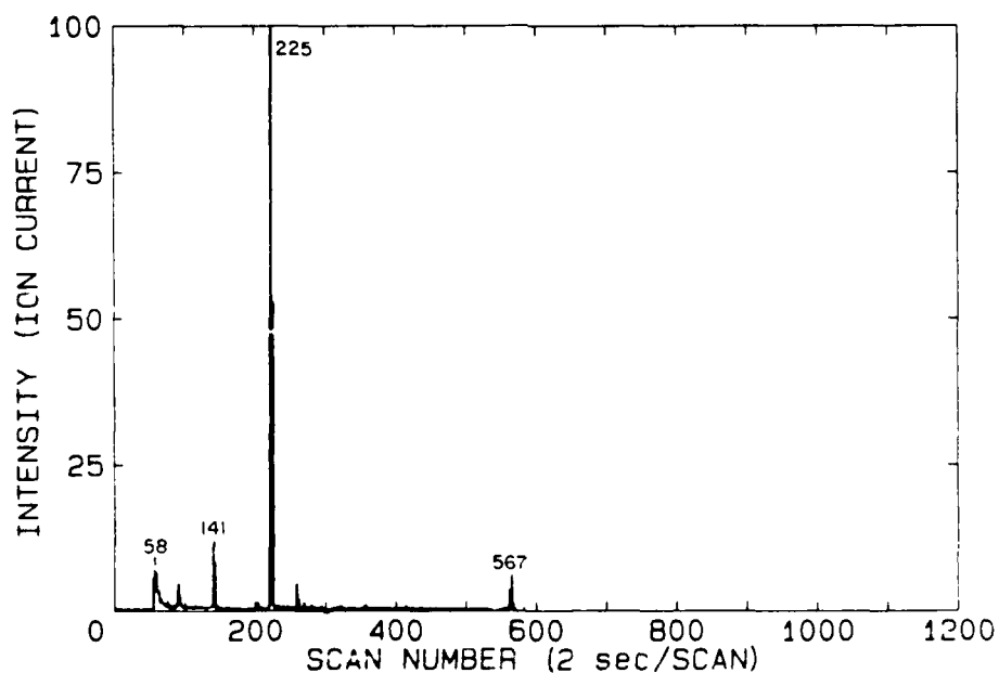
FIGURE 11: RIC showing the compounds released from Hetron 197AT resin after heating for 7 minutes at 300°C in an inert atmosphere.
