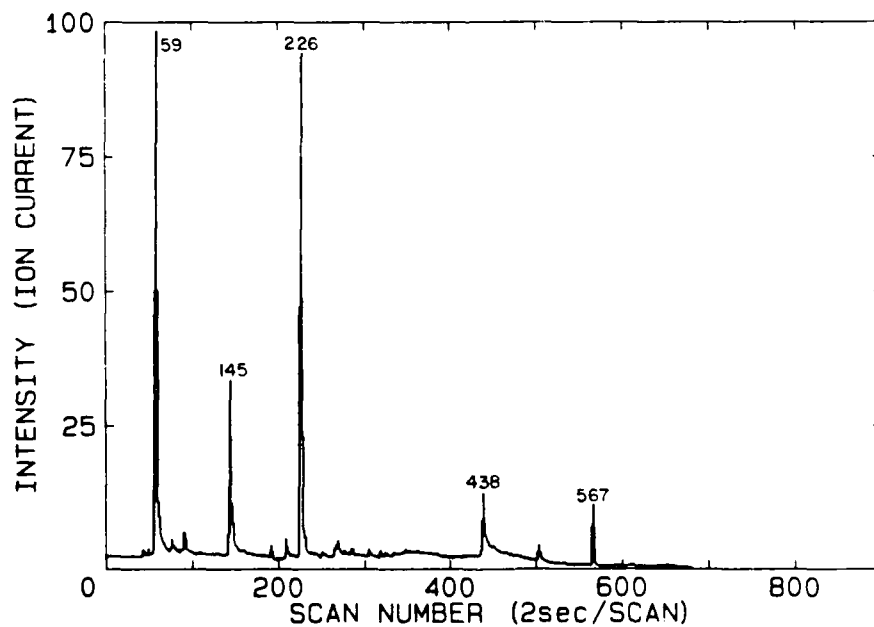
FIGURE 7: RIC showing the compounds released from Vibrin F1029 resin after heating for 7 minutes at 200 C in an inert atmosphere.
