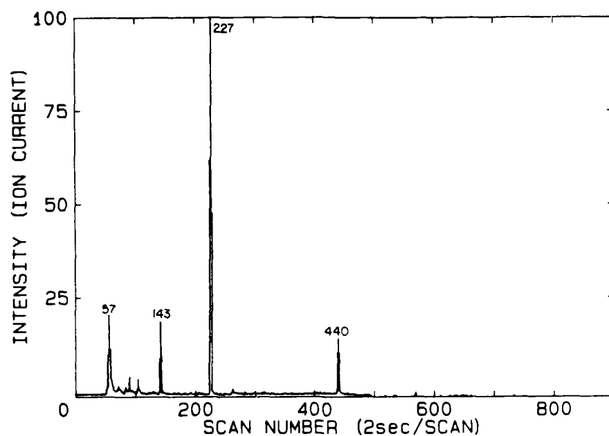
FIGURE 8: RIC showing the compounds released from Vibrin F1029 resin after heating for 7 minutes at 300 C in an inert atmosphere.
