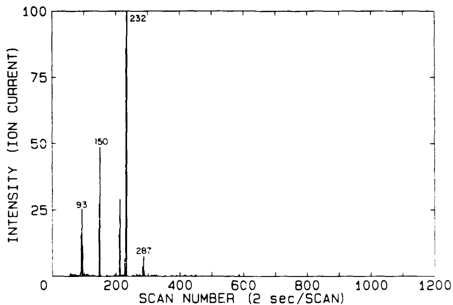
FIGURE 12: RIC showing the compounds released from Hetron 197AT resin after heating for 7 minutes at 400°C in an inert atmosphere.
