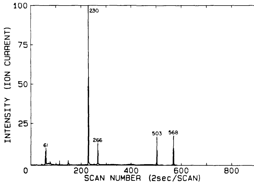
FIGURE 25: RIC showing the compounds released from Hetron 99P resin after heating for 7 minutes at 200°C in a reactive atmosphere.
