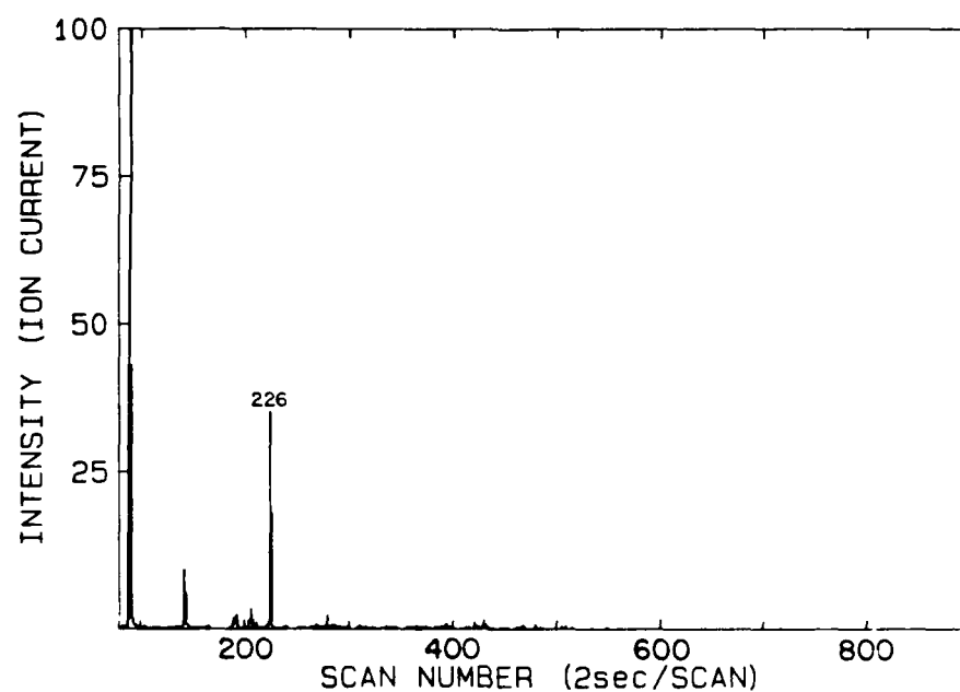
FIGURE 32: RIC showing the compounds released from the polyester portion of Hetron 99P resin after heating at 400°C for 10 minutes in an inert atmosphere.
