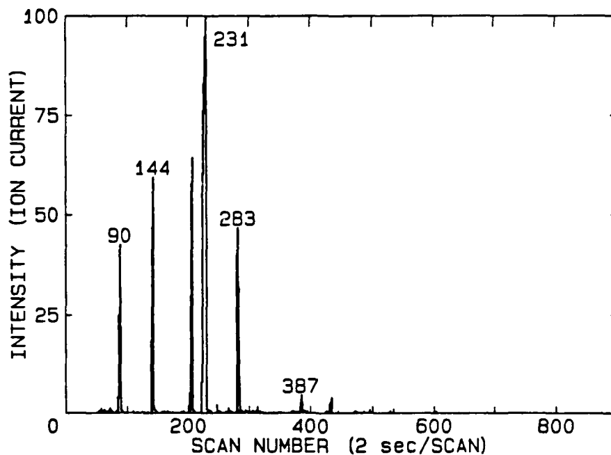
FIGURE 28: RIC showing the compounds released from a sample of polystyrene heated at 400°C for 10 minutes in an inert atmosphere.
