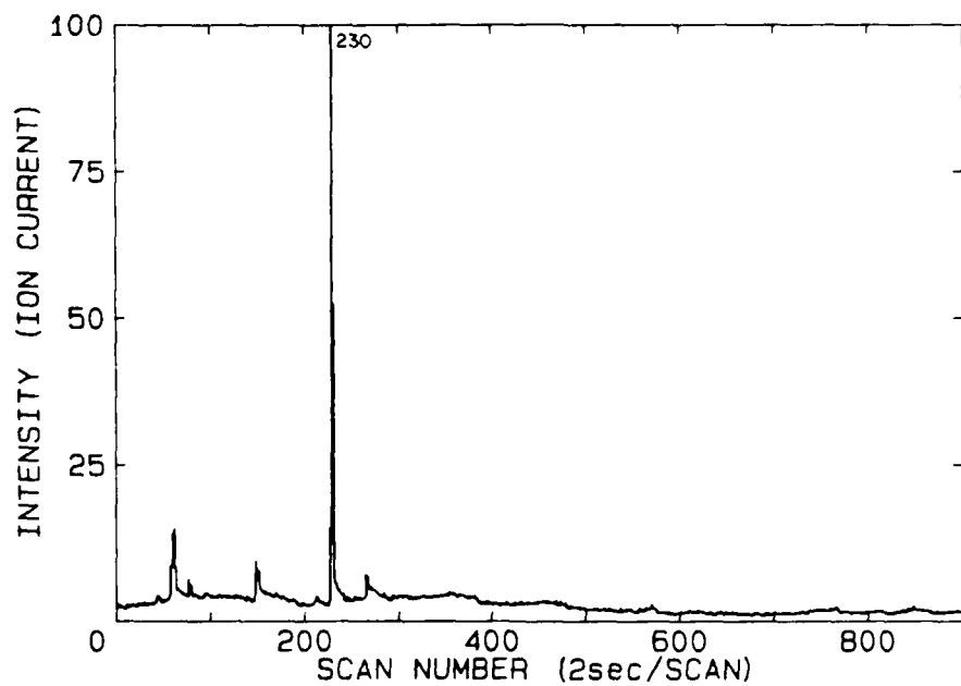
FIGURE 16: RIC showing the compounds released from Derakane 510A resin after heating for 7 minutes at 200°C in a reactive atmosphere.
