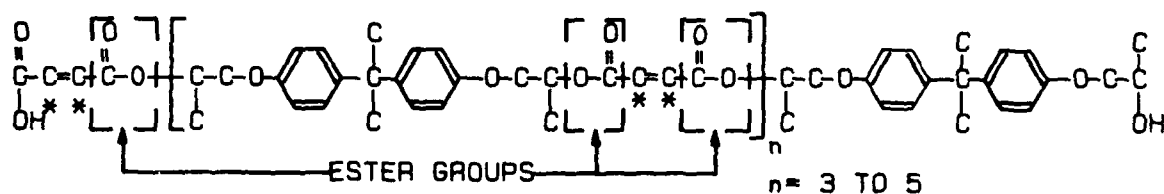
FIGURE 2: Structure of a typical bisphenol A fumaric acid polyester.
