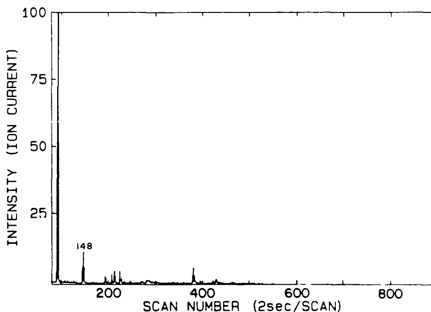
FIGURE 31: RIC showing the compounds released from the polyester portion of Hetron 197AT resin after heating at 400°C for 10 minutes in an inert atmosphere.
