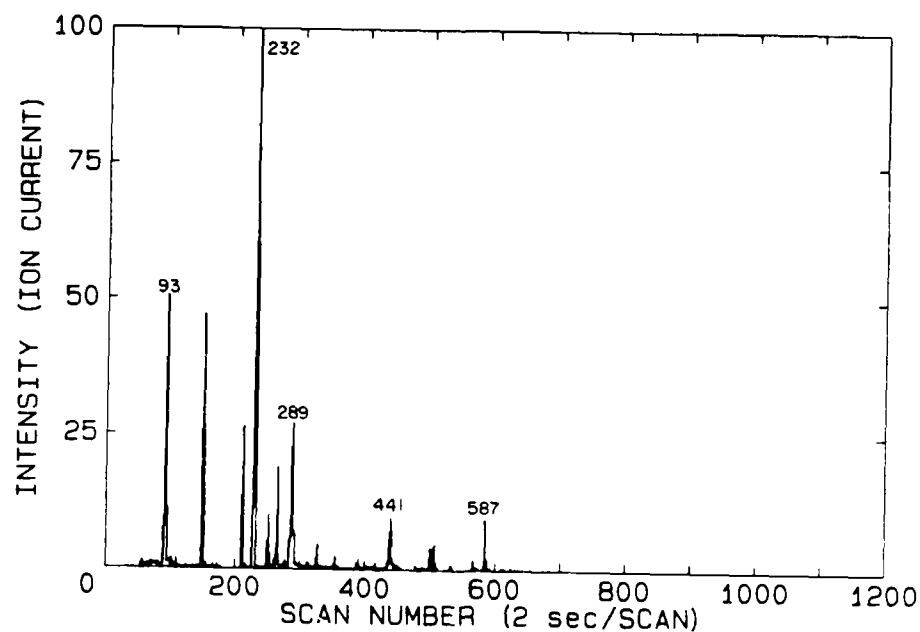
FIGURE 18: RIC showing the compounds released from Derakane 510A resin after heating for 7 minutes at 400°C in a reactive atmosphere.
