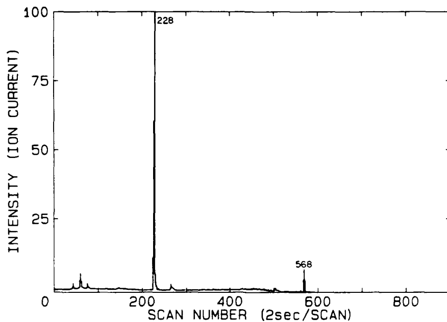
FIGURE 22: RIC showing the compounds released from Hetron 197AT resin after heating for 7 minutes at 200°C in a reactive atmosphere.
