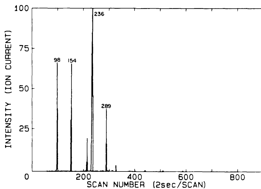
FIGURE 9: RIC showing the compounds released from Vibrin F1029 resin after heating for 7 minutes at 400°C in an inert atmosphere.
