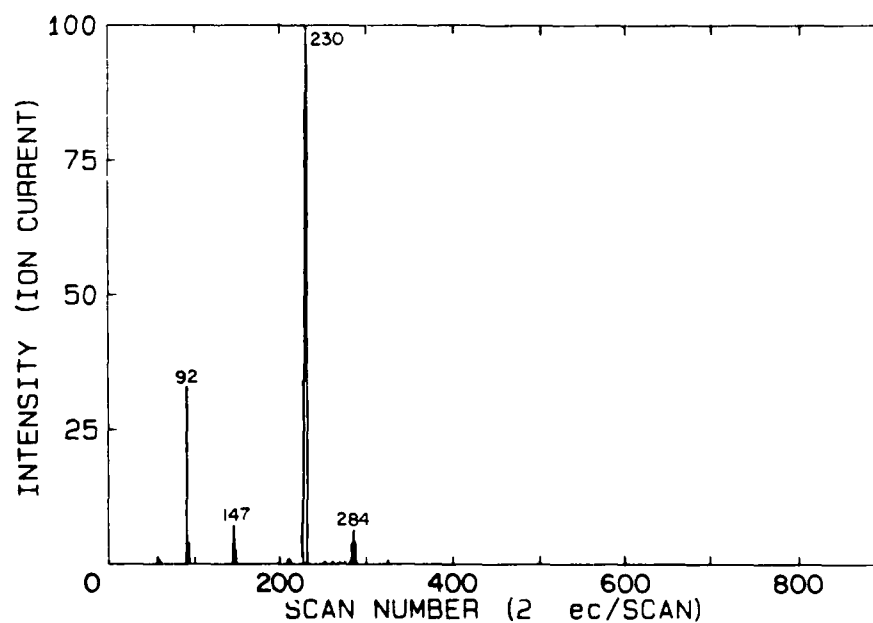
FIGURE 5: RIC showing the compounds released from Derakane 510A resin after heating for 7 minutes at 300 C in an inert atmosphere.
