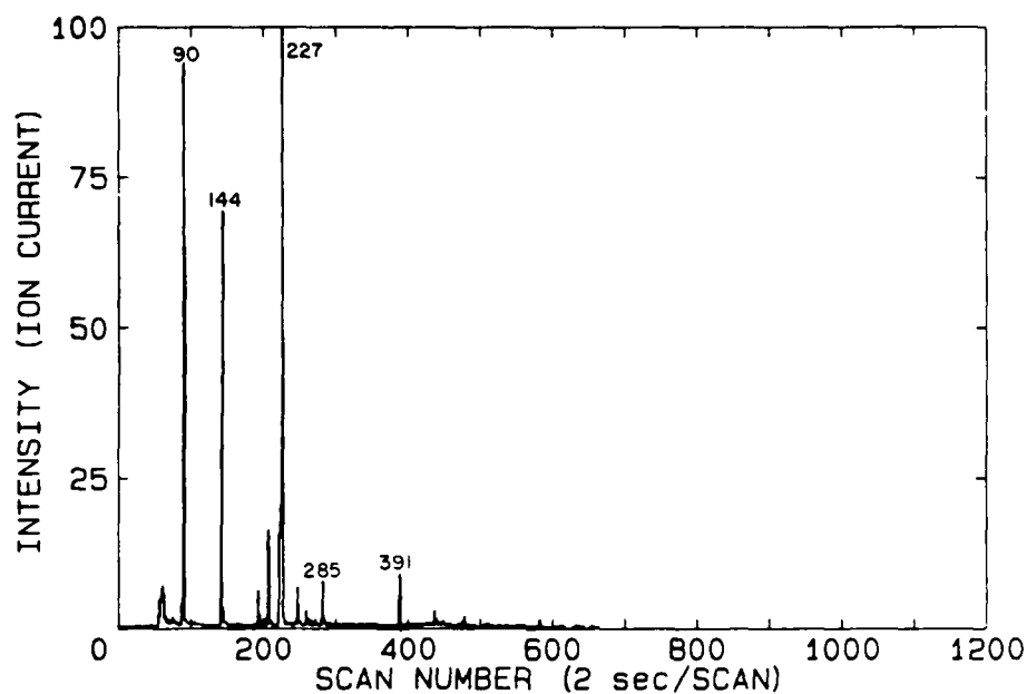
FIGURE 24: RIC showing the compounds released from Hetron 197AT resin after heating for 7 minutes at 400°C in a reactive atmosphere.
