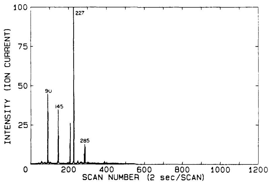
FIGURE 27: RIC showing the compounds released from Hetron 99P resin after heating for 7 minutes at 400°C in a reactive atmosphere.
