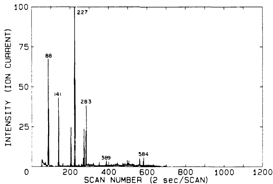
FIGURE 15: RIC showing the compounds released from Hetron 99P resin after heating for 7 minutes at 400°C in an inert atmosphere.
