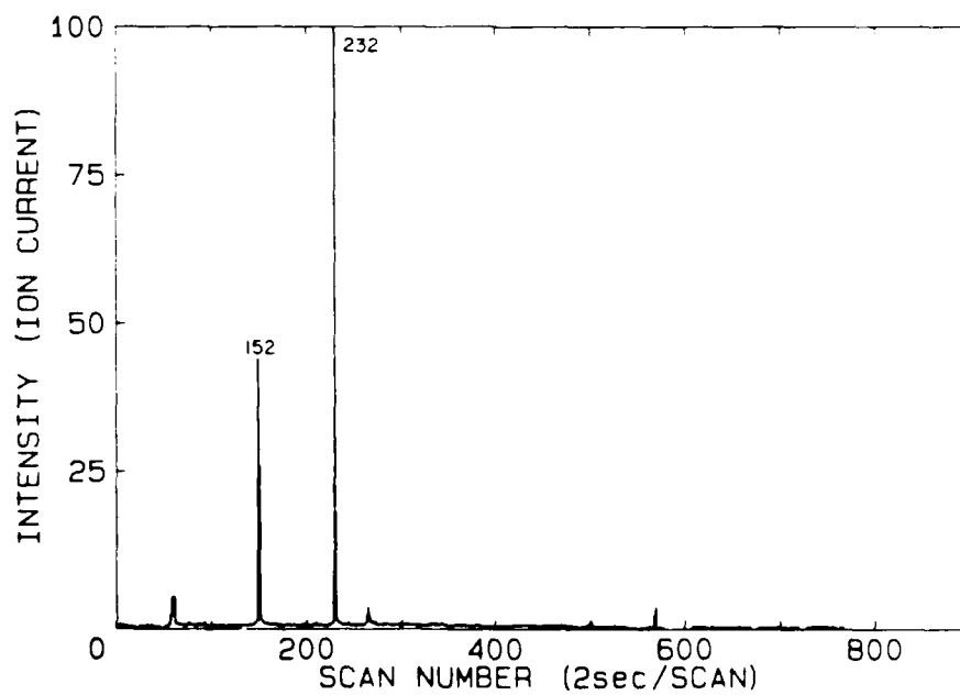
FIGURE 13: RIC showing the compounds released from Hetron 99P resin after heating for 7 minutes at 200°C in an inert atmosphere.
