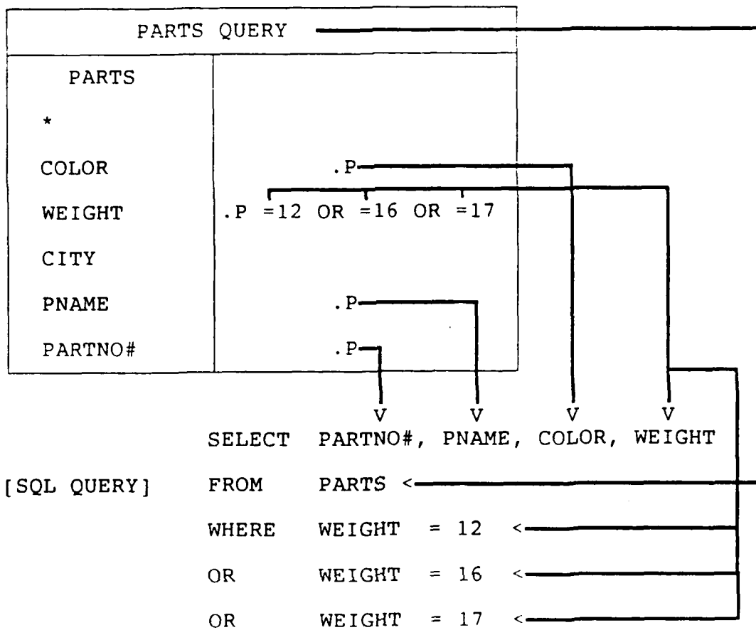
Figure 14. Retrieval Using a Set of Weight Values
