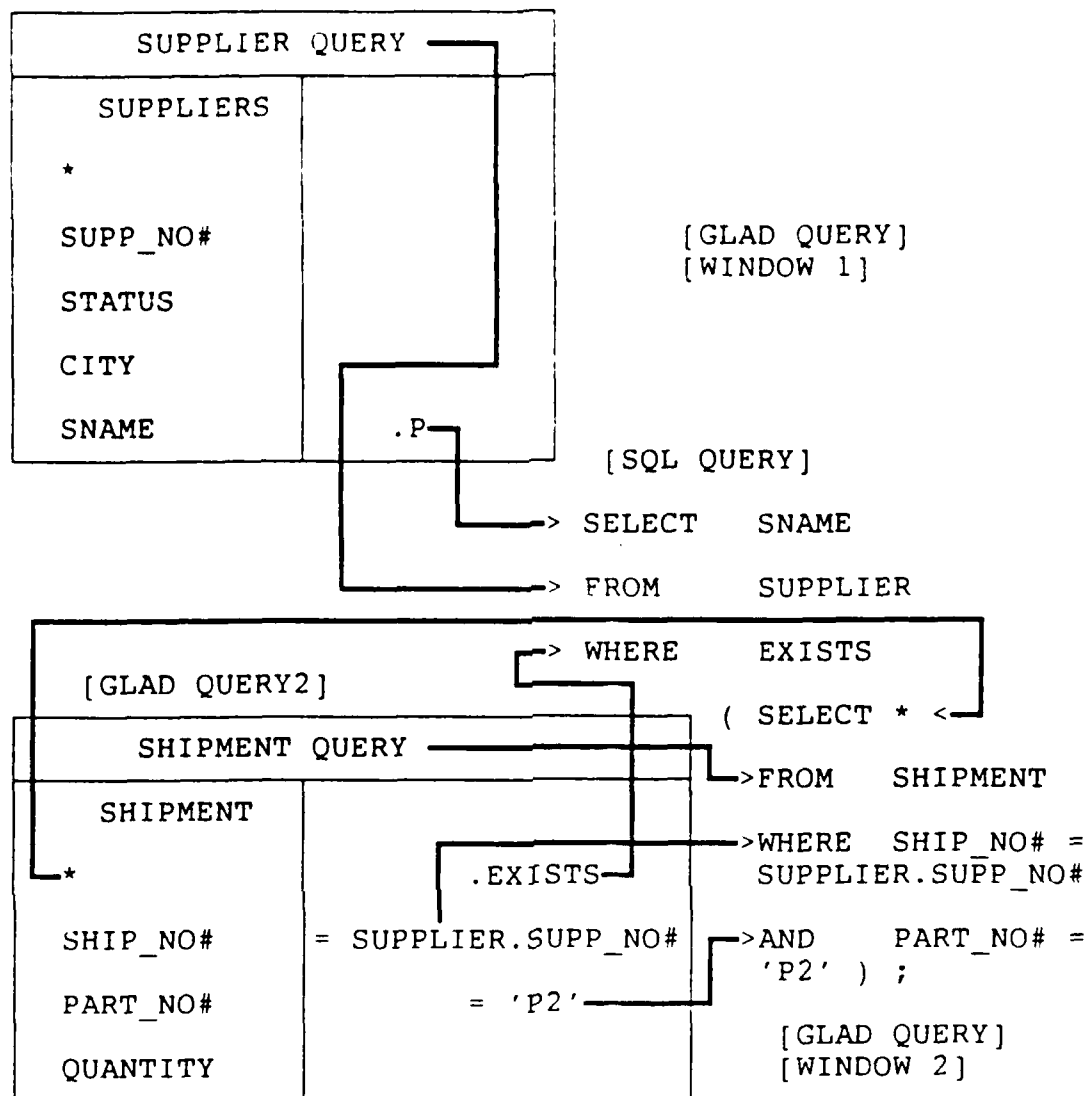
Figure 21. Query Illustrating Nested Selects
