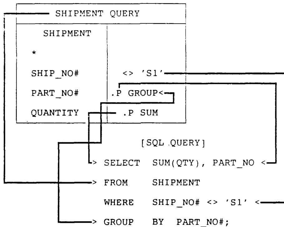
Figure 25. GLAD Query Using GROUP BY
