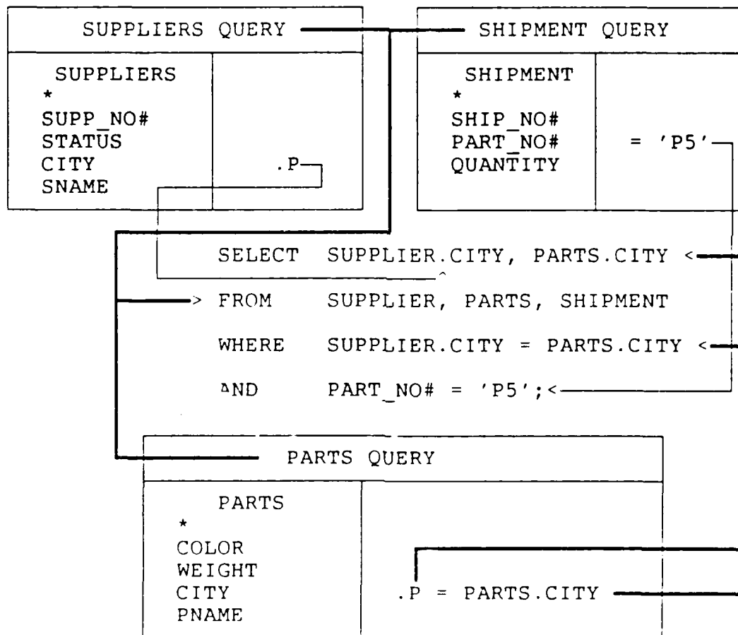
Figure 20. Three Object GLAD Query
