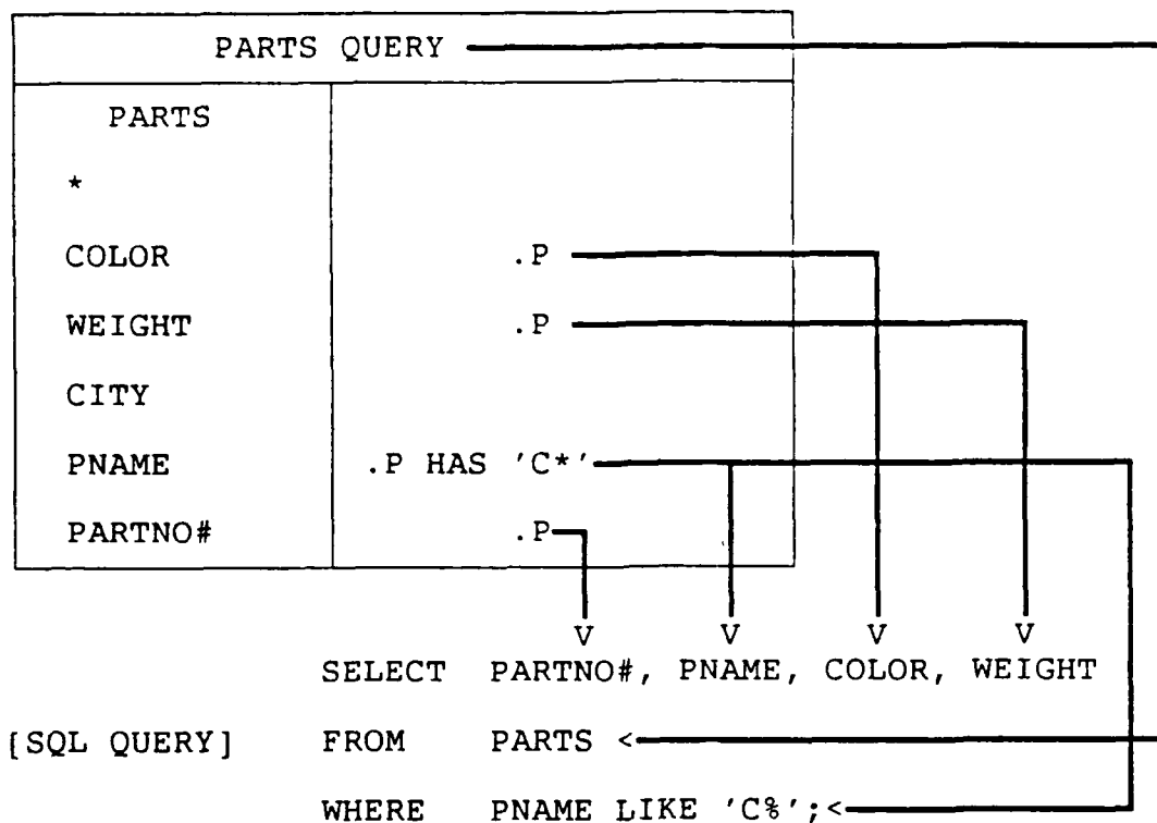
Figure 16. Retrieval Using a Search String
