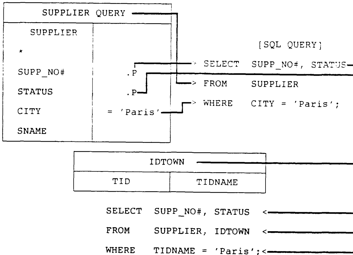
Figure 27. Non-Atomic Sub-Object with a Condition
