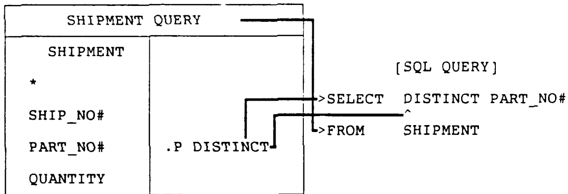
Figure 5. Simple Query with Distinct Ordering
