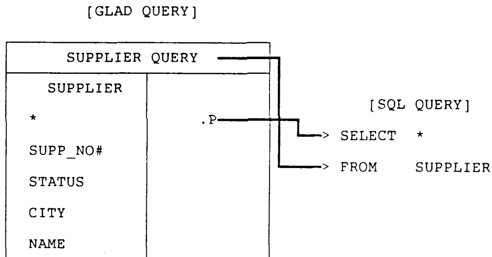
Figure 9. Copy the Entire Table
