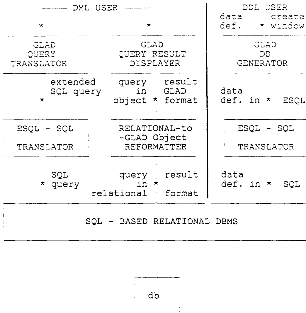
Figure 35. Translation Scheme
