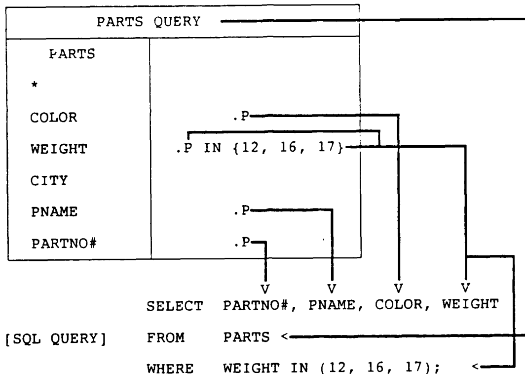
Figure 13. Retrieval Using a Set of Weight Values
