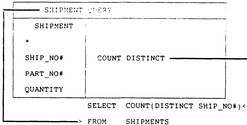
Figure 22. GLAD Query with Distinct Count
