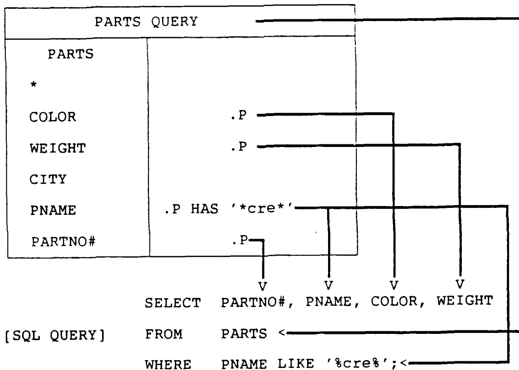
Figure 17. Retrieval with Embedded Sting
