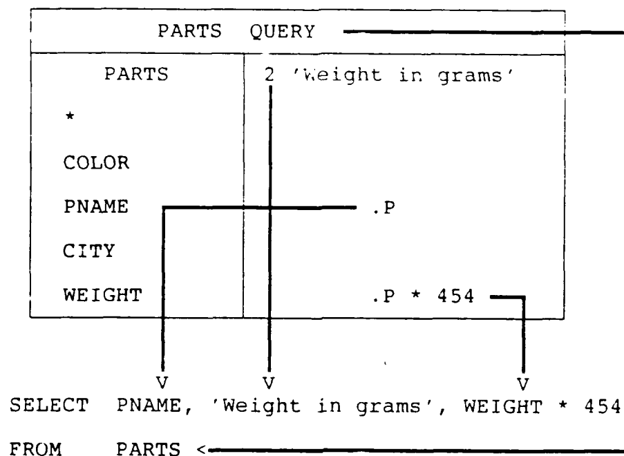
Figure 7. Query with a Message
