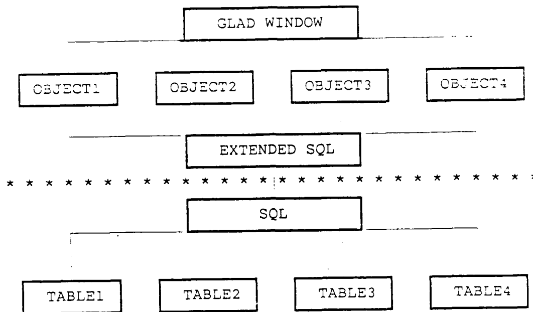
Figure 34. GLAD and SQL System Modules
