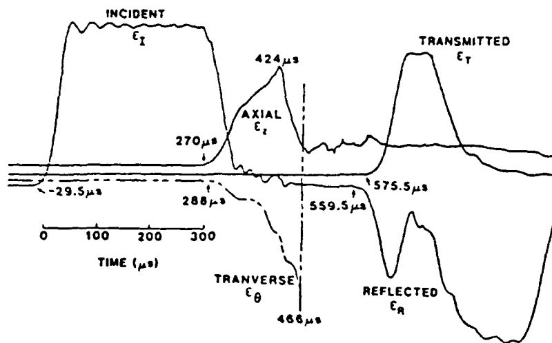
Figure 2. Strain Pulses in Pressure Bars and Axial and Transverse Specimen Surface Strains
