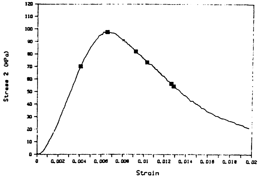
Figure 17. Dynamic stress-strain curve for no-collar test of Specimen F05 with six points marked corresponding to maximum strains in collar-interrupted tests.
