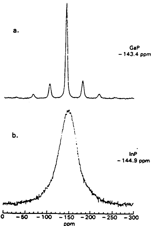
Fig. 3. 31 P MAS NMR spectra of zinc blende-type GaP and InP.
